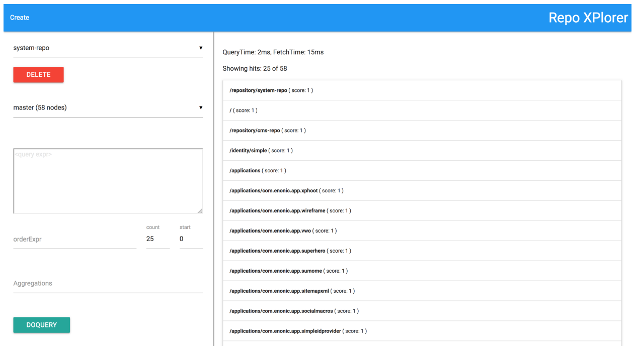
Fig. 7.1: Screenshot from the Repo XPlorer app which will be available on Enonic Market soon
