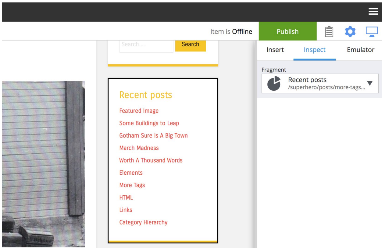
Fig. 7.2: Fragments can be inserted on multiple pages
