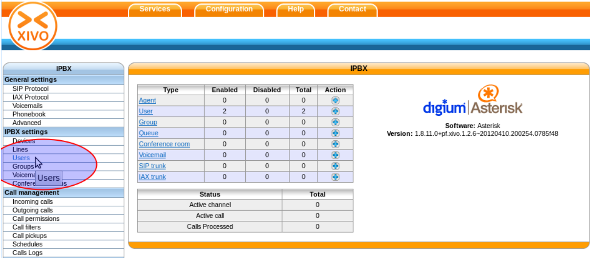
Fig. 1.8: Users settings
