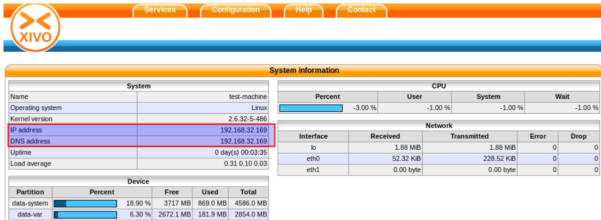
Fig. 1.6: System informations
