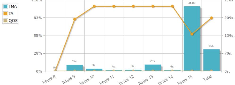
Queues Performance
