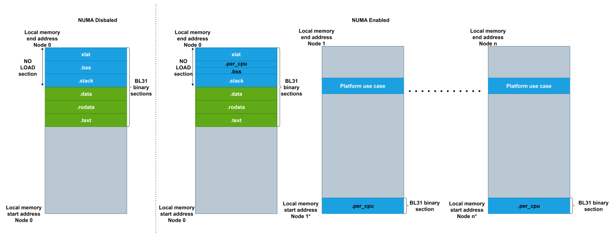
Figure: BL31/BL32 binary storage in local memory of per node when per-cpu NUMA framework is enabled
