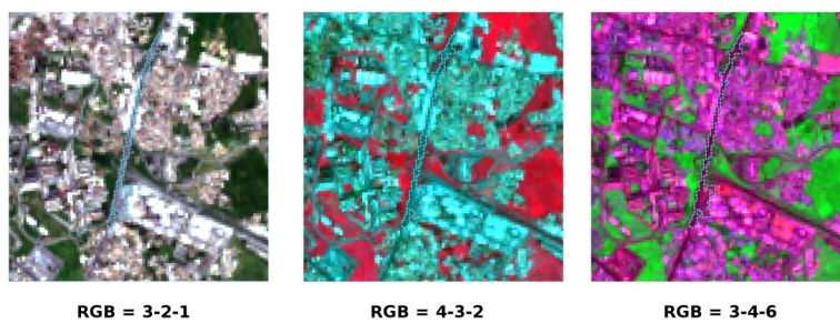
Rys. 19.10: Built-up ROI: road
