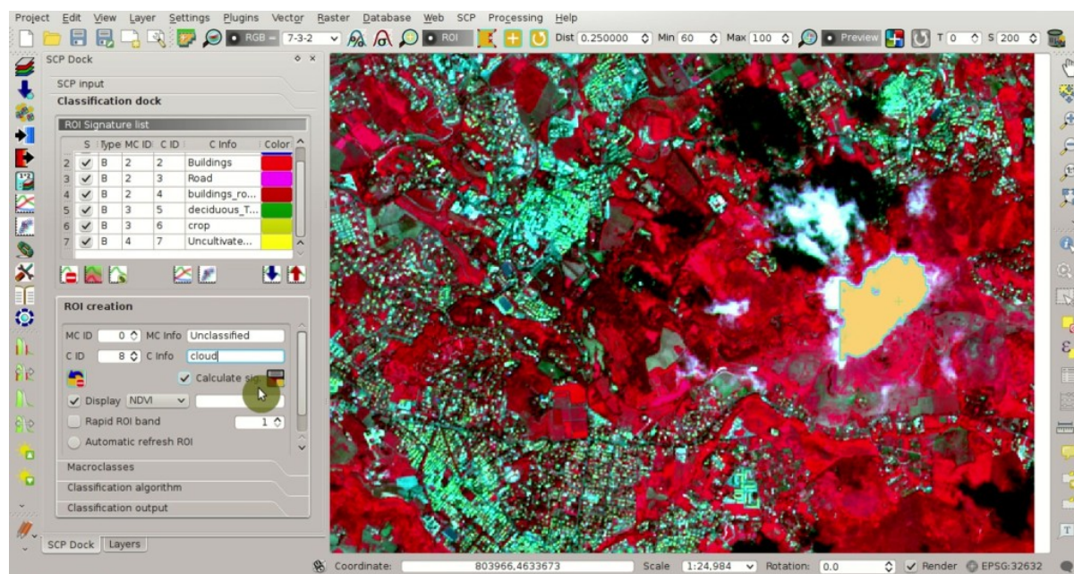
Rys. 20.23: Example of ROI for clouds
