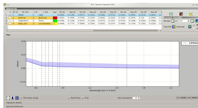
Rys. 22.8: Signature plot: the spectral range is extended
