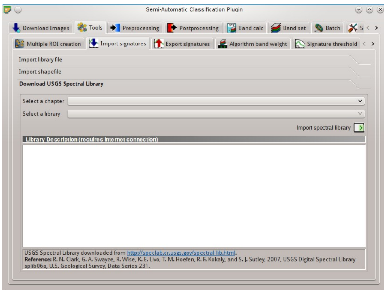
Rys. 10.10: Download USGS Spectral Library
