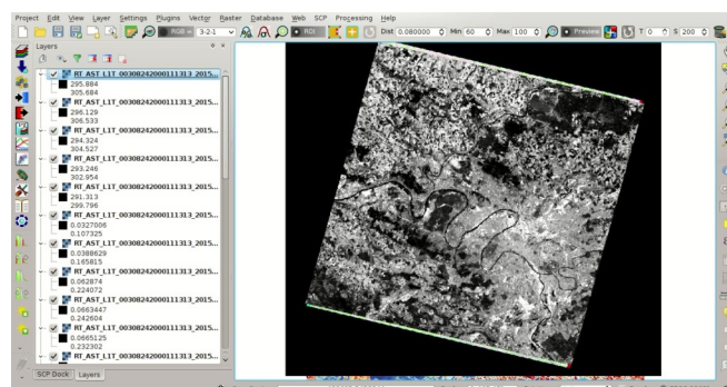
Rys. 23.19: Converted ASTER bands
