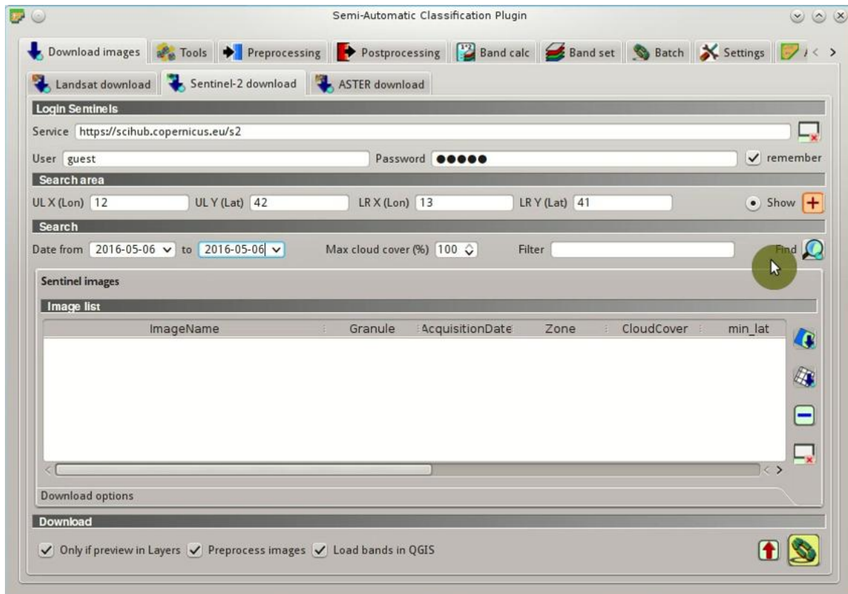
Rys. 20.1: Search Sentinel-2 images
