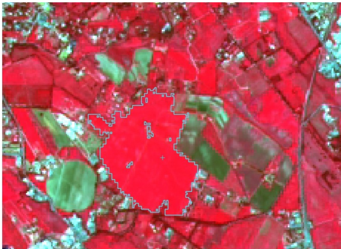
Rys. 19.7: Vegetation
