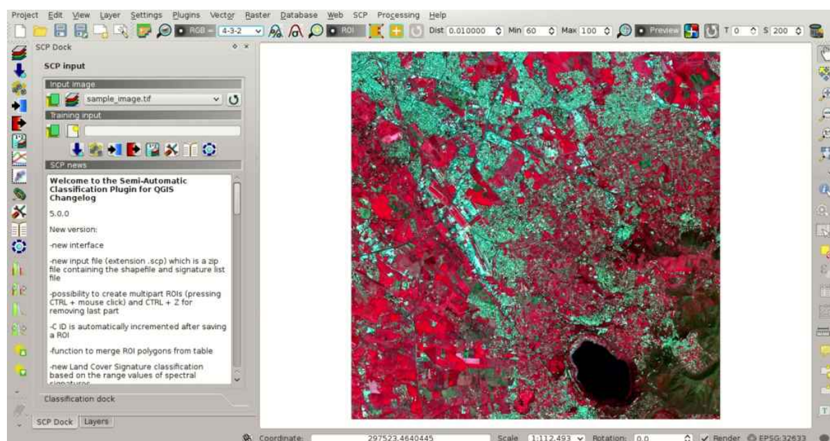
Rys. 19.1: Color composite RGB=4-3-2
