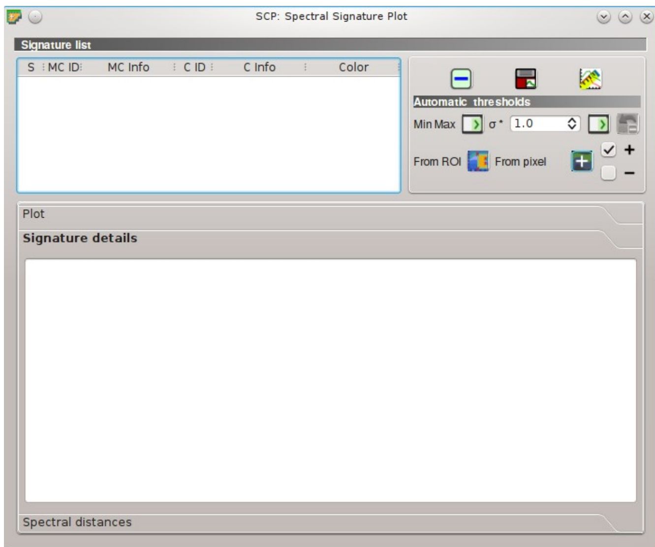
Rys. 11.3: Spectral Signature: Signature details
