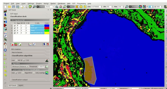
Rys. 22.7: Signature plot: the spectral range is extended
