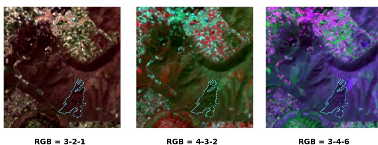
Rys. 19.13: Vegetation ROI: deciduous trees
