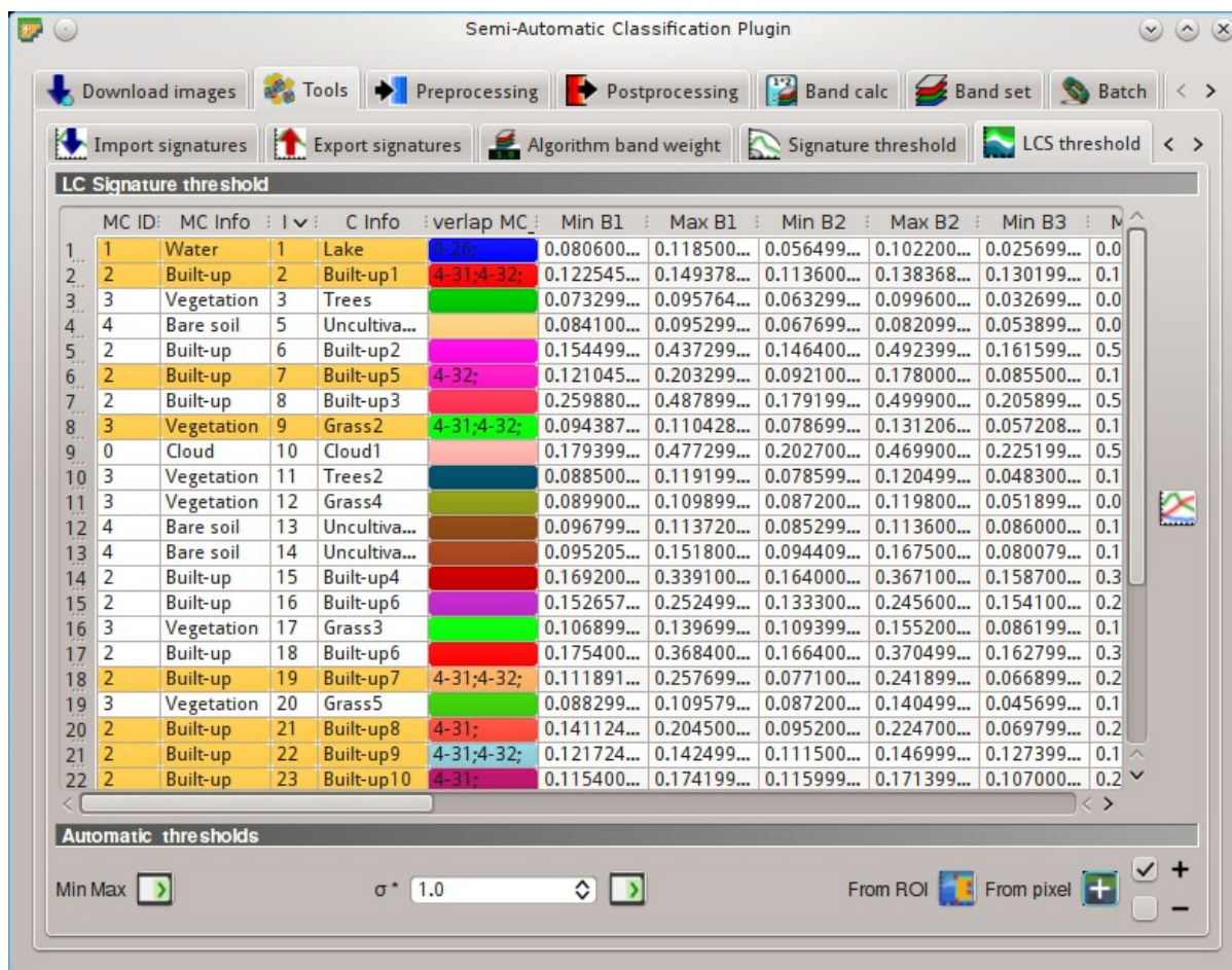
Rys. 22.13: LCS threshold. Overlapping regions are highlighted in orange
