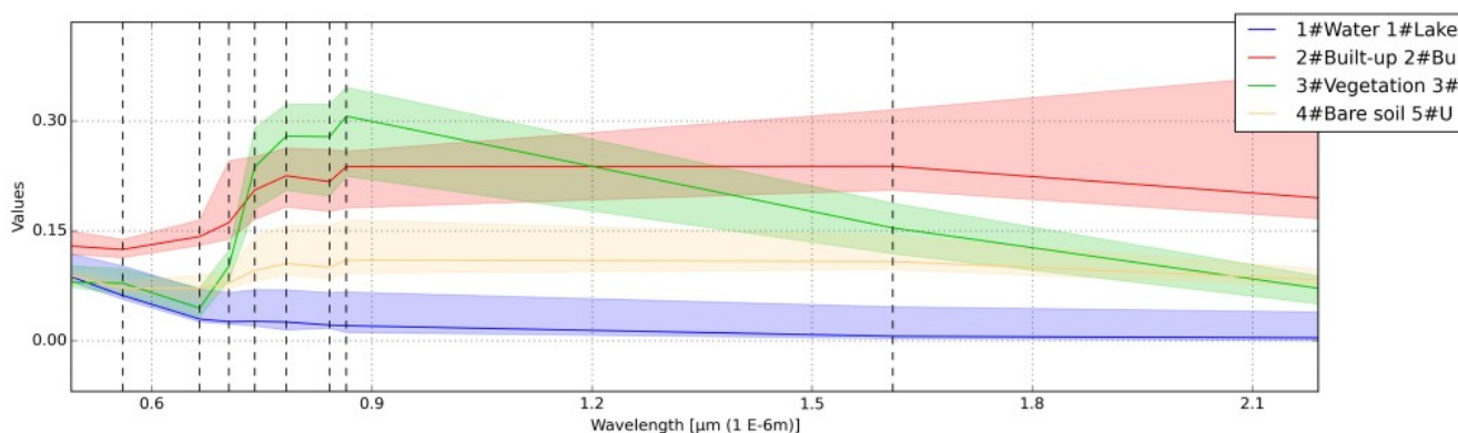
Rys. 11.2: Spectral Signature: Example of spectral signature plot
