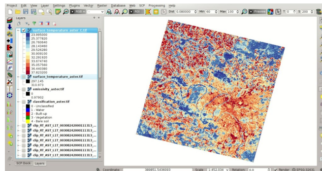
Rys. 23.28: Land Surface Temperature of the ASTER Image
