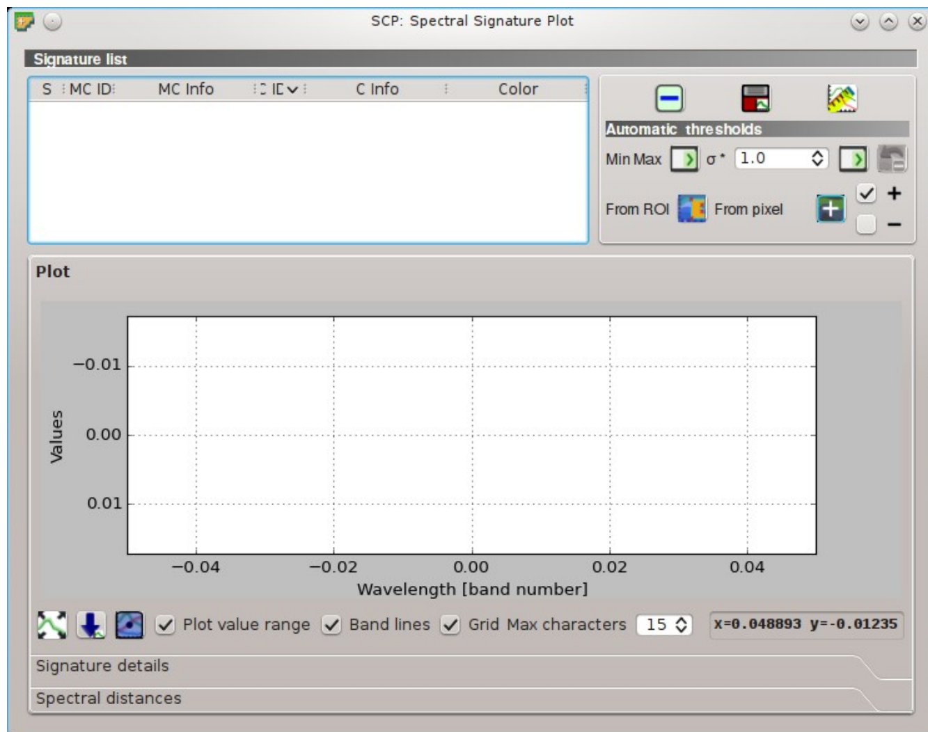
Rys. 11.1: Spectral Signature Plot
