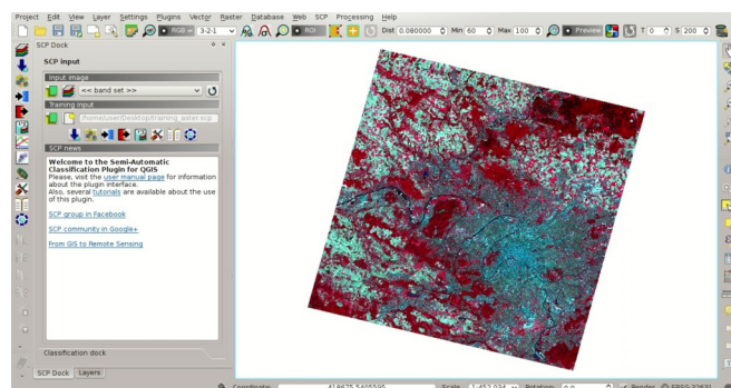
Rys. 23.23: ASTER color composite
