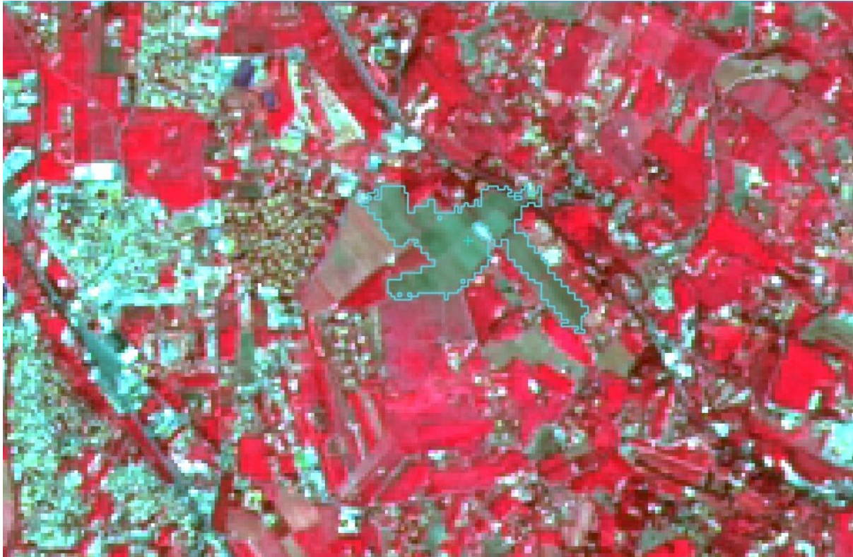
Rys. 19.8: Bare soil
