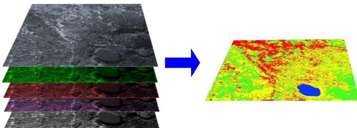
Rys. 30.1: A multispectral image processed to produce a land cover classification (Landsat image provided by USGS)
