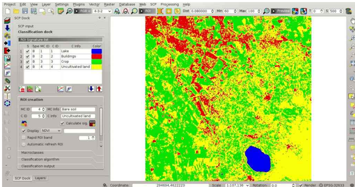
Rys. 19.17: Result of the land cover classification
