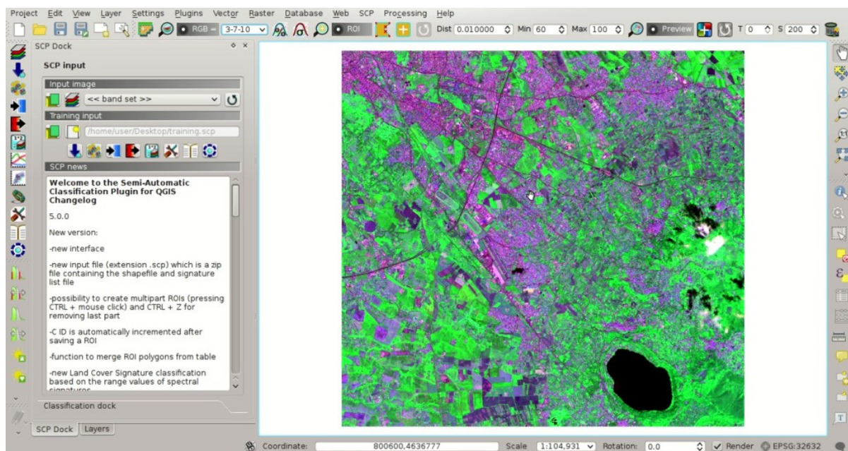
Rys. 20.14: Color composite RGB = 3-7-10
