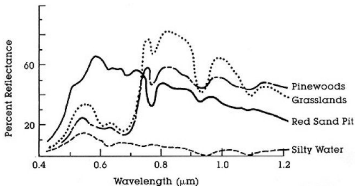
Rys. 14.2: Spectral Reflectance Curves of Four Different Targets (from NASA, 2013)
