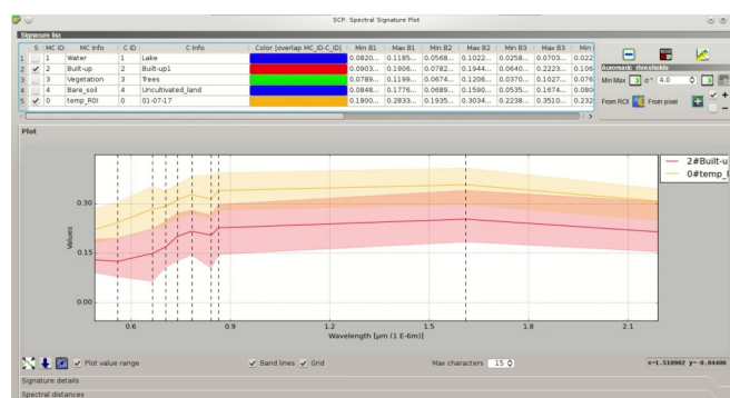
Rys. 22.11: The plot of a temporary ROI
