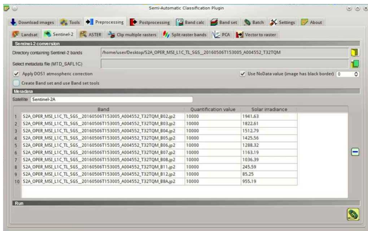
Rys. 20.6: Sentinel-2 conversion to reflectance
