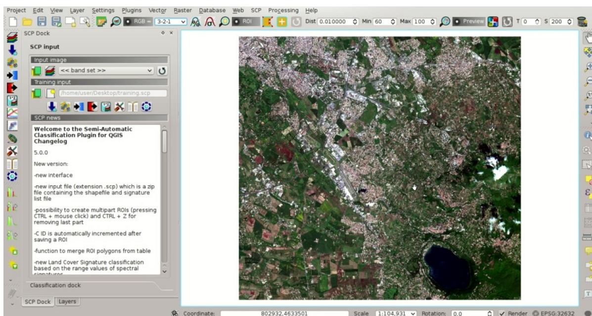
Rys. 20.13: Color composite RGB = 3-2-1
