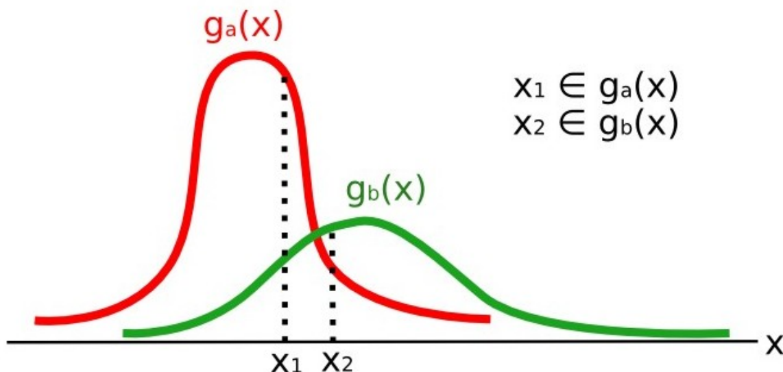
Rys. 15.4: Maximum Likelihood example
