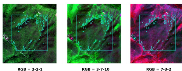
Rys. 20.20: Vegetation ROI: deciduous trees
