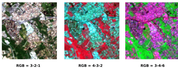
Rys. 19.9: Built-up ROI: large buildings
