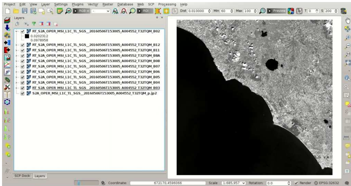
Rys. 20.7: Converted Sentinel-2 bands
