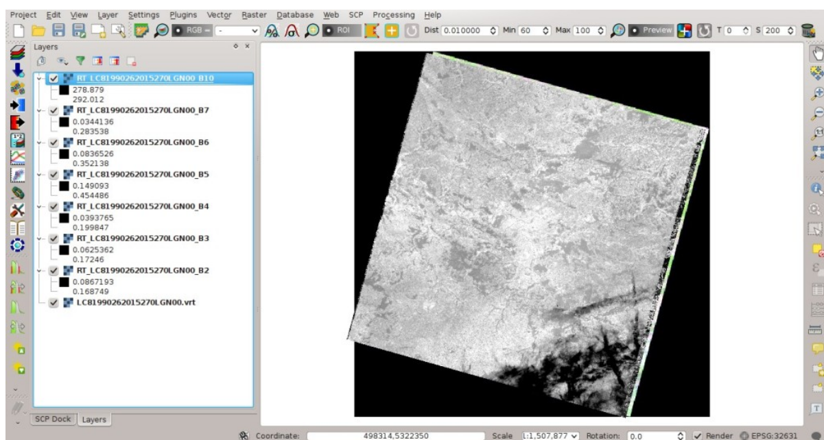
Rys. 23.5: Converted Landsat bands
