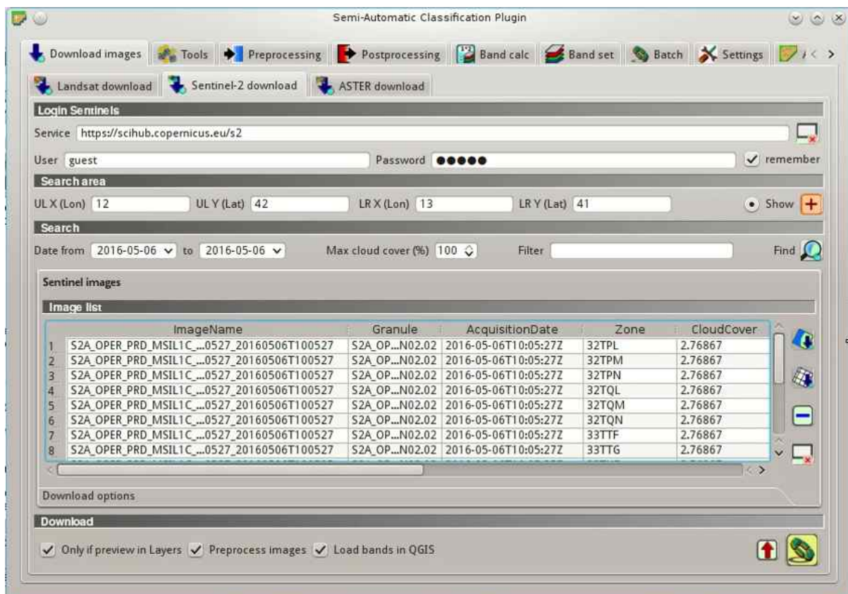
Rys. 20.2: Sentinel-2 search result
