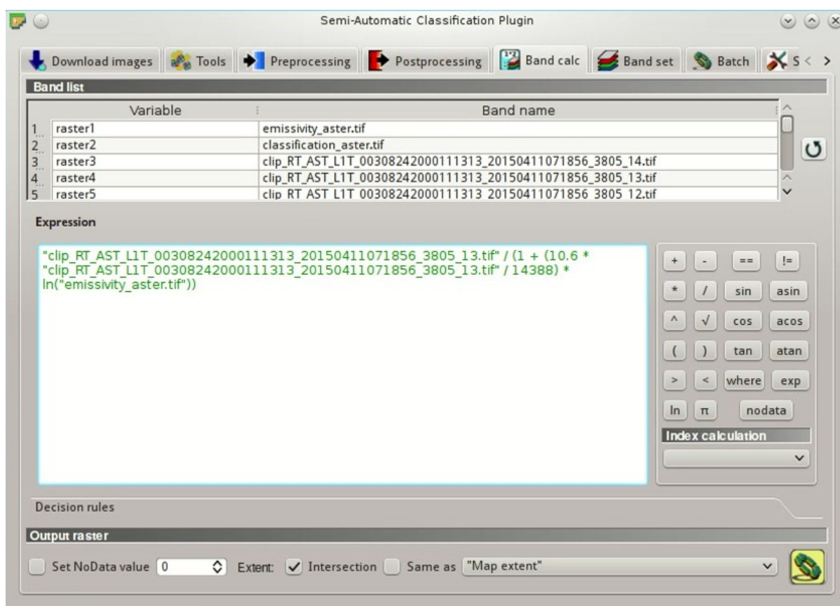
Rys. 23.27: Calculation of surface temperature
