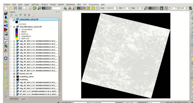
Rys. 23.26: ASTER emissivity raster
