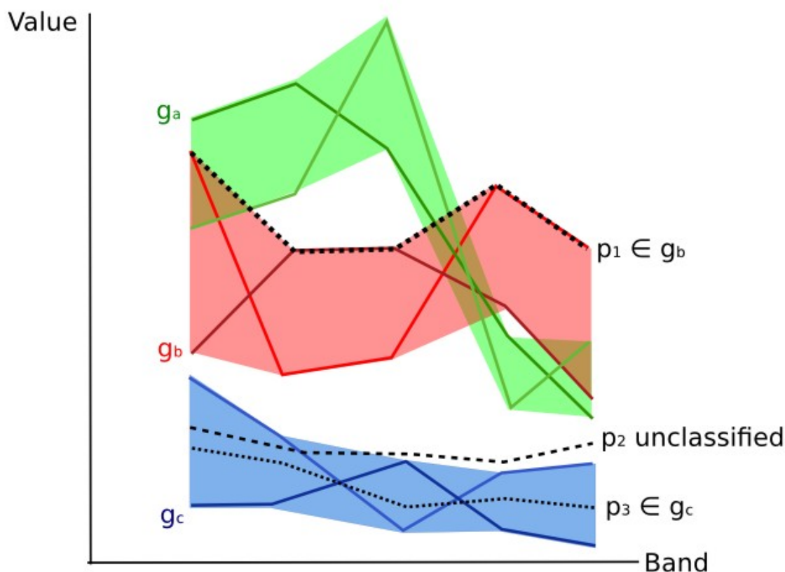
Rys. 15.7: Plot of spectral ranges
