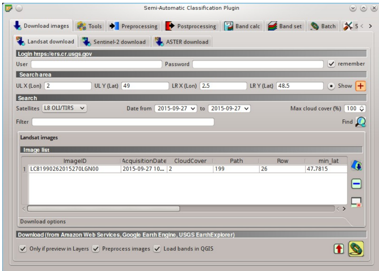
Rys. 23.1: Landsat search result
