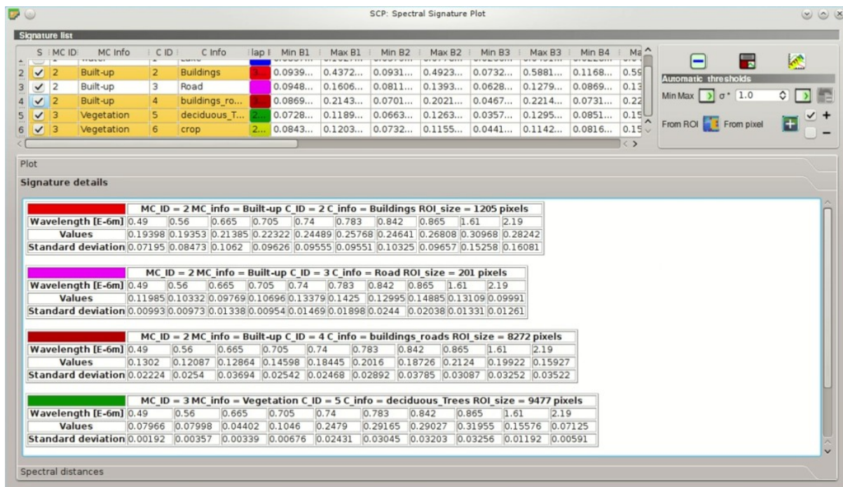
Rys. 20.28: Spectral signature values
