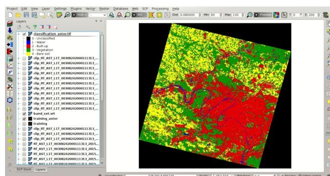
Rys. 23.24: ASTER land cover classification
