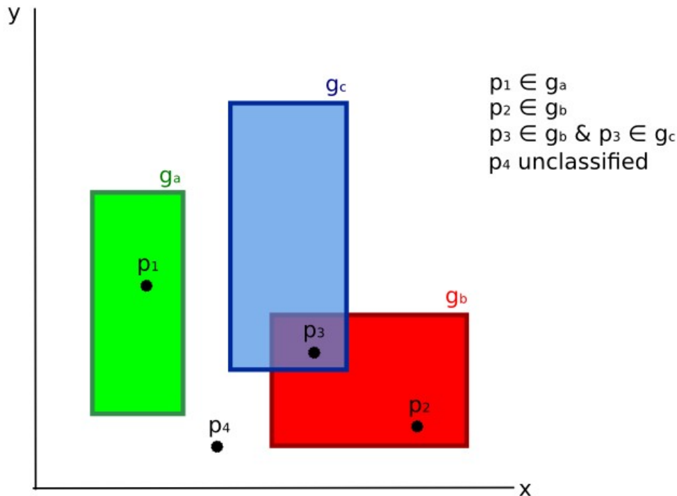
Rys. 15.6: Land cover signature classification
