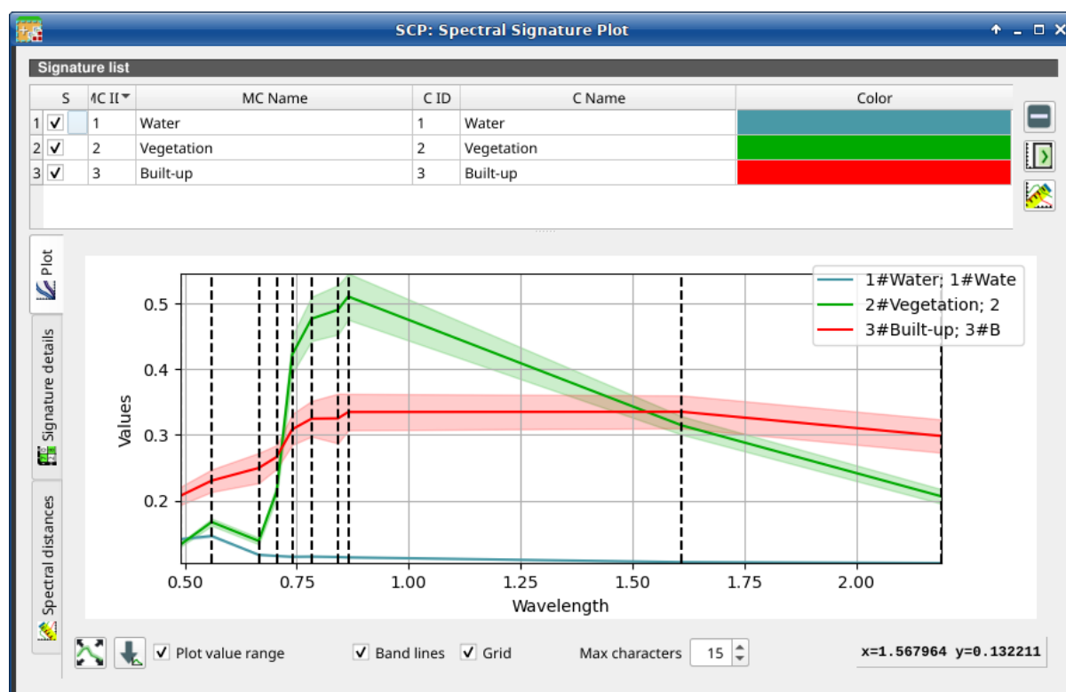
Рис. 51: Spectral Signature: Example of plot
