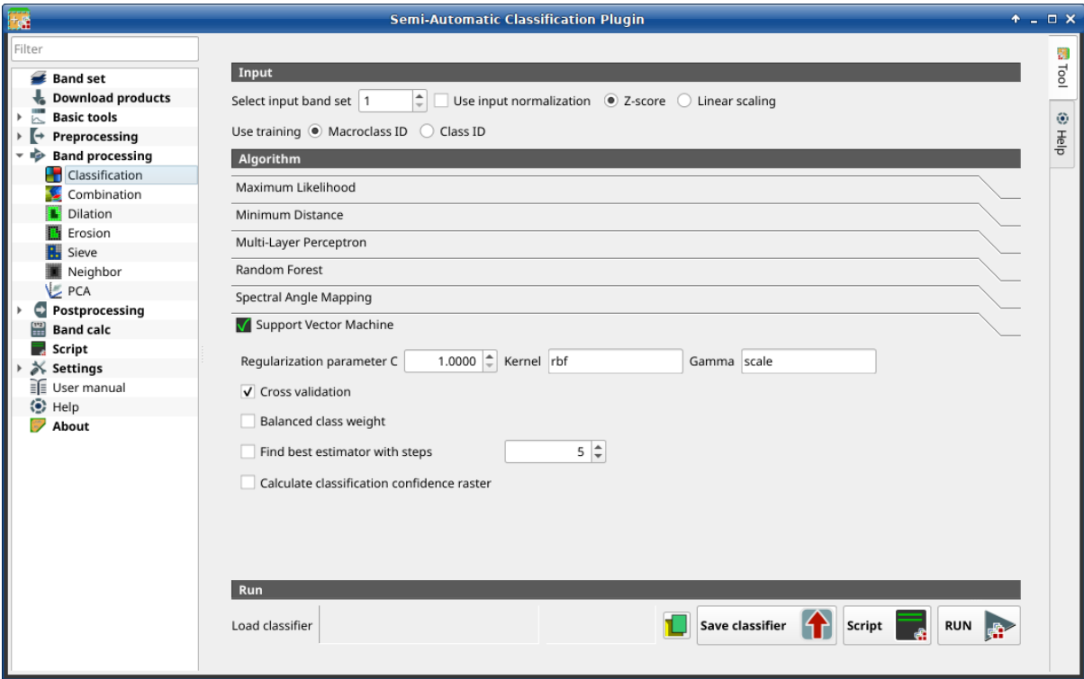
Рис. 33: Support Vector Machine
