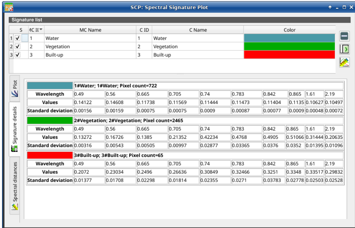
Рис. 52: Spectral Signature: Example of signature details
