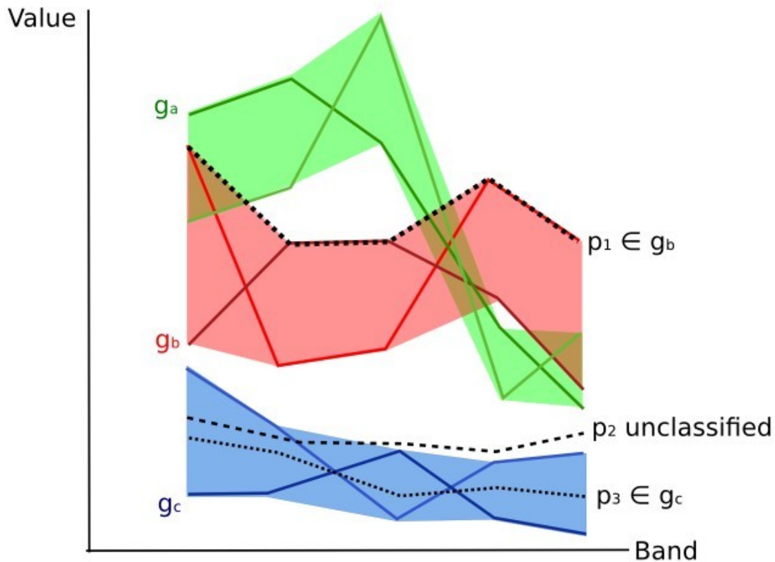
Рис. 10: Plot of spectral ranges
