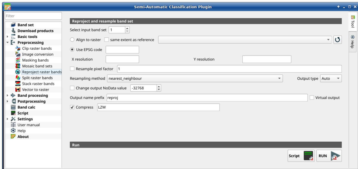
Рис. 23: Reproject raster bands
