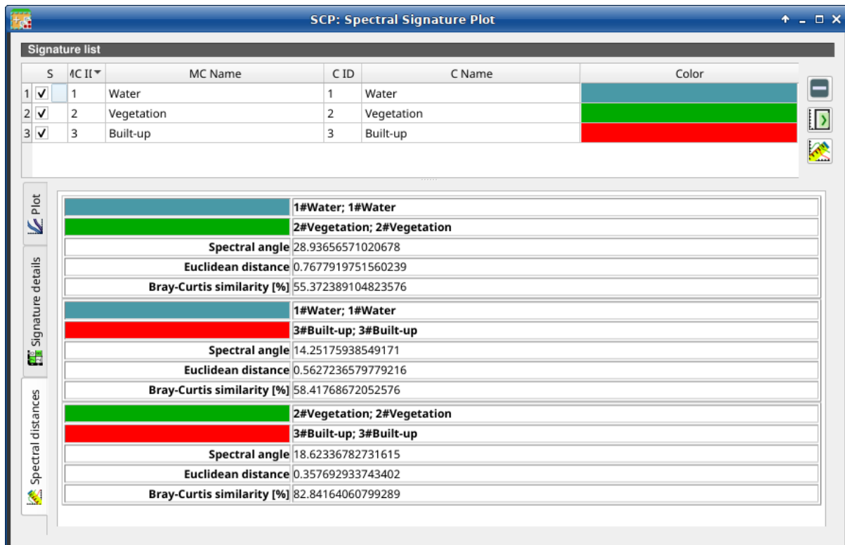
Рис. 53: Spectral Signature: Example of spectral distances
