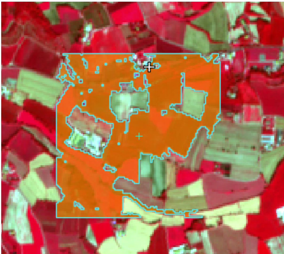
Рис. 8: Vegetation. Color composite RGB = 7-3-2
