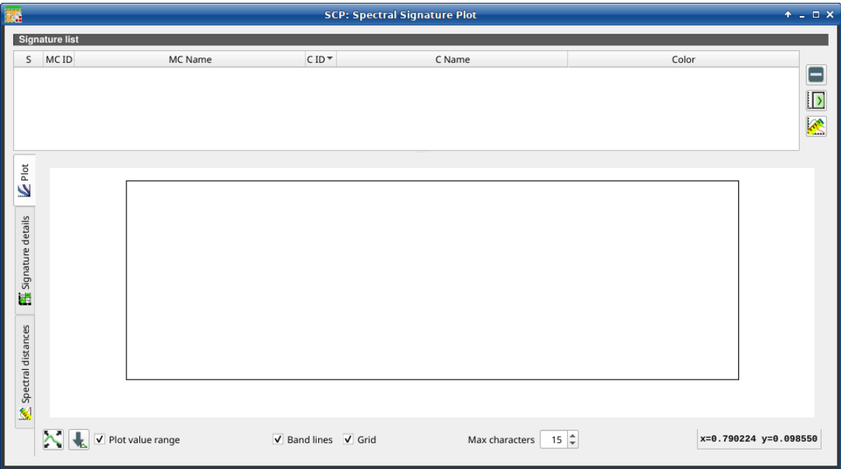
Рис. 50: Spectral Signature Plot
