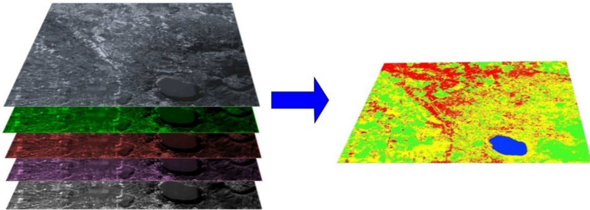
Рис. 3: A multispectral image processed to produce a land cover classification (Landsat image provided by USGS)
