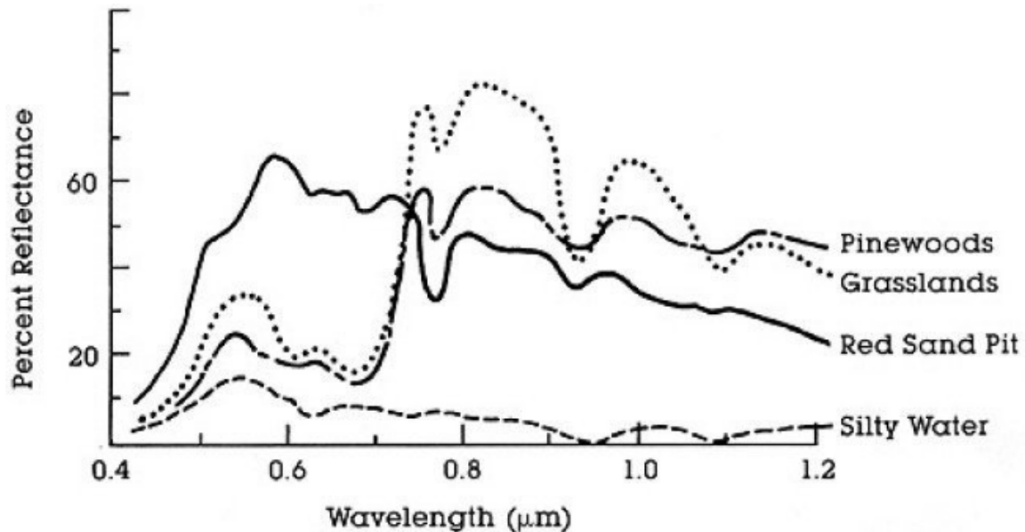
Рис. 2: Spectral Reflectance Curves of Four Different Targets (from NASA, 2013)
