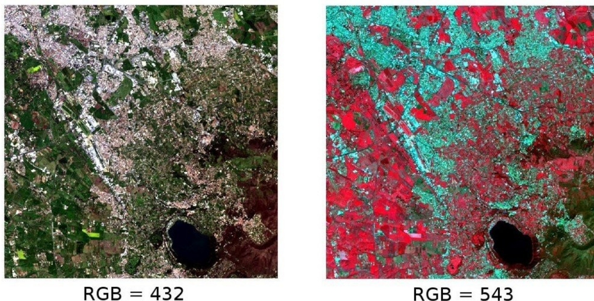
Рис. 4: Color composite of a Landsat 8 image Data available from the U.S. Geological Survey
