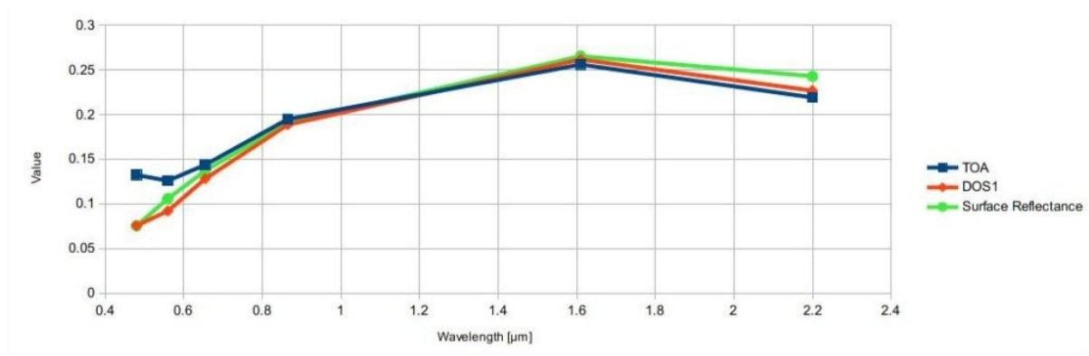
Рис. 13: Spectral signatures of a built-up pixel
