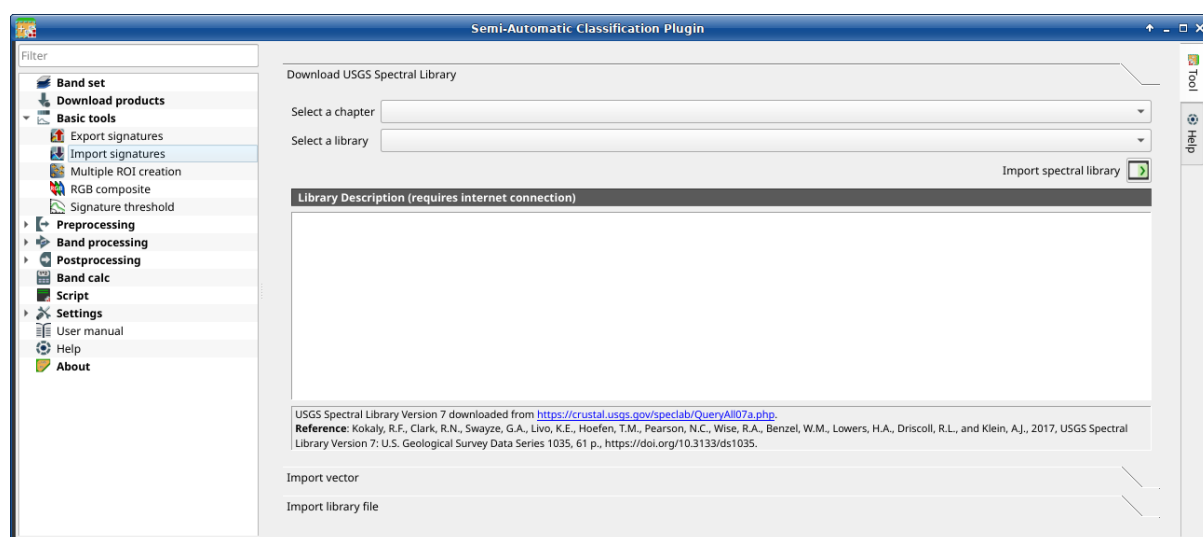
Рис. 15: Download USGS Spectral Library
