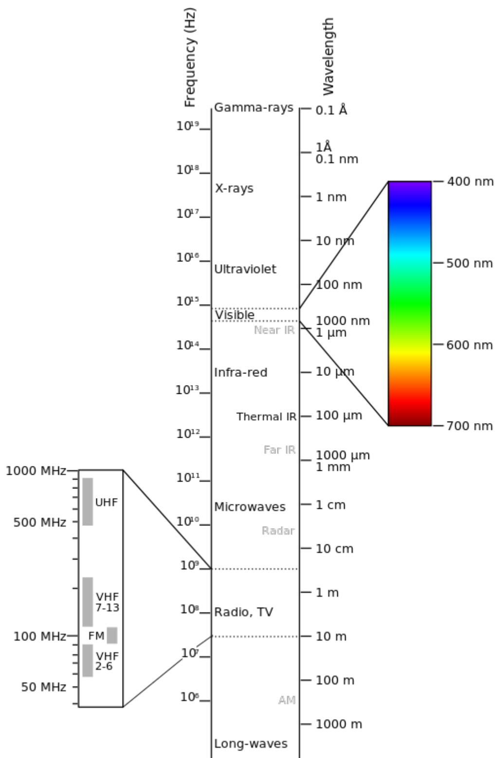
Рис. 1: Electromagnetic-Spectrum
