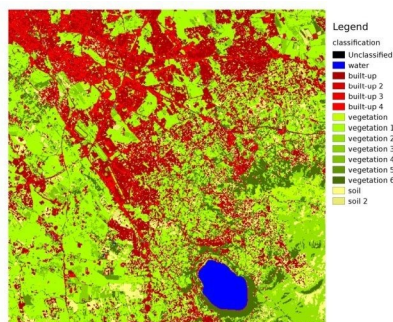
Рис. 11: Landsat classification Data available from the U.S. Geological Survey
