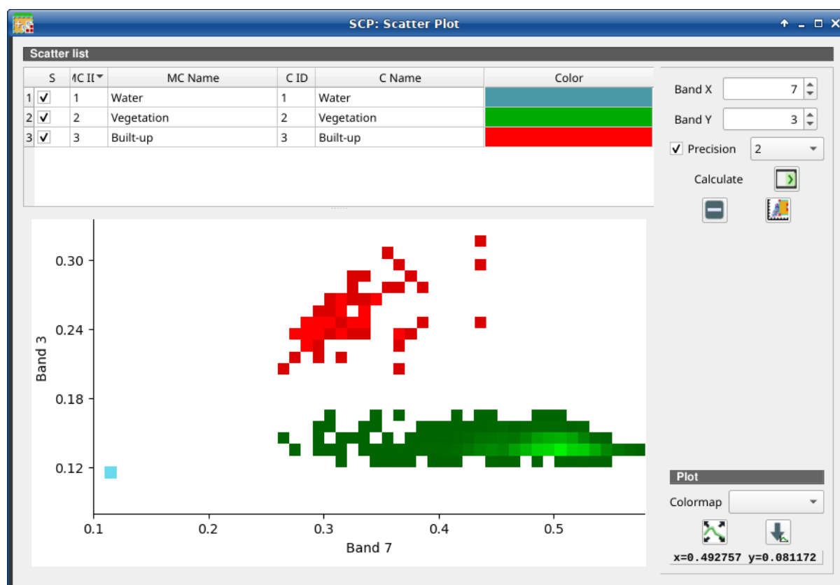
Рис. 55: Example Scatter Plot
