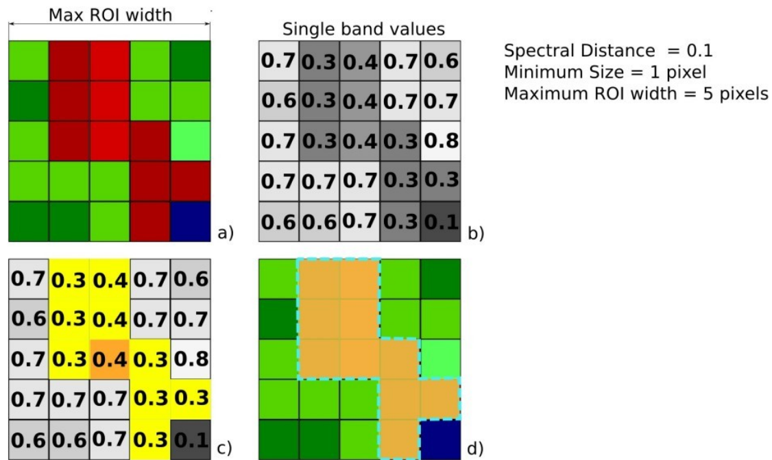
Рис. 5: Region growing example
