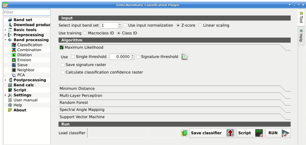
Рис. 11: Setting the algorithm and using C ID
