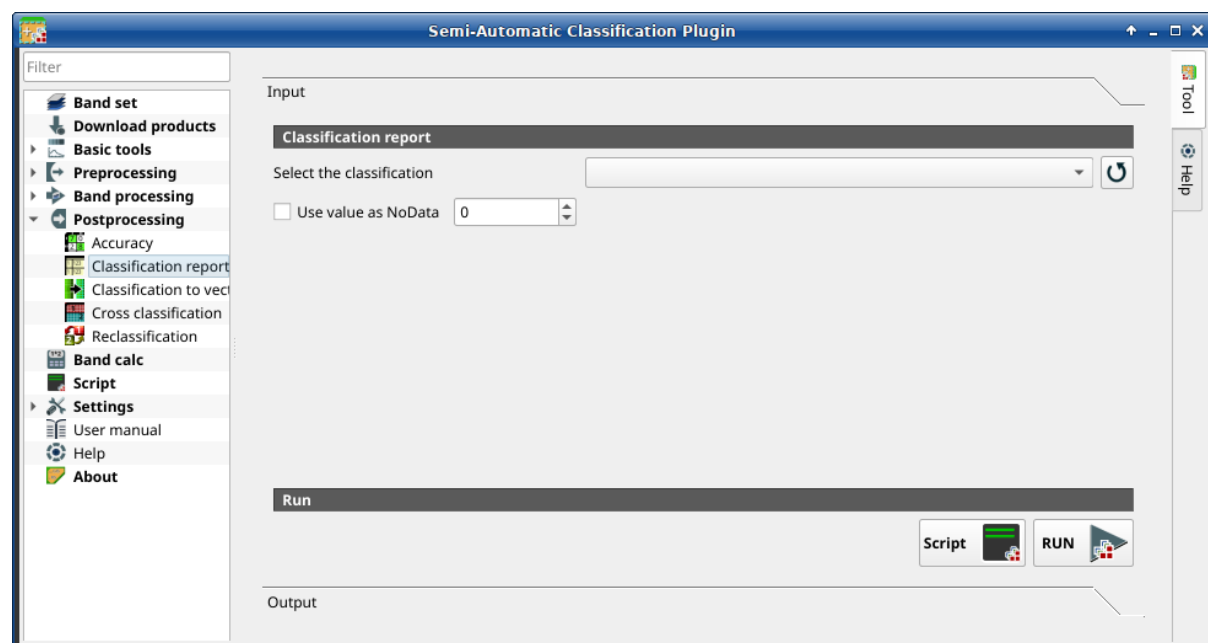
Fig. 41: Classification report
