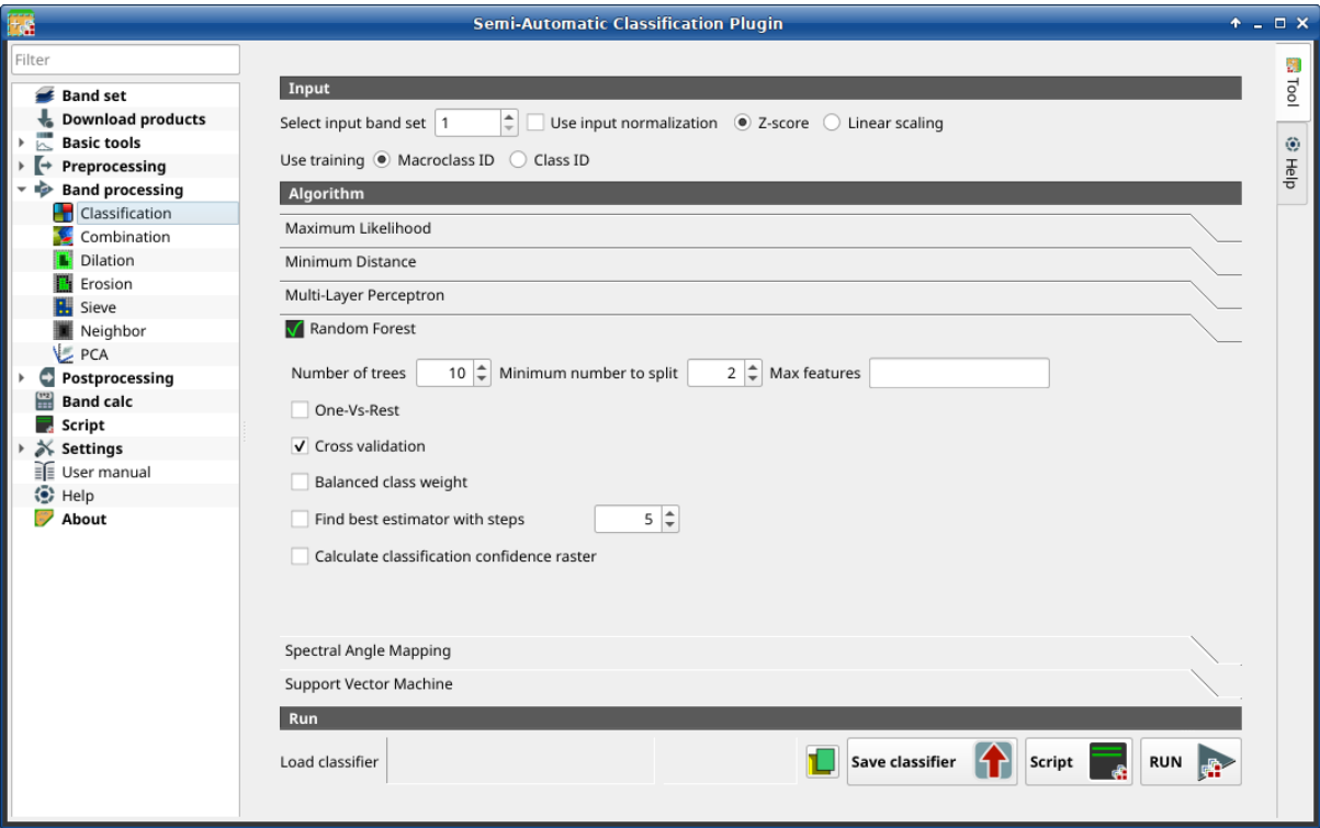
Fig. 31: Random Forest
