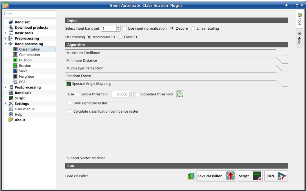
Rys. 32: Spectral Angle Mapping
