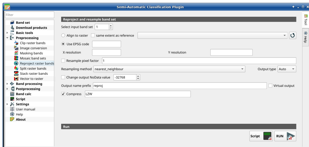
Rys. 23: Reproject raster bands
