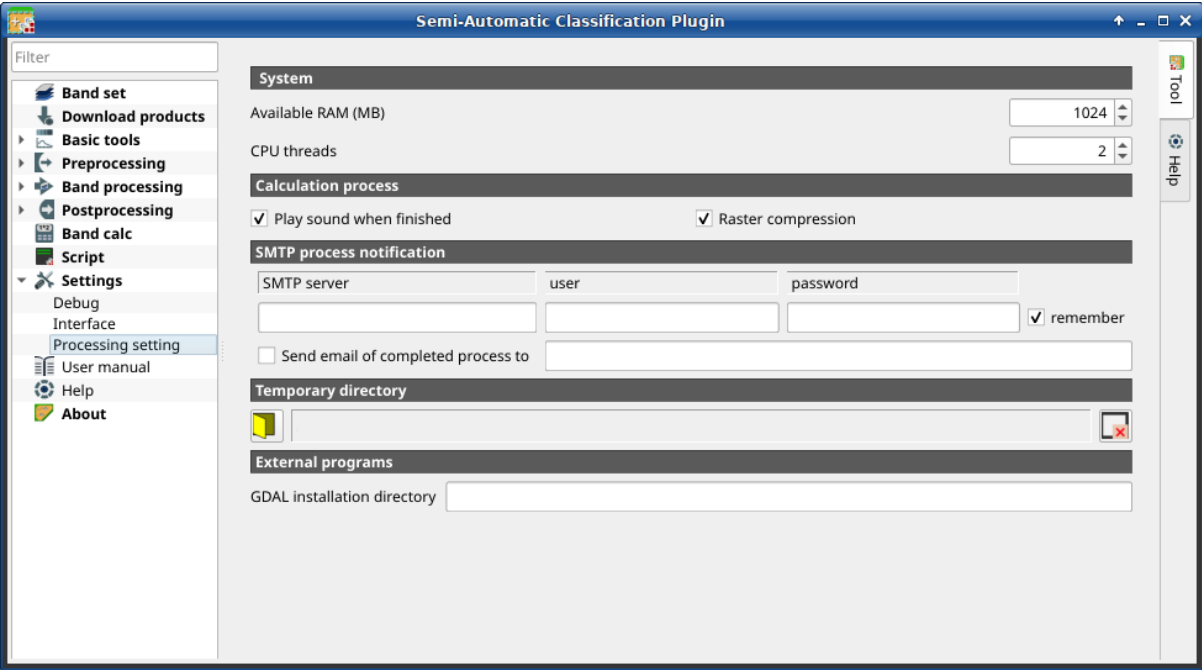
Rys. 49: Processing
