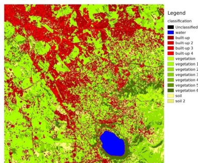
Rys. 11: Landsat classification Data available from the U.S. Geological Survey
