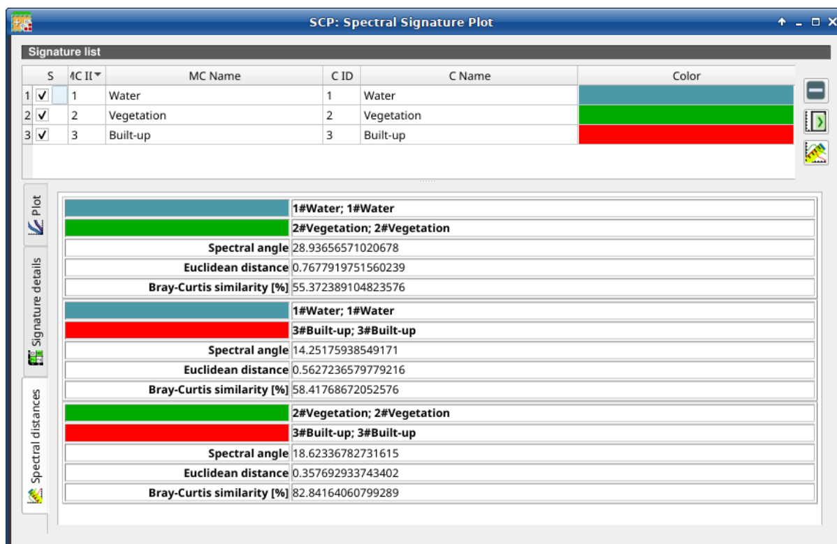
Rys. 53: Spectral Signature: Example of spectral distances
