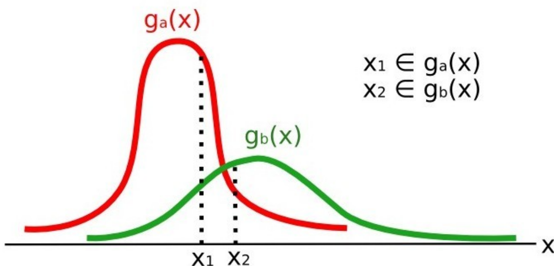
Rys. 7: Maximum Likelihood example
