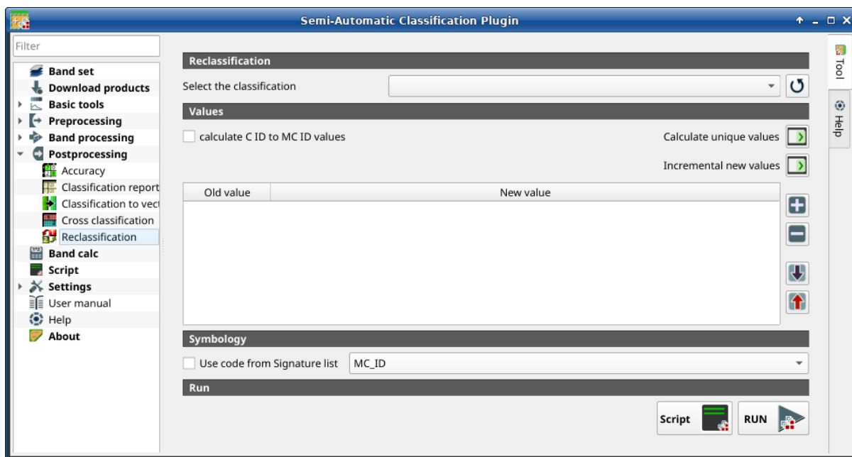
Rys. 44: Reclassification
