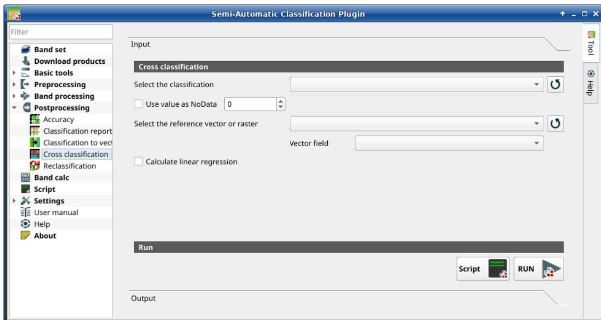
Rys. 43: Cross classification
