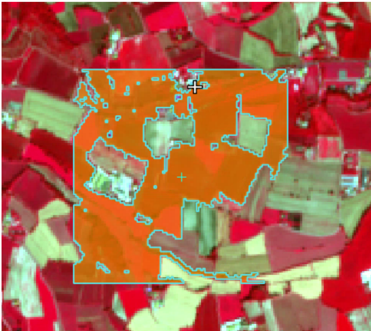
Rys. 8: Vegetation. Color composite RGB = 7-3-2
