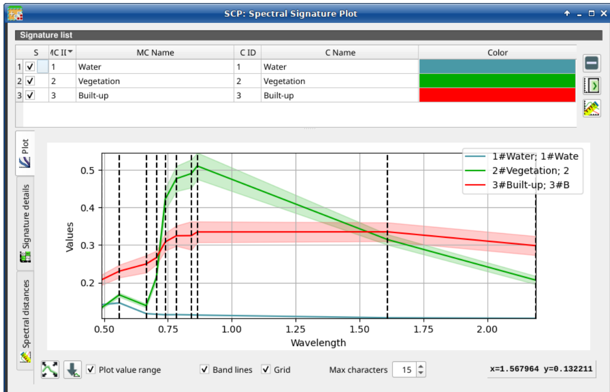
Rys. 51: Spectral Signature: Example of plot
