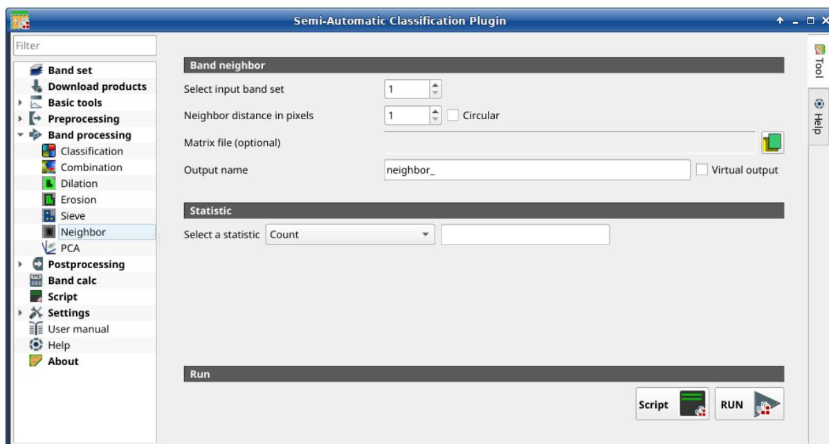
Rys. 38: Neighbor
