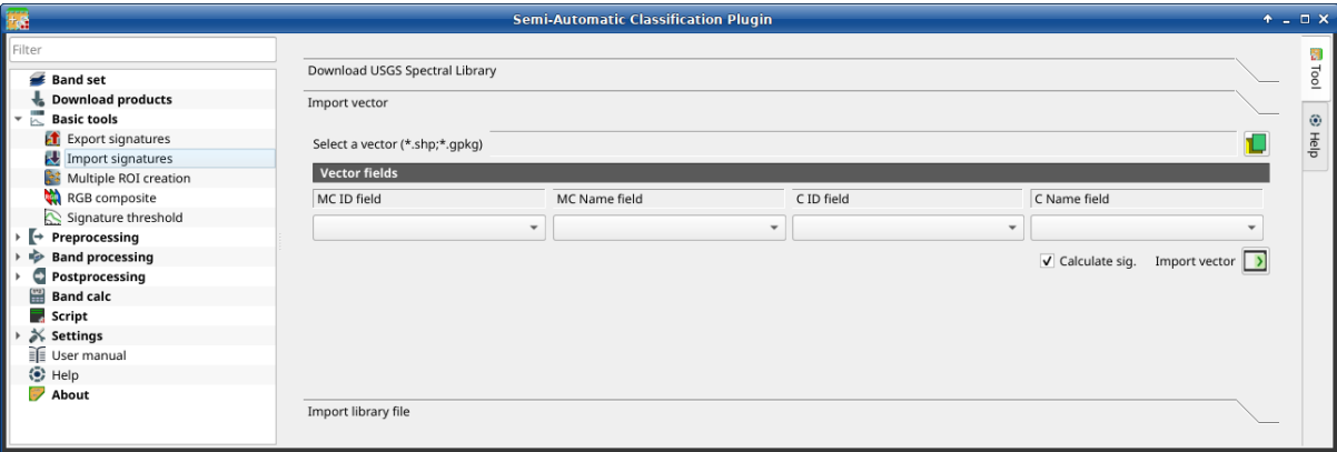
Rys. 14: Import vector
