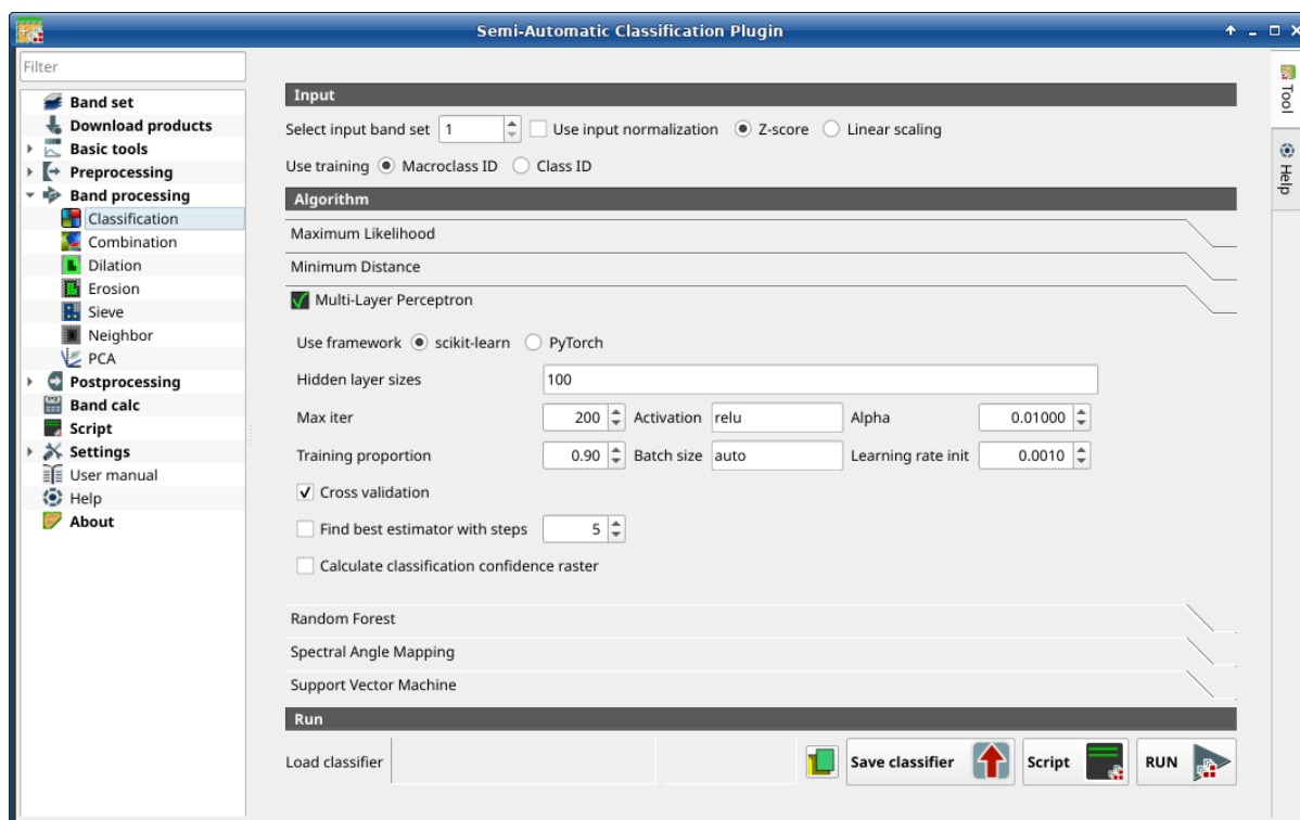
Rys. 30: Multi-layer Perceptron
