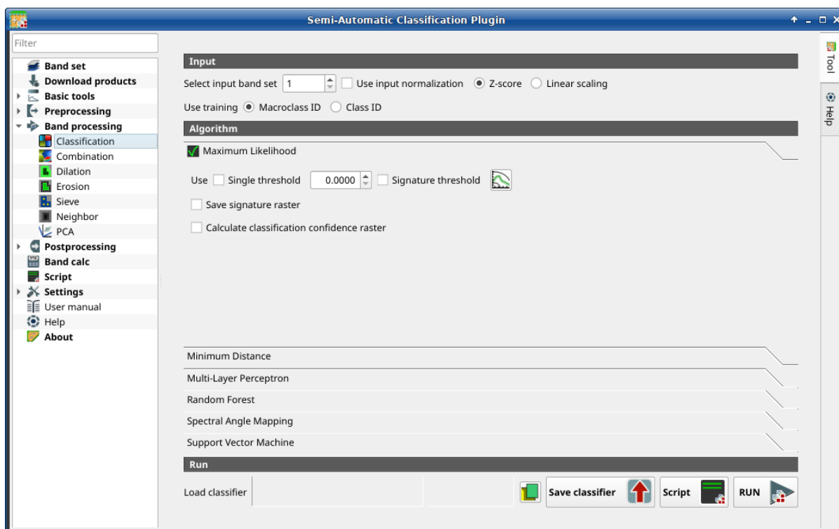
Rys. 27: Classification
