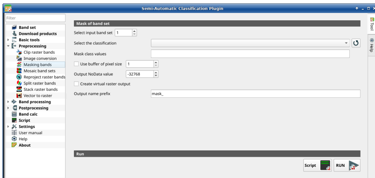
Rys. 21: Masking bands
