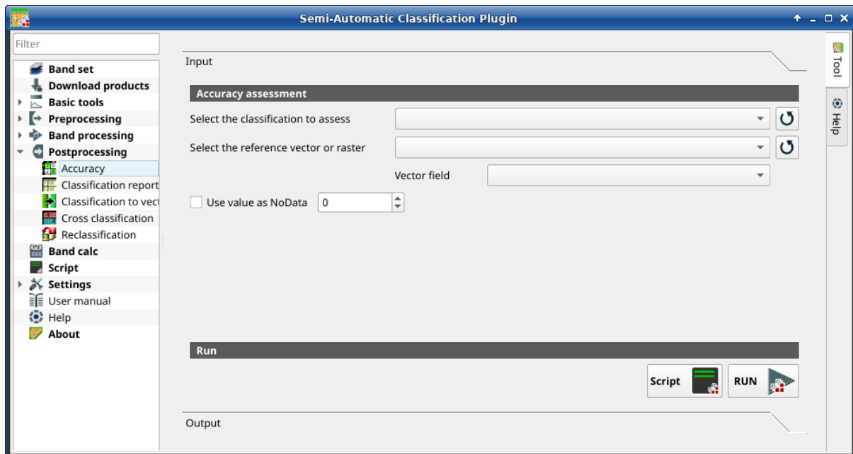
Rys. 40: Accuracy
