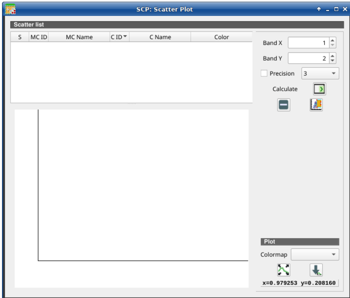
Rys. 54: Scatter Plot
