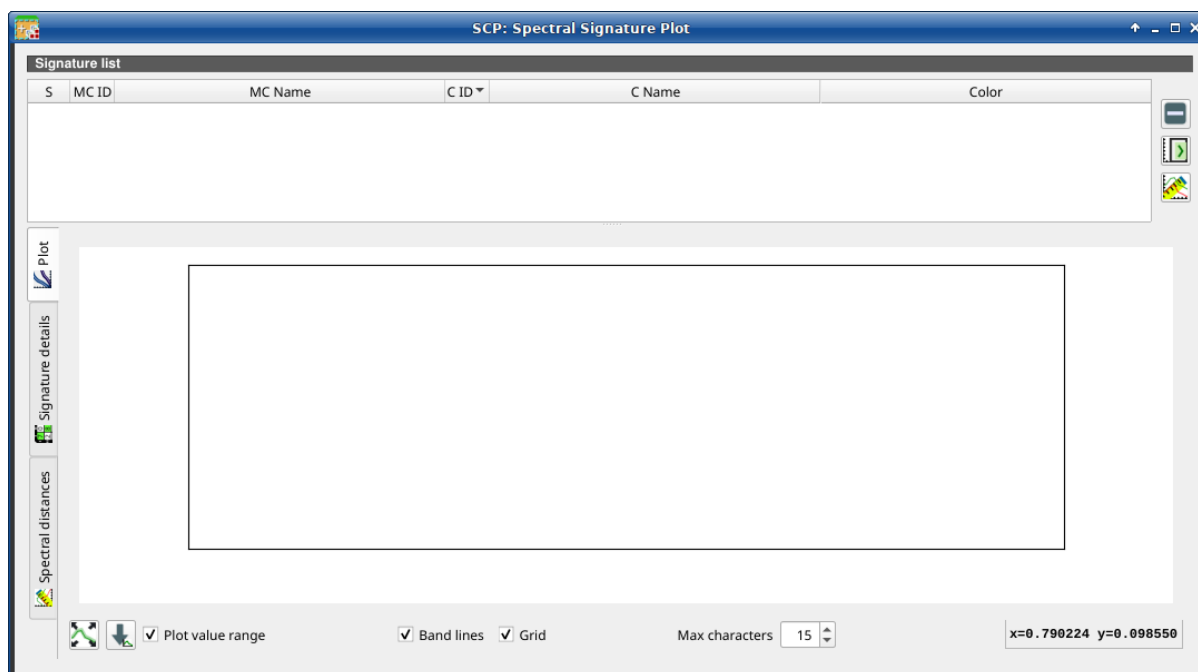
Rys. 50: Spectral Signature Plot
