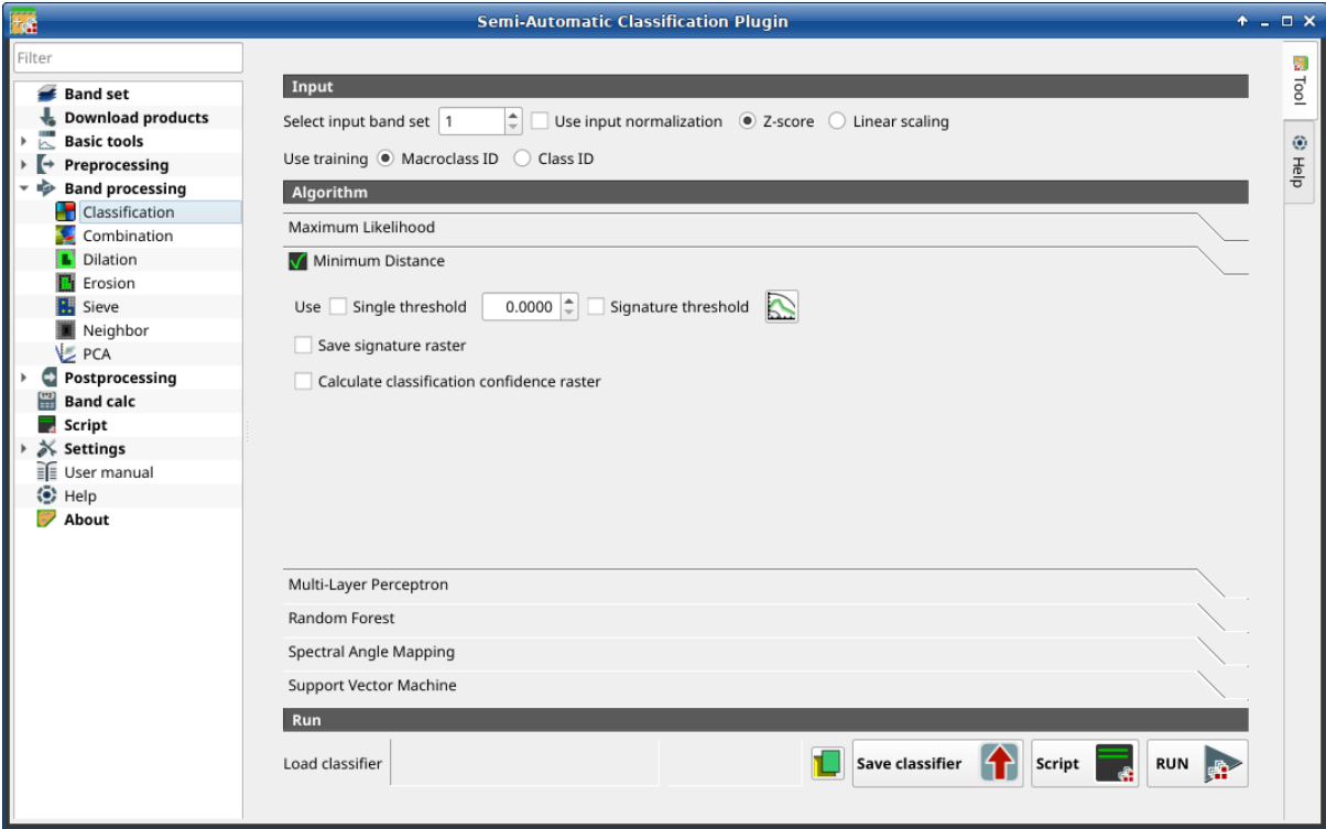
Rys. 29: Minimum Distance
