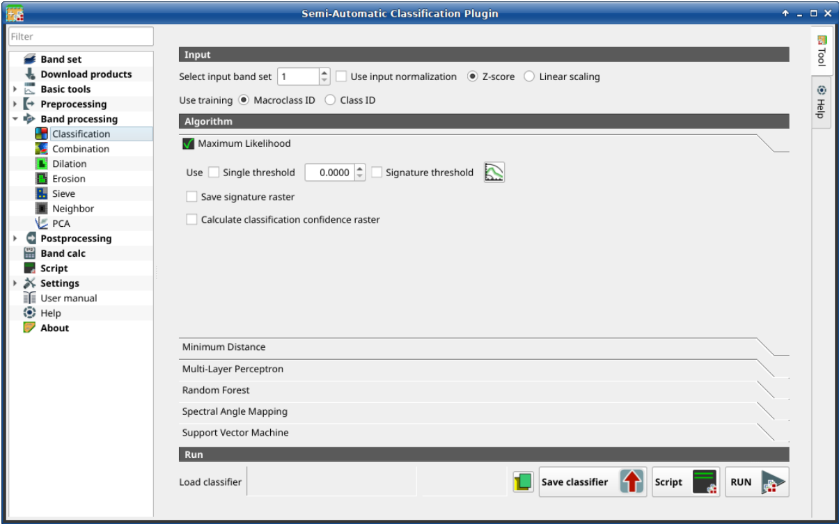
Rys. 28: Maximum Likelihood
