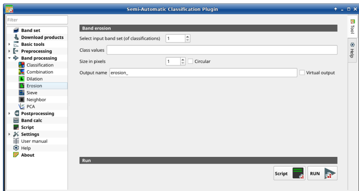
Rys. 36: Erosion
