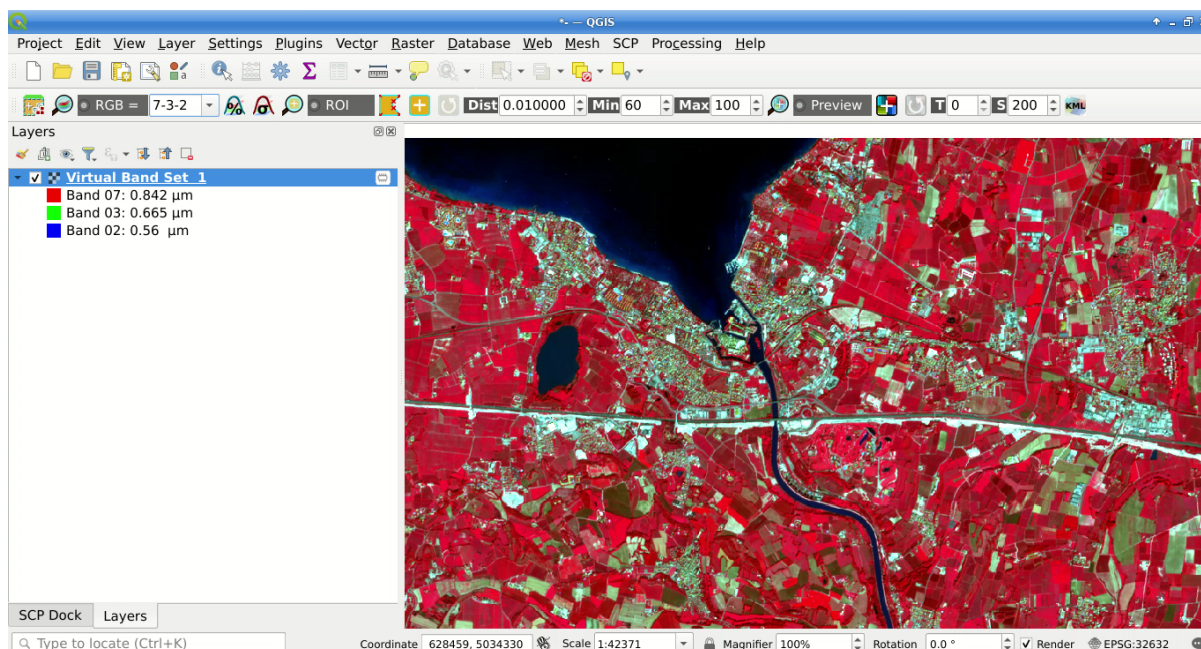
Rys. 2: Color composite RGB=7-3-2
