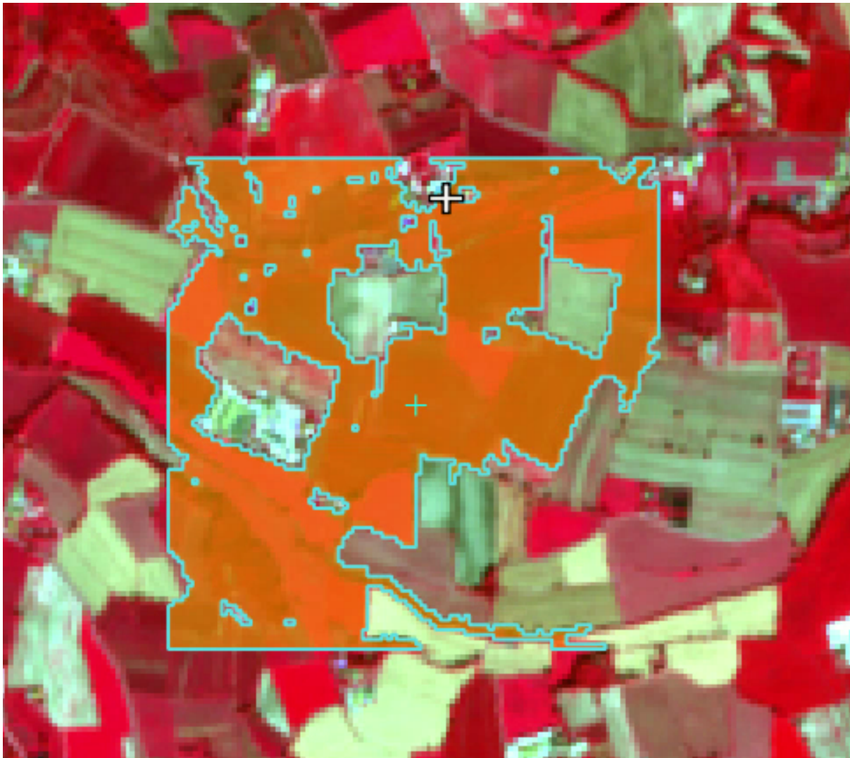
8: Vegetation. Color composite RGB = 7-3-2
