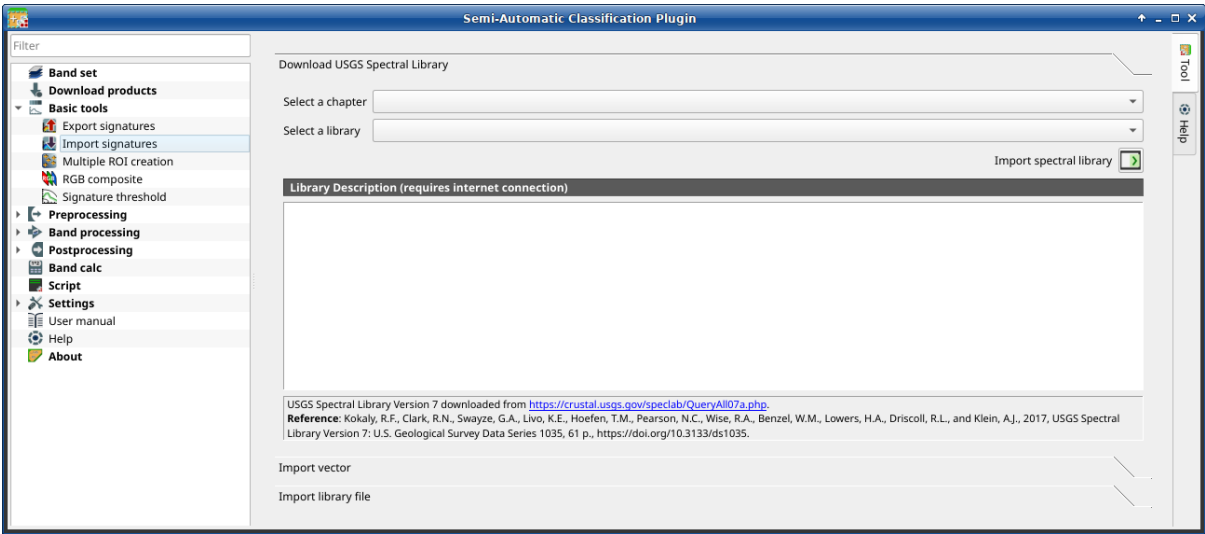
15: Download USGS Spectral Library
