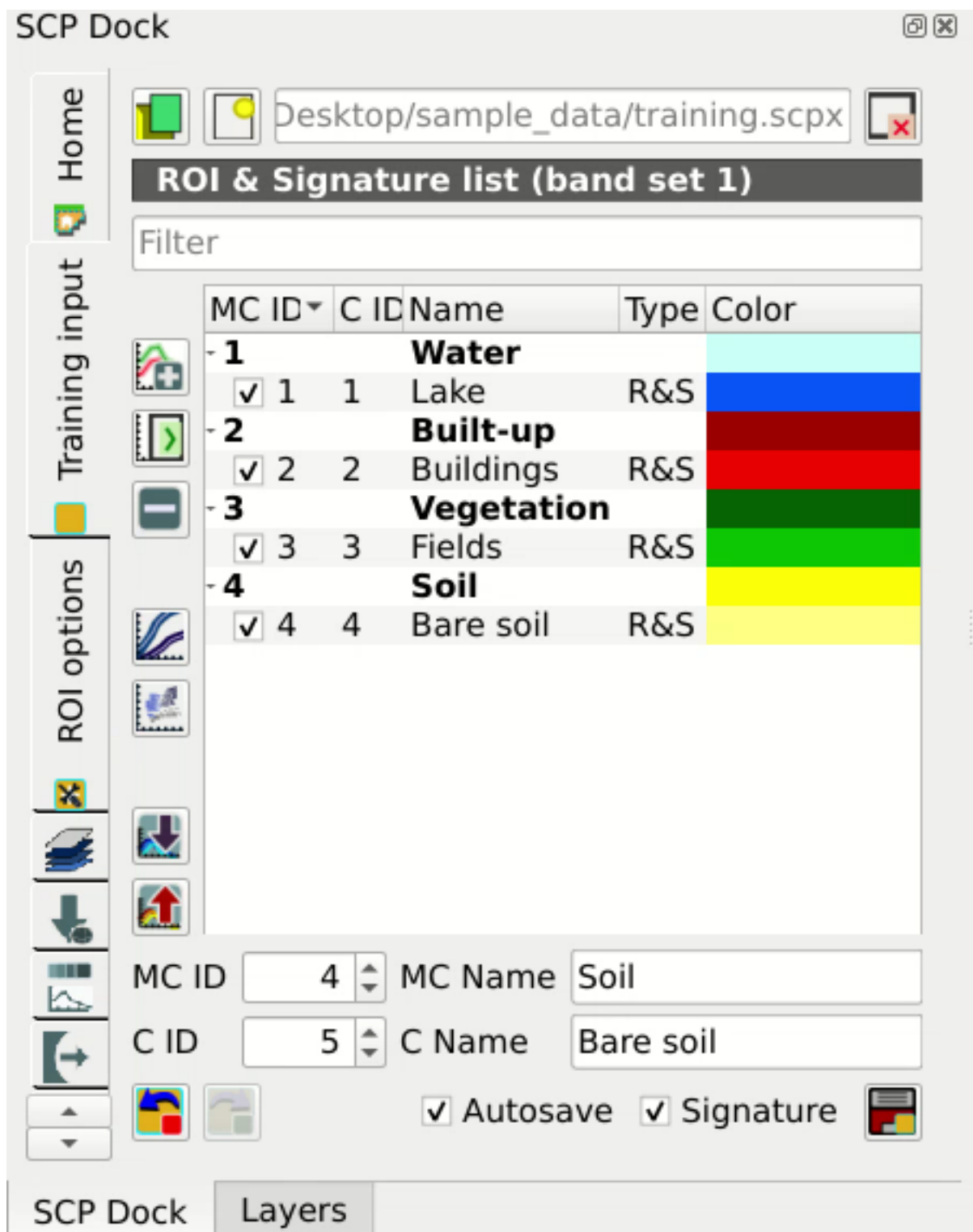
10: Definition of class colors
