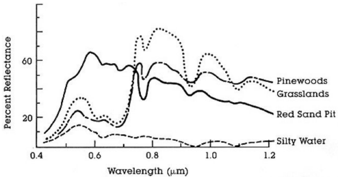
2: Spectral Reflectance Curves of Four Different Targets (from NASA, 2013)
