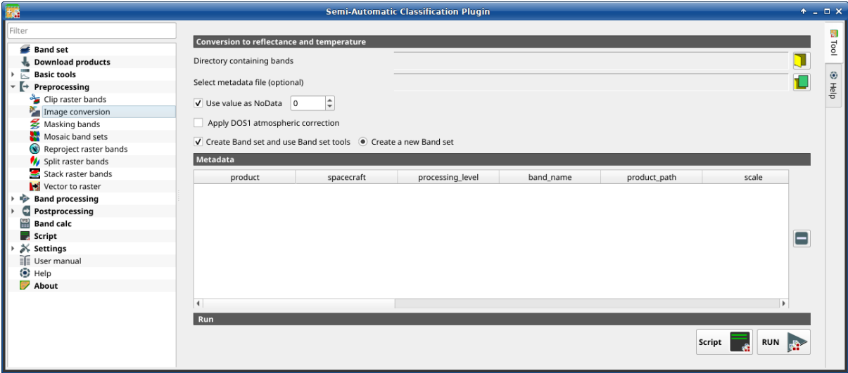
20: Image conversion
