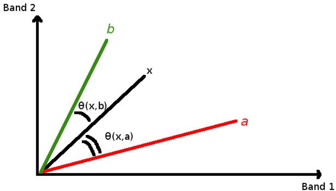
8: Spectral Angle Mapping example
