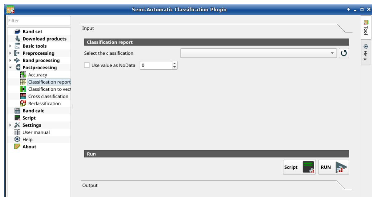
41: Classification report
