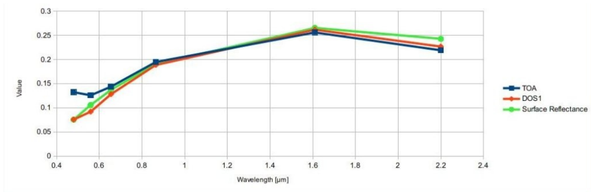
13: Spectral signatures of a built-up pixel
