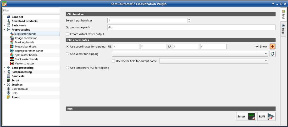
19: Clip multiple rasters
