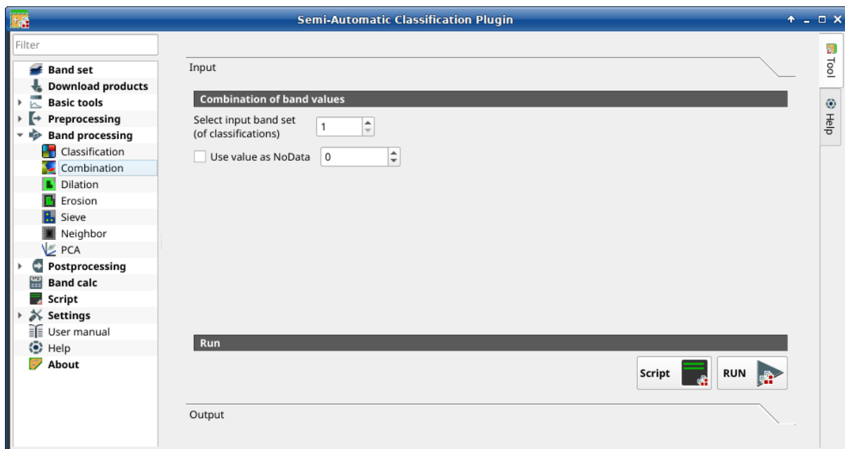
34: Combination
