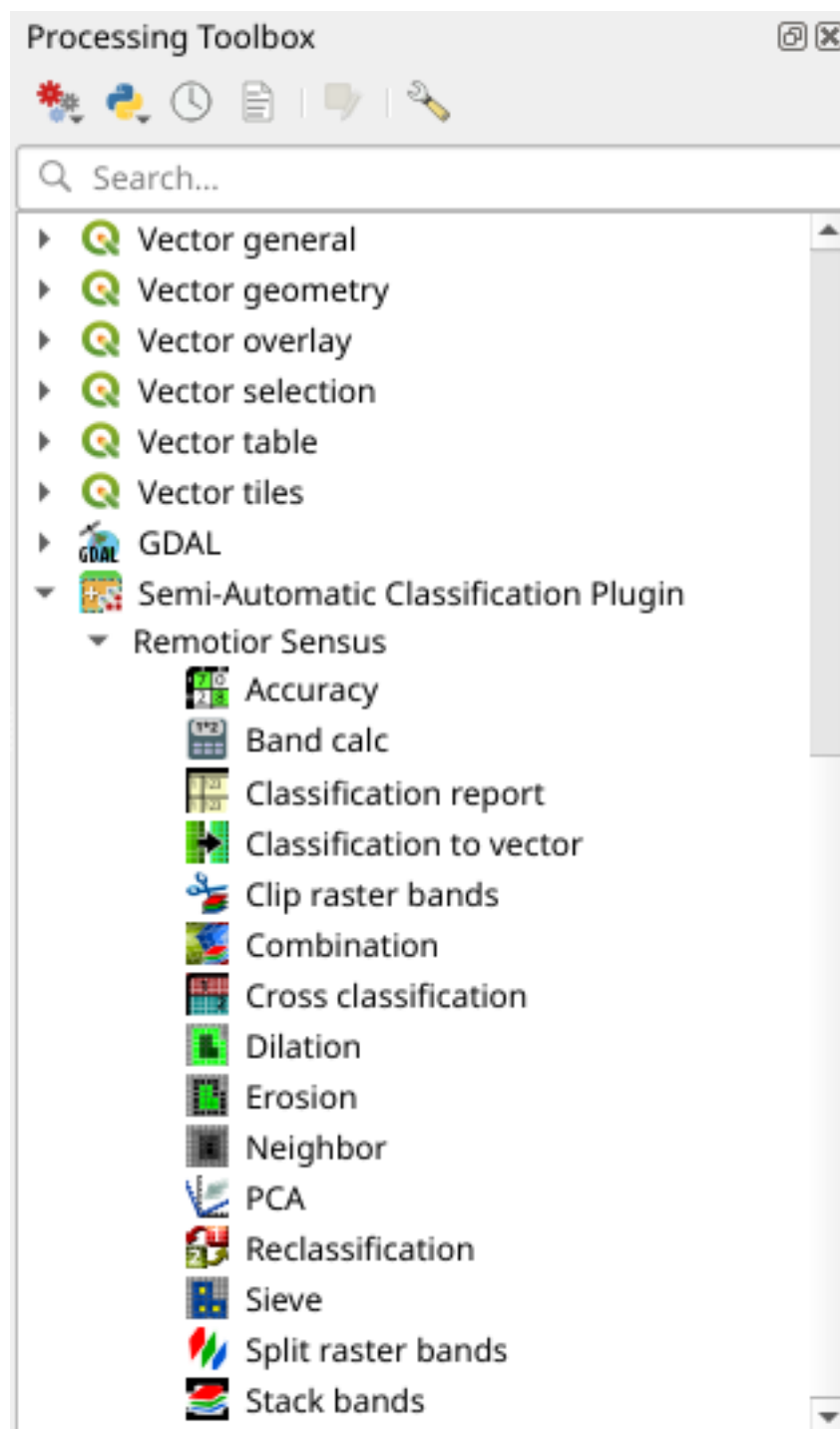
56: Integration in QGIS Processing Toolbox
