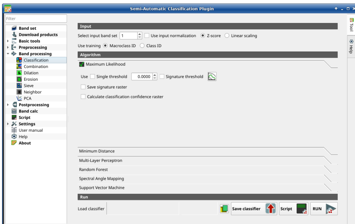
27: Classification
