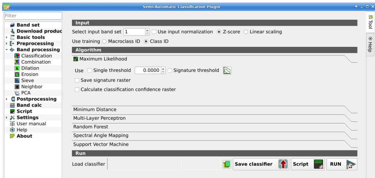
11: Setting the algorithm and using C ID
