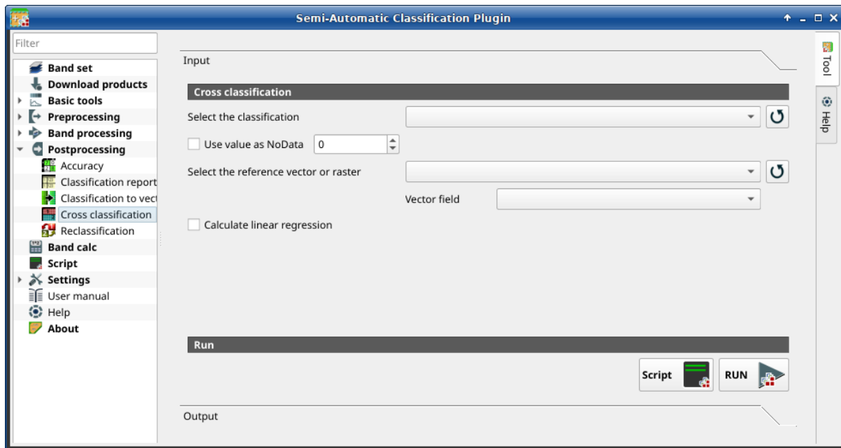
43: Cross classification
