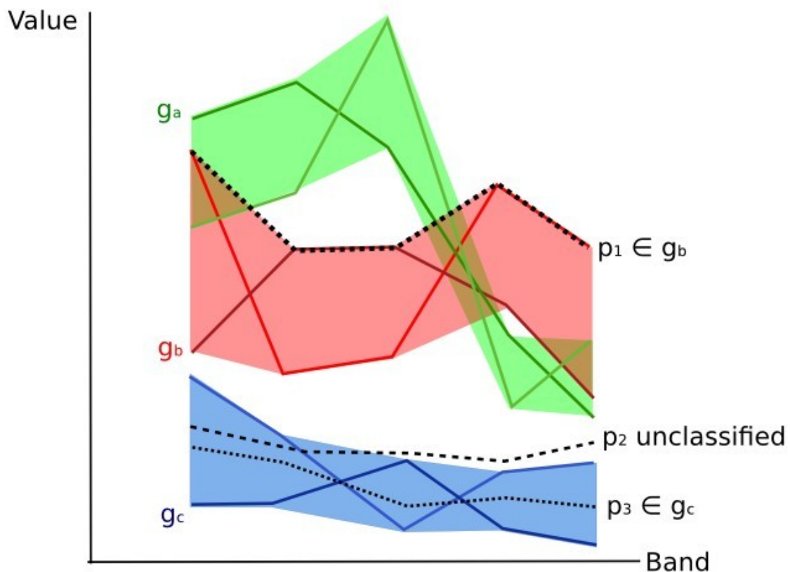
10: Plot of spectral ranges
