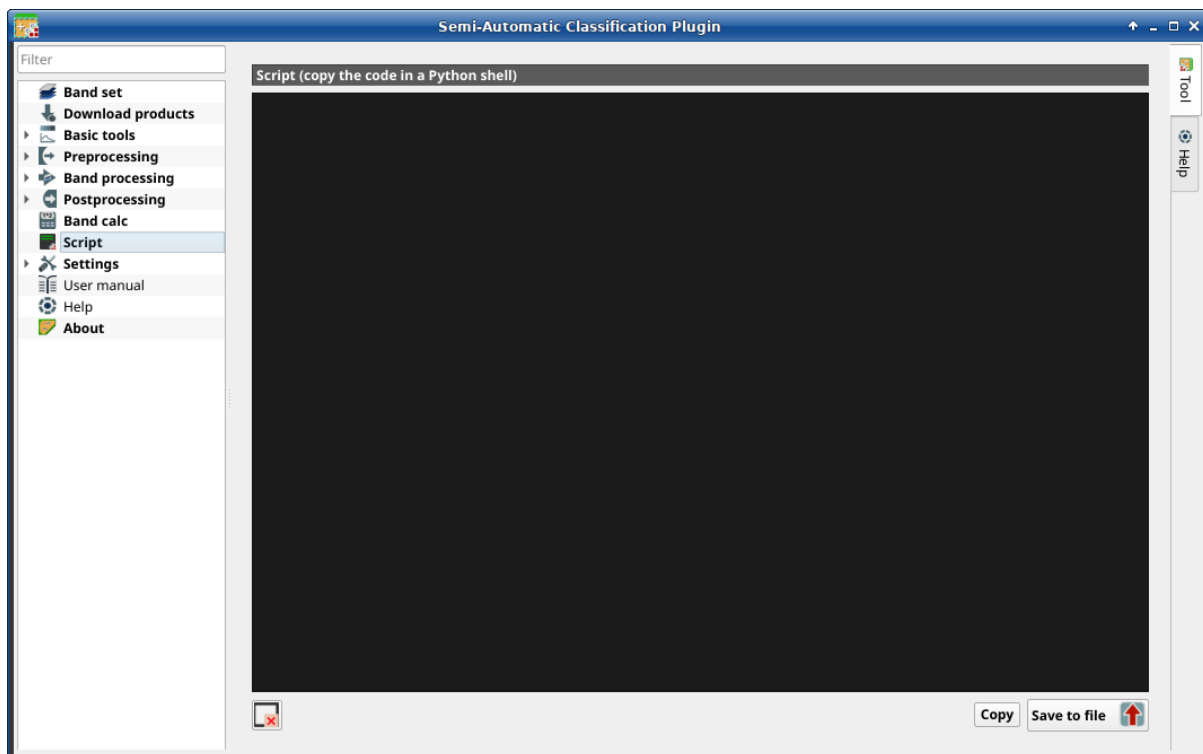
46: Script
