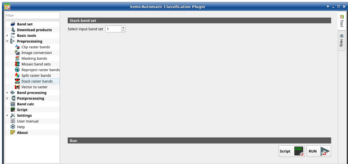
25: Stack raster bands
