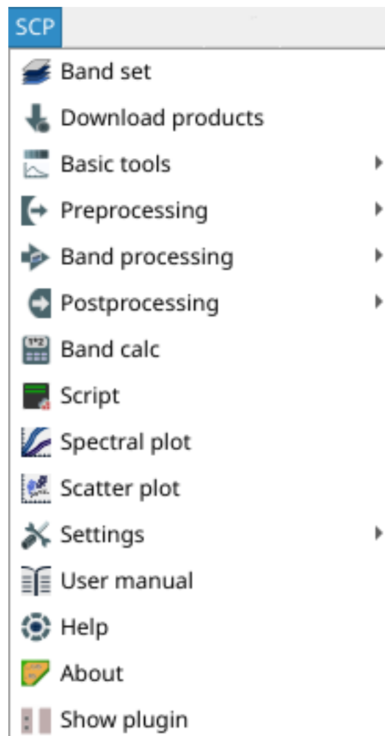
1: SCP menu
