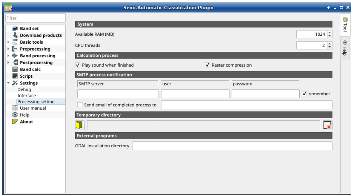
49: Processing
