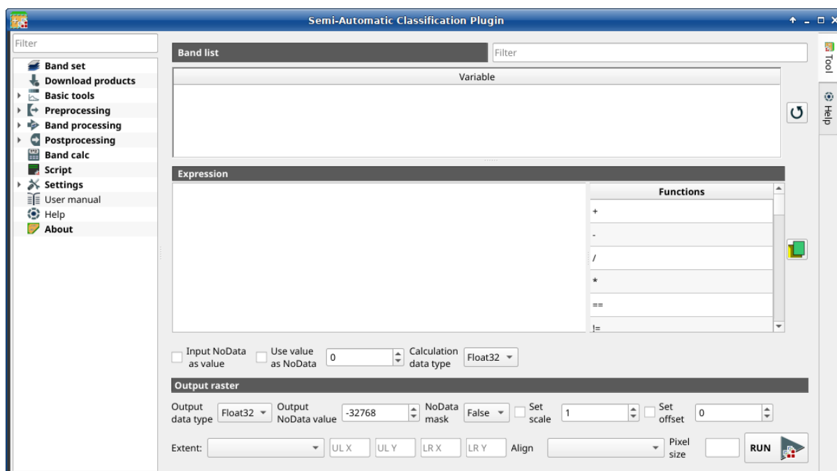
45: Band calc
