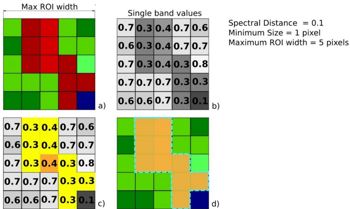
5: Region growing example
