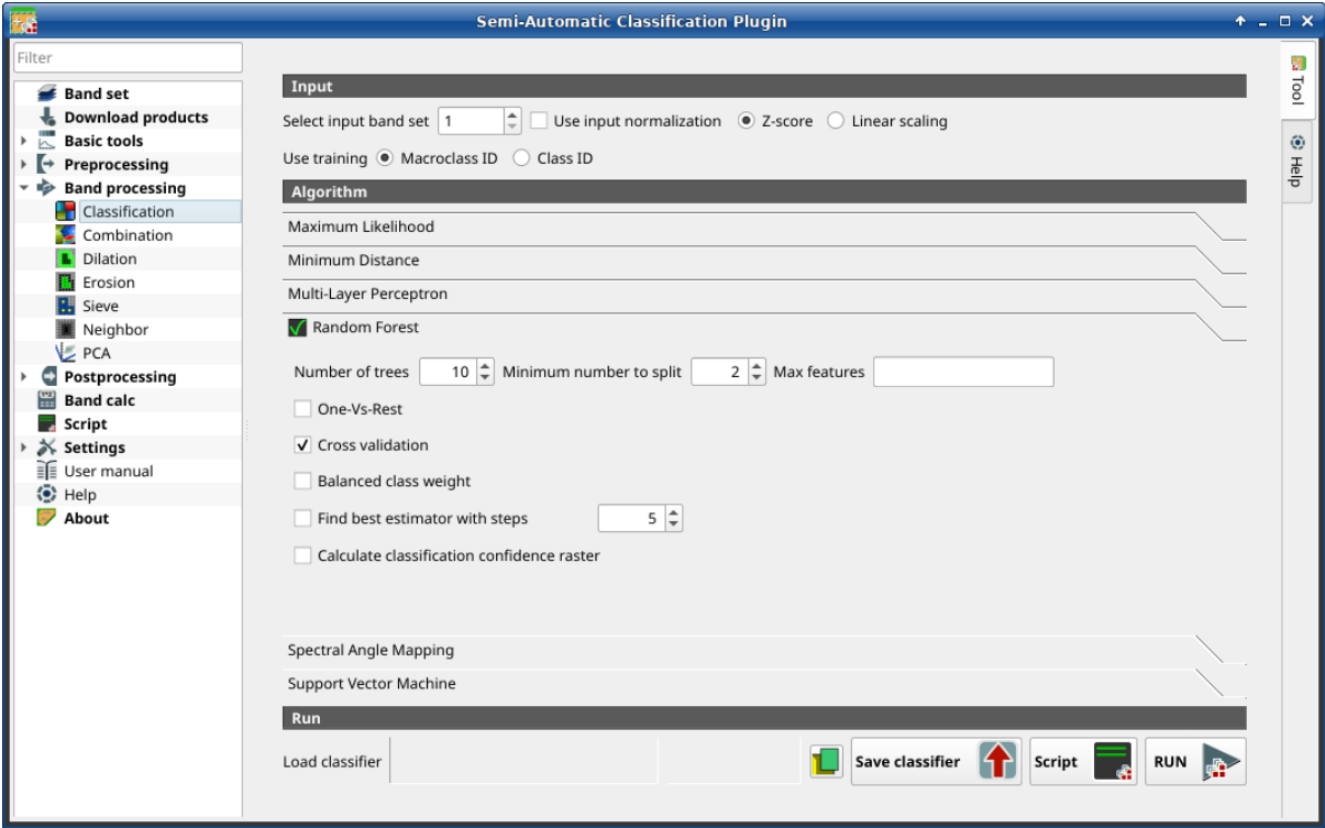
31: Random Forest
