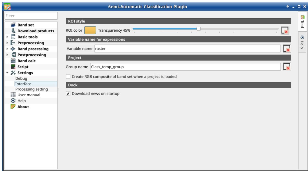
48: Interface
