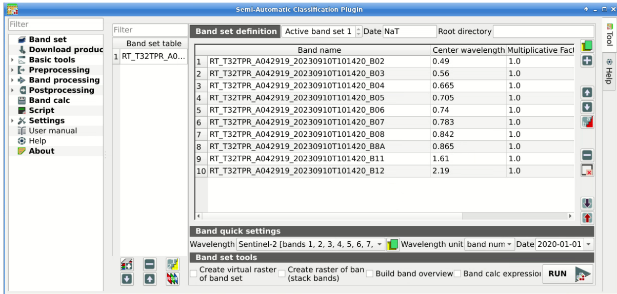
1: Definition of a band set
