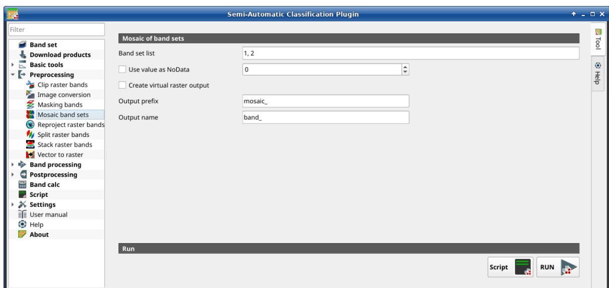
22: Mosaic band sets
