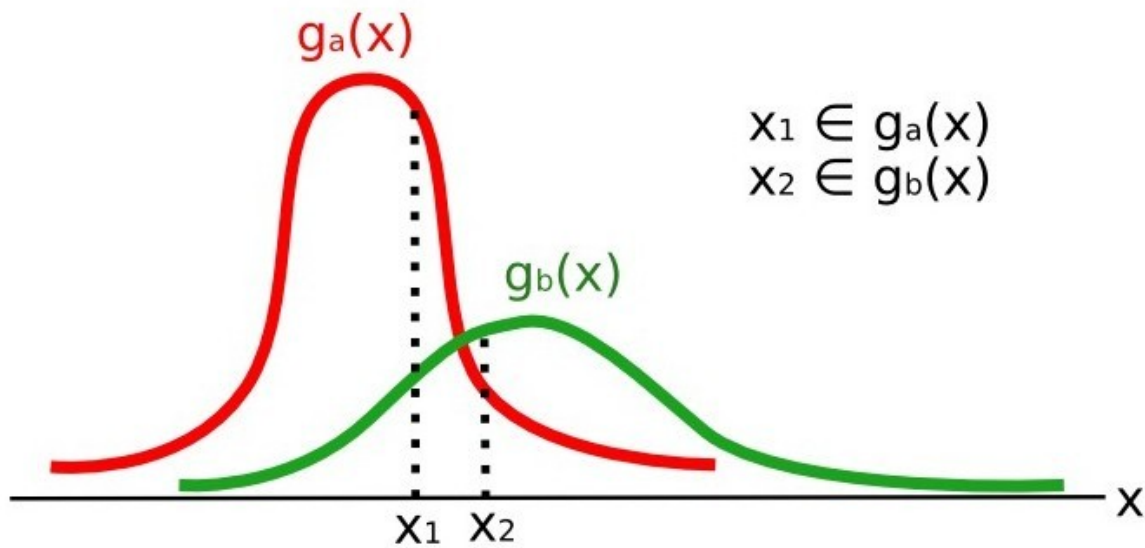
7: Maximum Likelihood example
