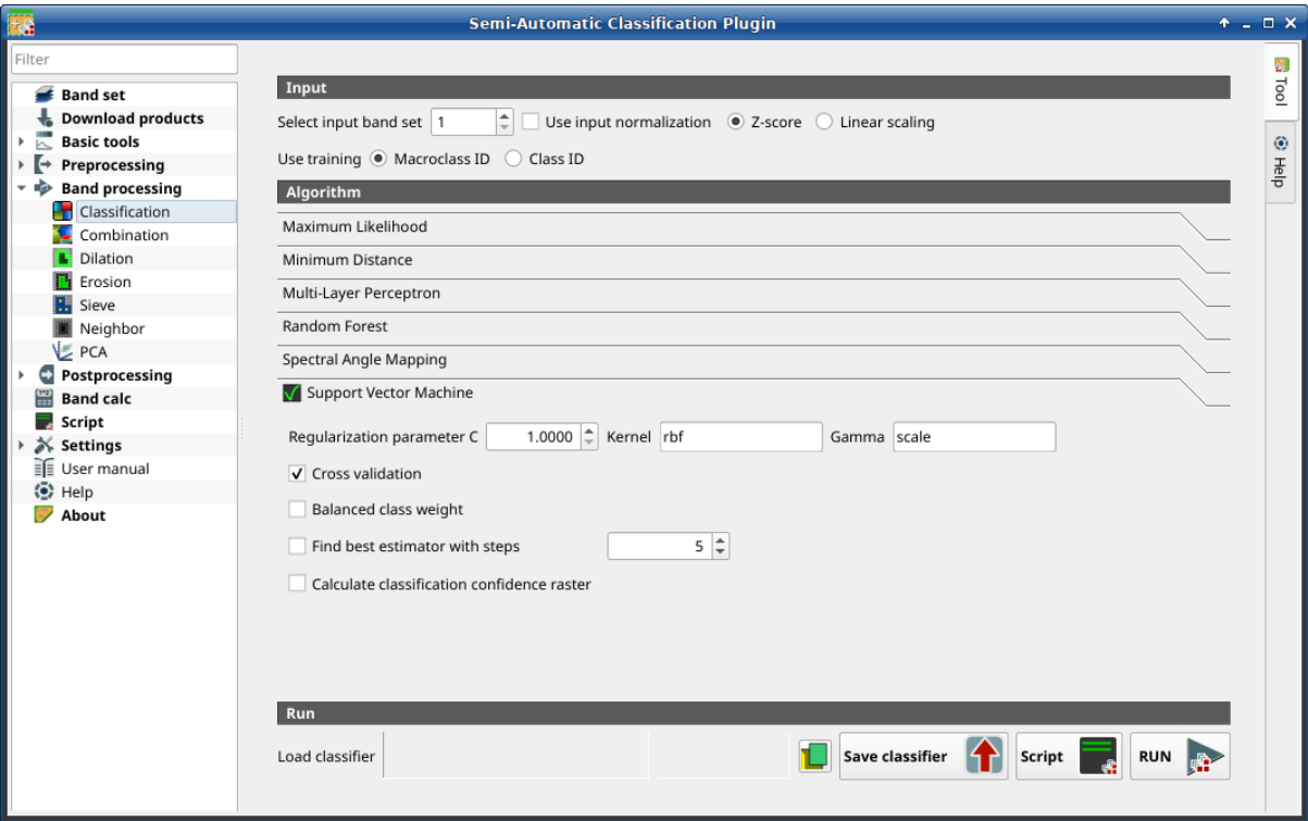
33: Support Vector Machine
