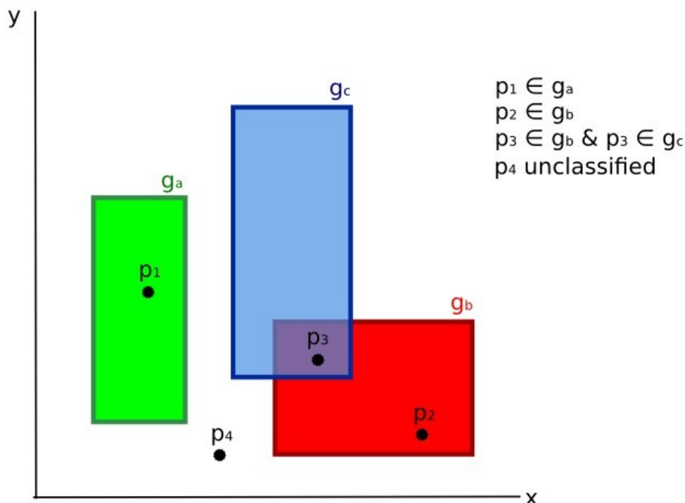
9: Land cover signature classification
