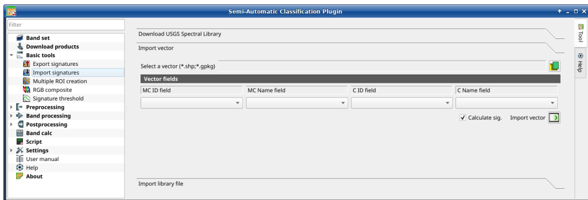
14: Import vector
