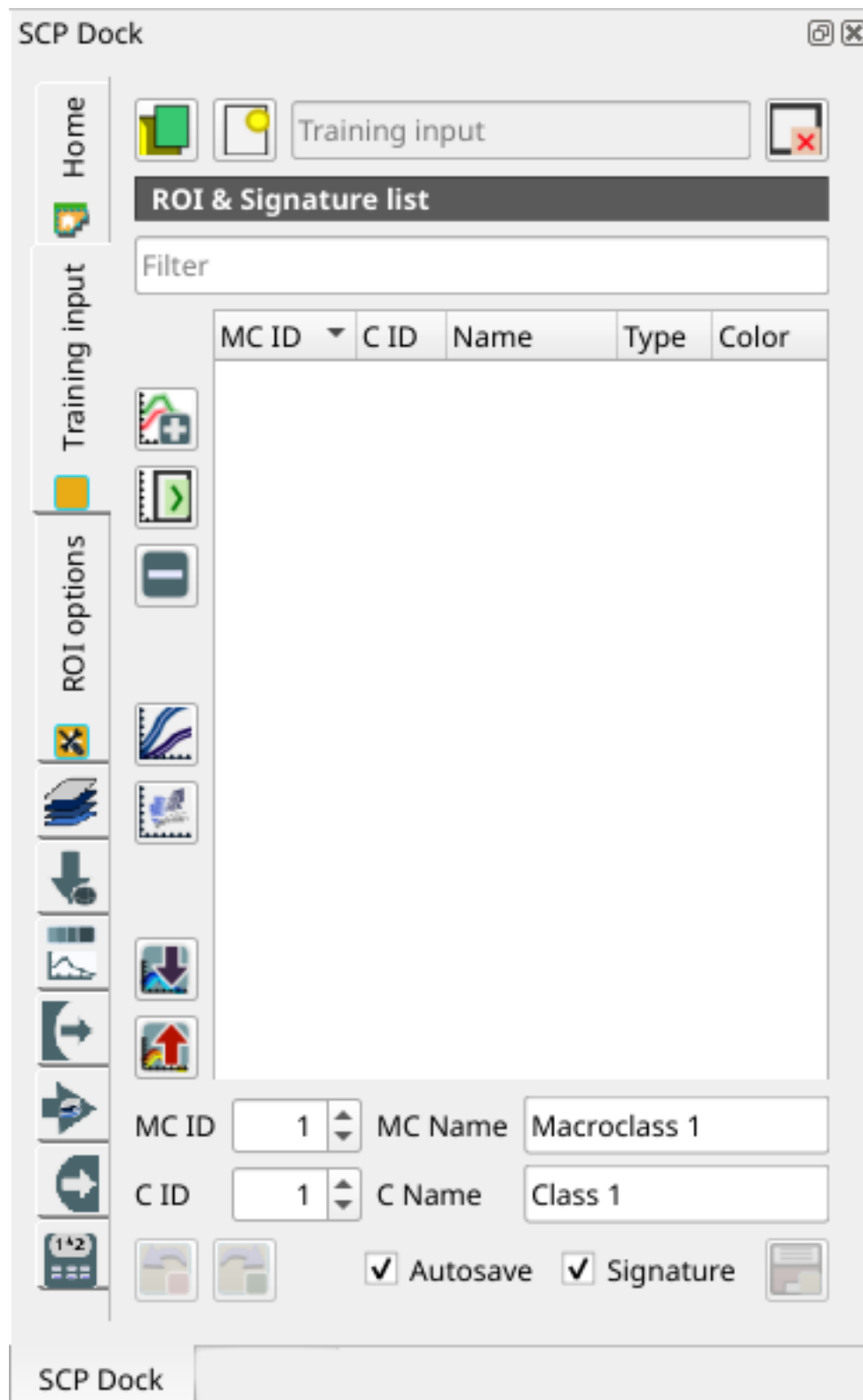
4: Training input
