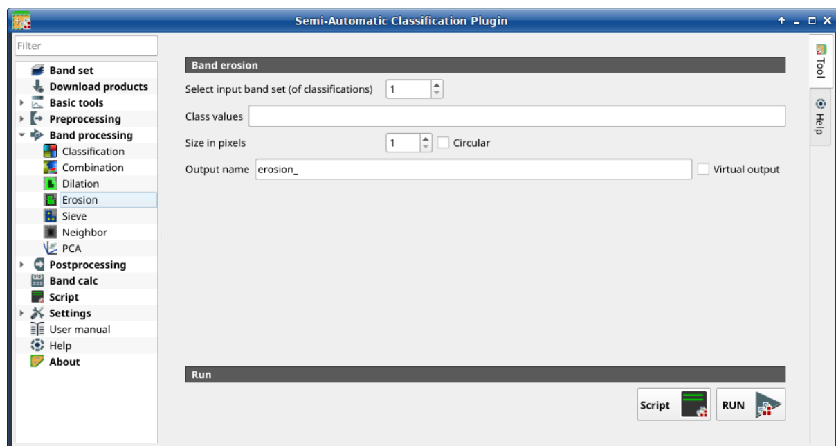
36: Erosion
