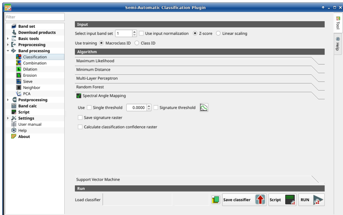
32: Spectral Angle Mapping
