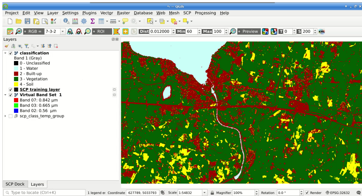
14: Result of the land cover classification
