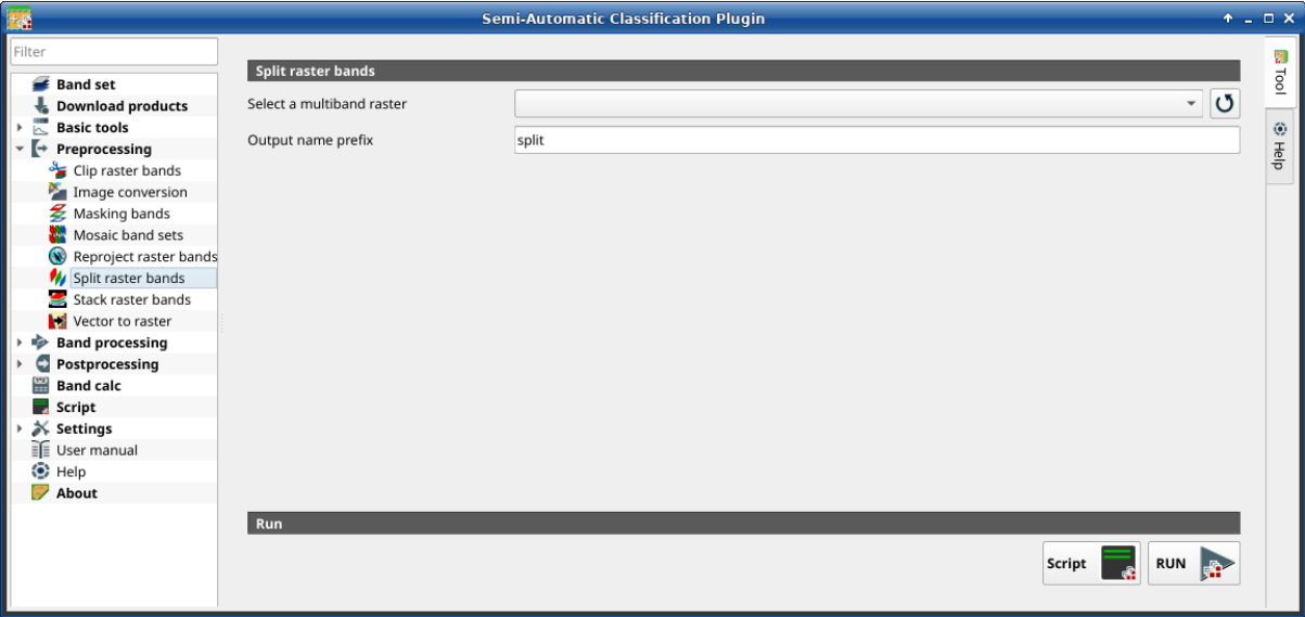
24: Split raster bands
