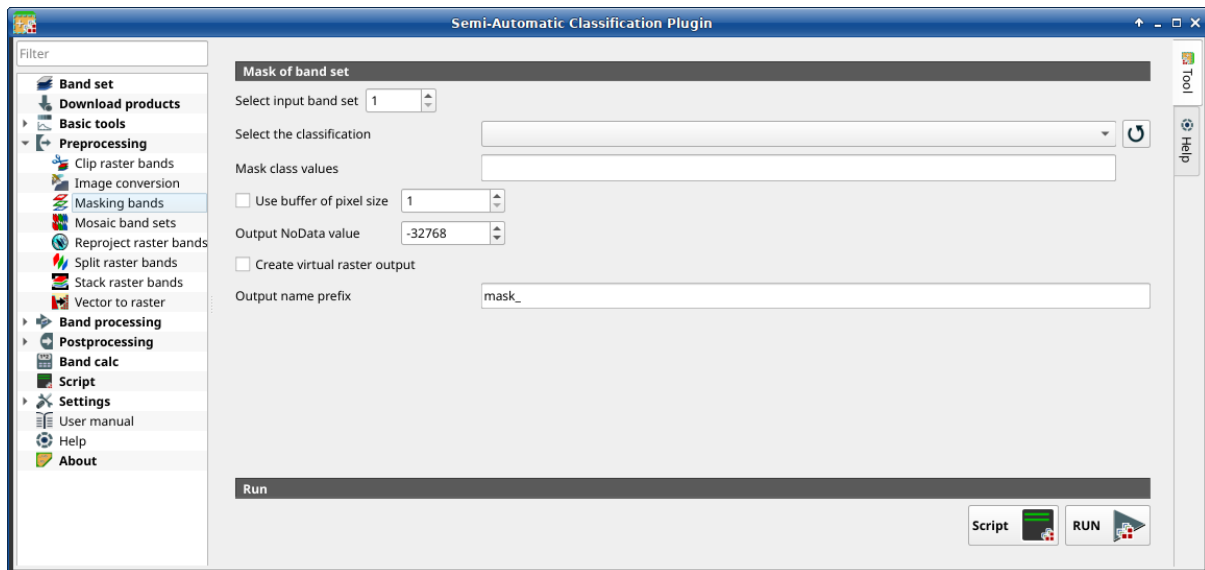
21: Masking bands
