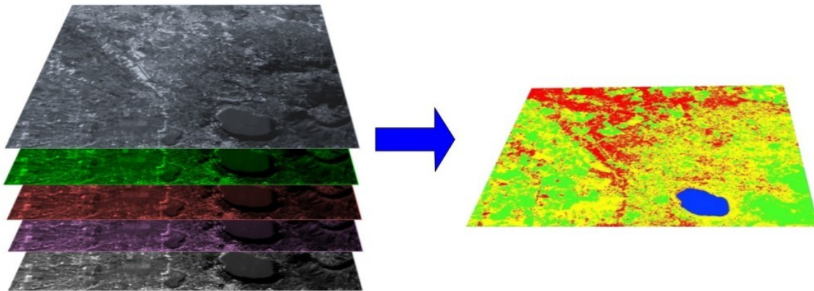
3: A multispectral image processed to produce a land cover classification (Landsat image provided by USGS)
