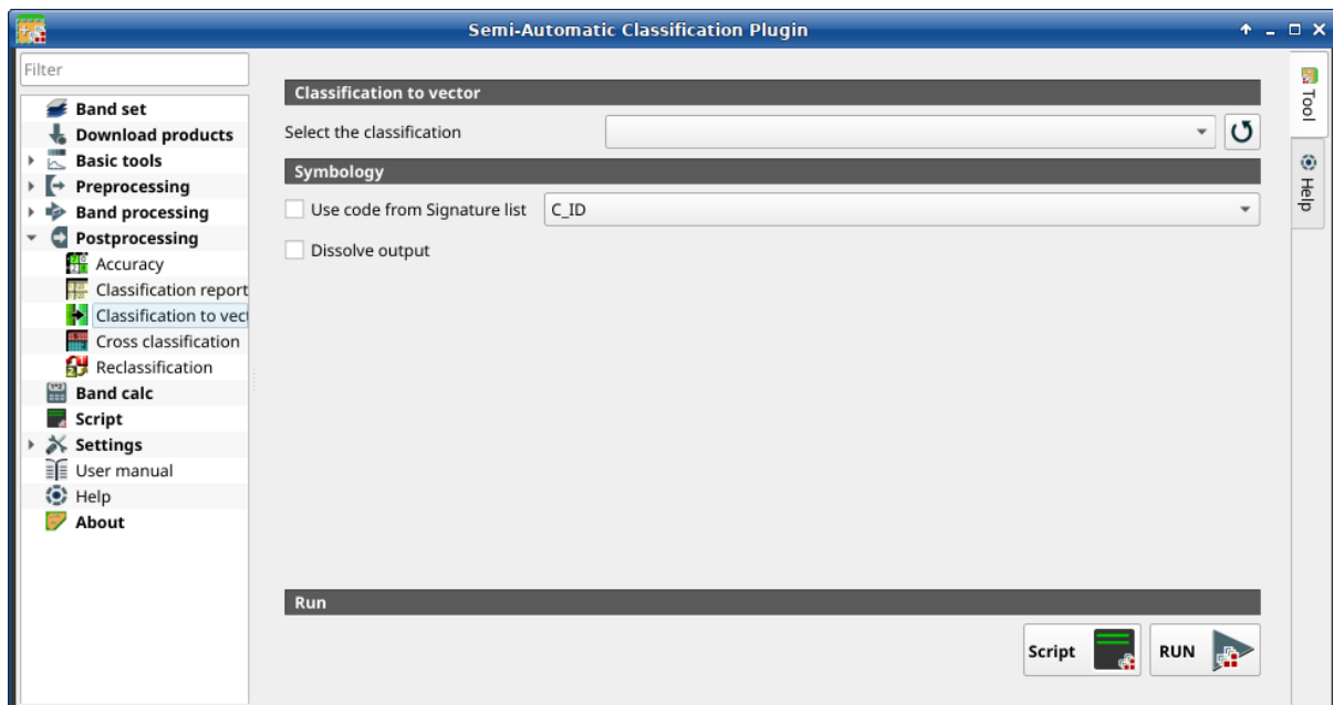
42: Classification to vector
