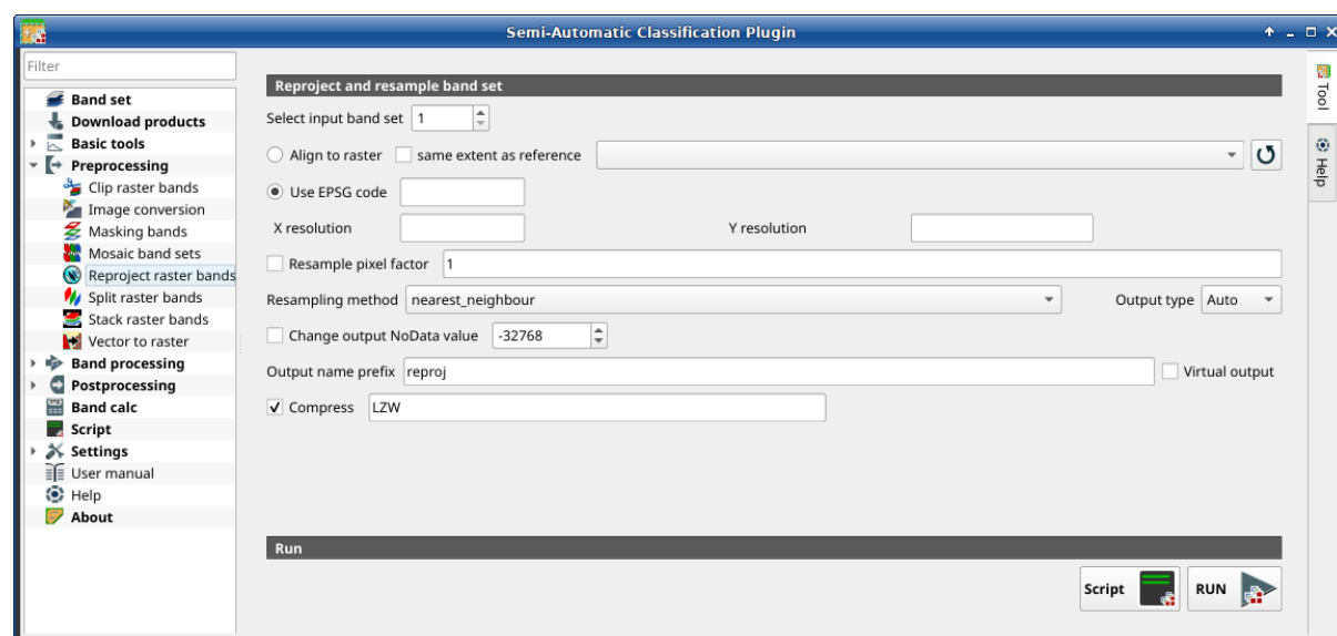
23: Reproject raster bands
