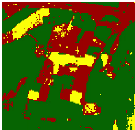
15: Example of error: Soil classified as Built-up
