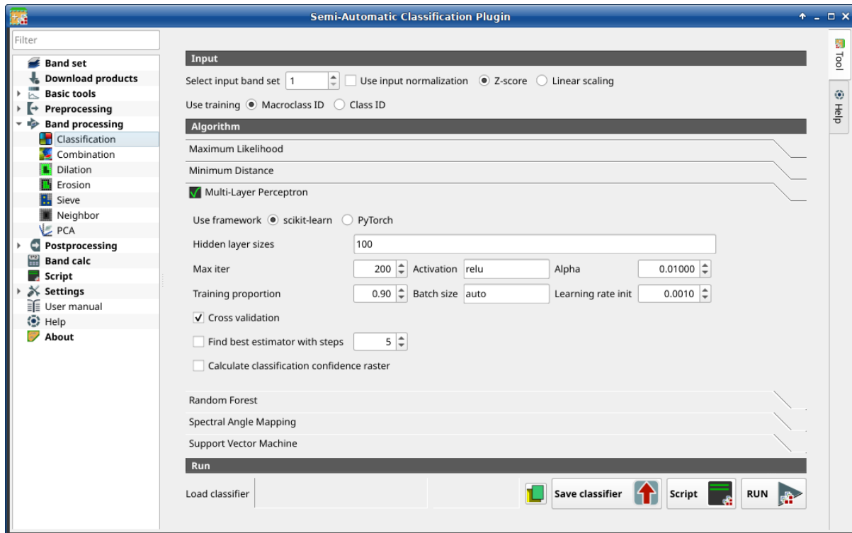
30: Multi-layer Perceptron
