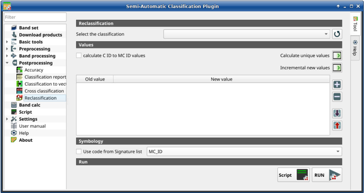
44: Reclassification
