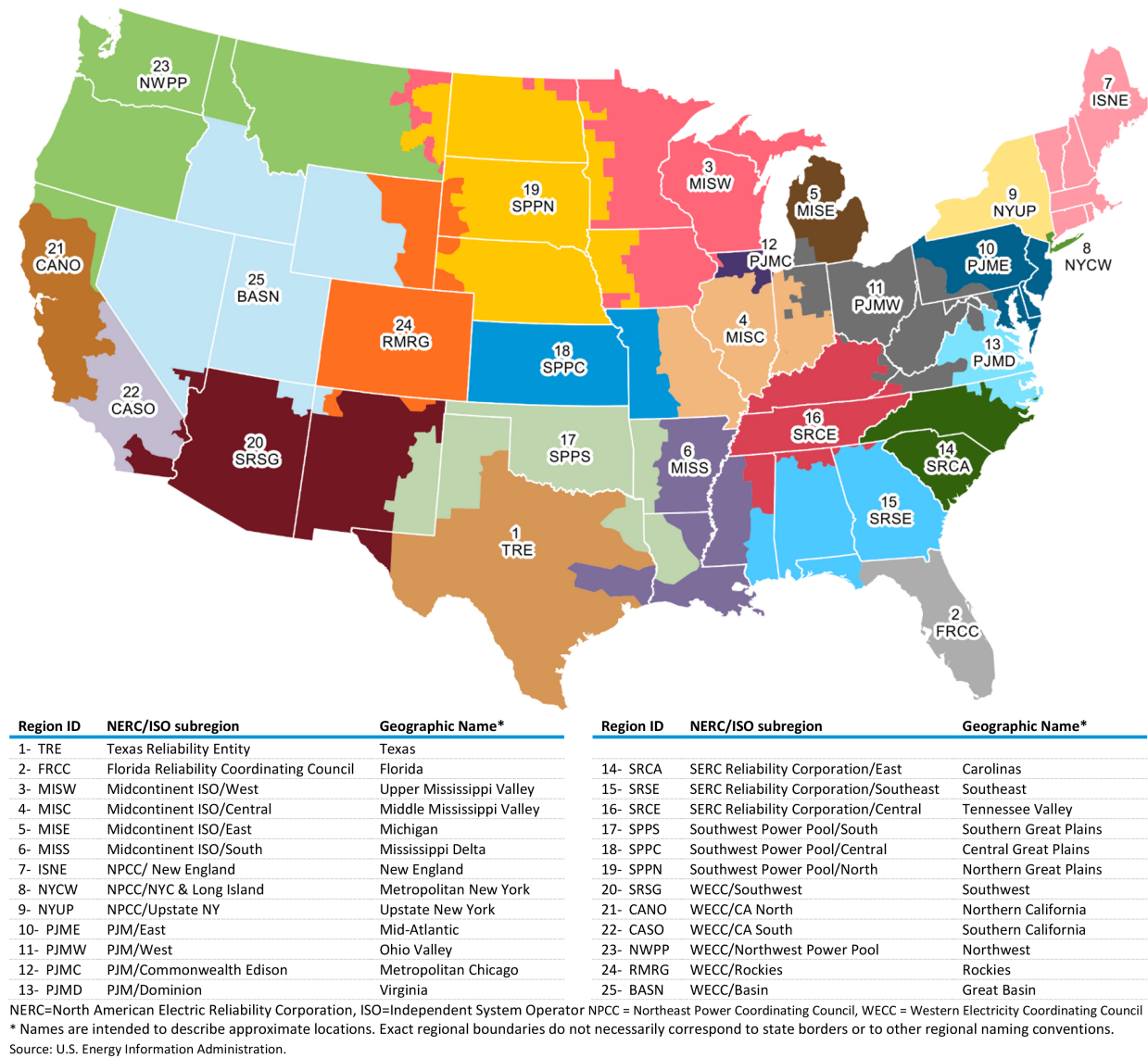
Fig. 11: Map of U.S. EIA Electricity Market Module (EMM) regions.
