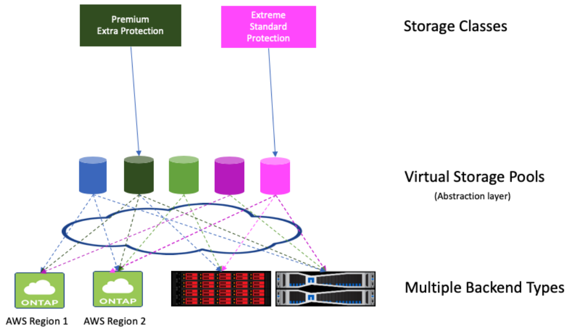
Fig. 1: Virtual Storage Pools
