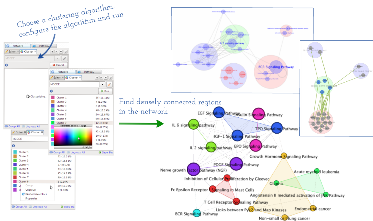
Fig. 5.1: Network Clustering
