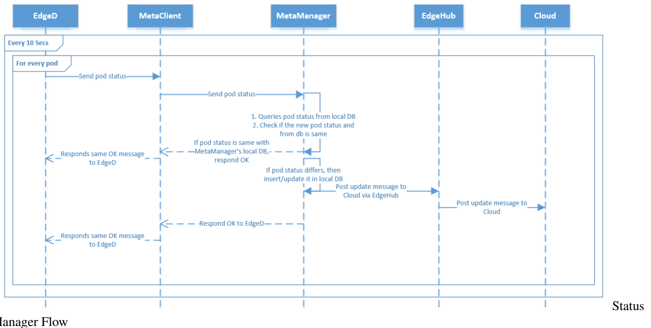
Fig 10: Status Manager Flow
