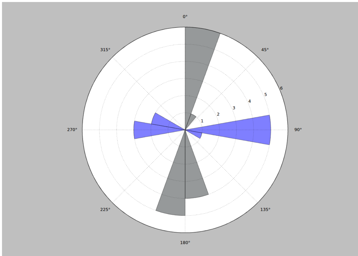
Fig. 1.30: This is how a plot appears in the rose diagram view.
