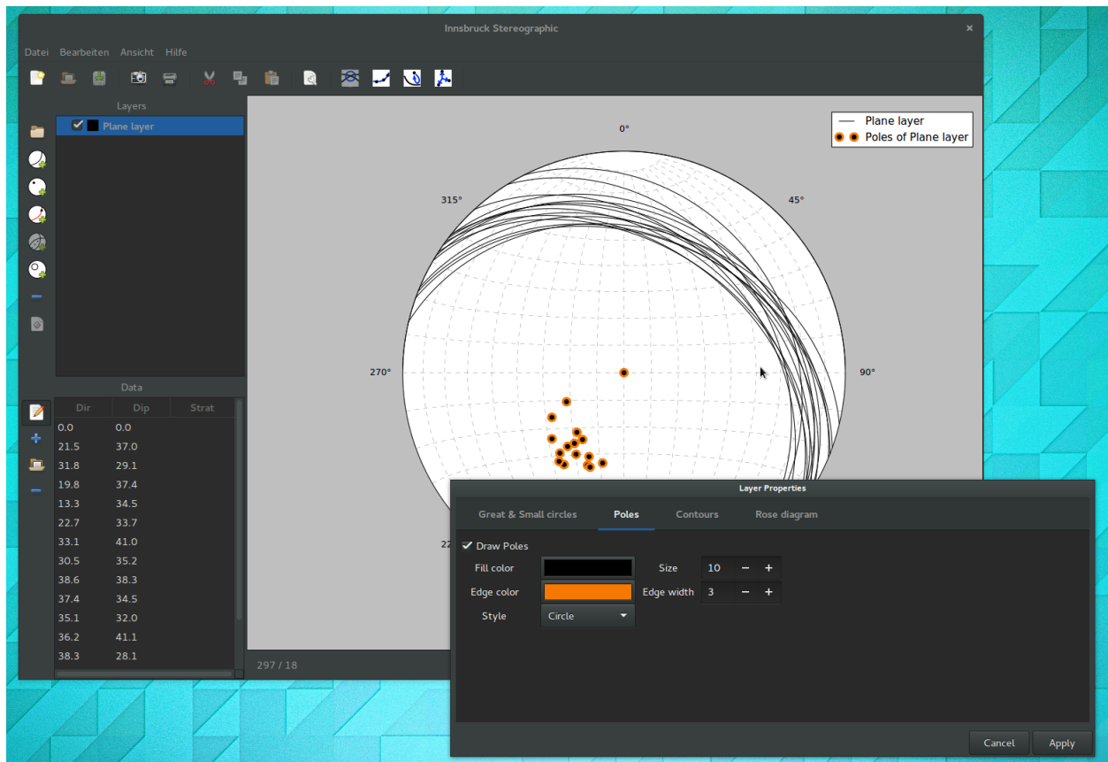
Fig. 1.22: Pole points have the same formatting options as linear-datasets have.
