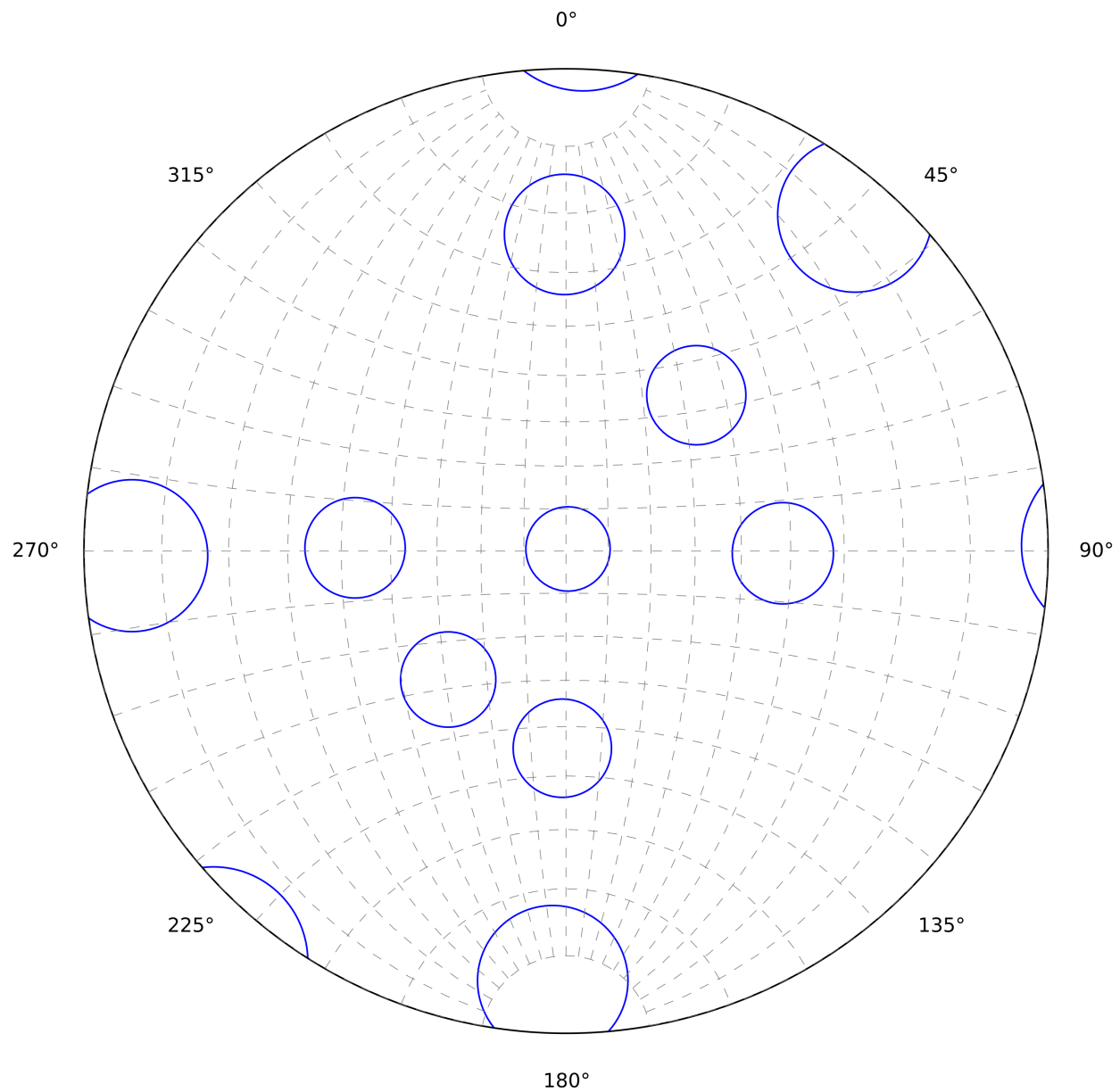
Fig. 1.18: Equal angle projections preserve angles, which can be seen by all small circles being perfect circles. Areas are not preserved and this is shown by the varying projected size of the small circles (all 10^\circ radius).
