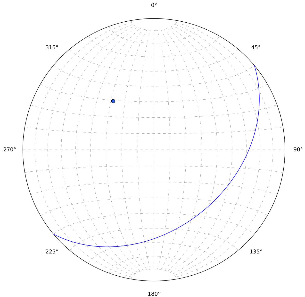
Fig. 1.19: A plane oriented 140/40 is shown here both as a great circle and a pole.
