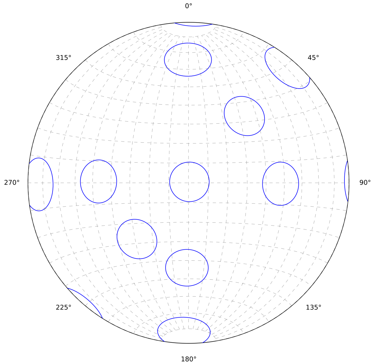
Fig. 1.17: Small circles (all 10^\circ radius) make it easier to see that area is preserved reasonably well across all orientations. Angles are slightly distorted and make the circles appear as ellipses.
