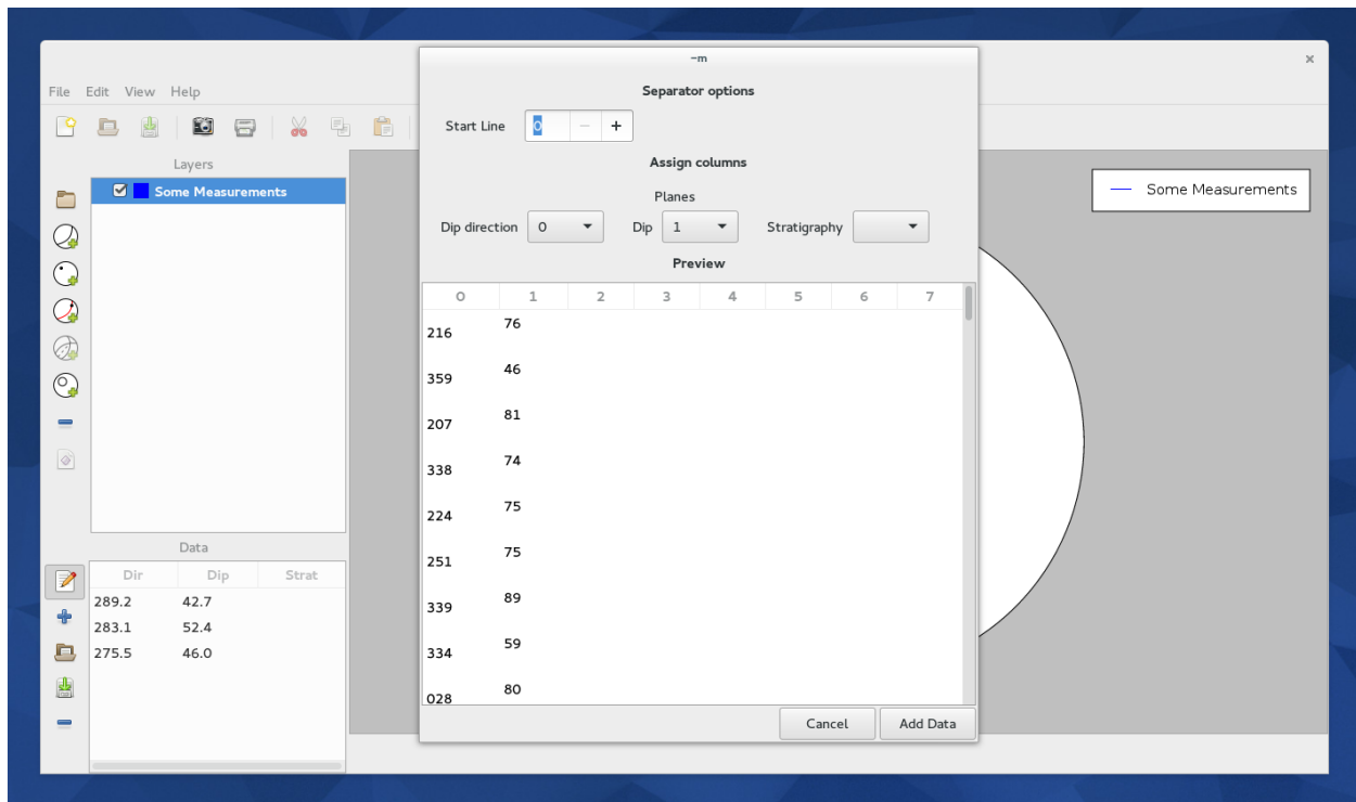
Fig. 1.32: The file parser dialog during a data-import. The columns in the data are assigned to the columns that Innsbruck Stereographic uses.
