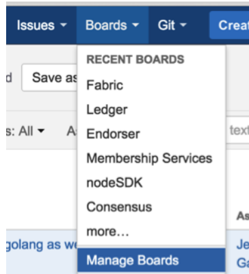
9.1: Jira boards
