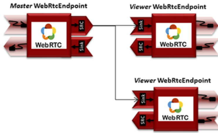
Fig. 22: One to many video call Media Pipeline
