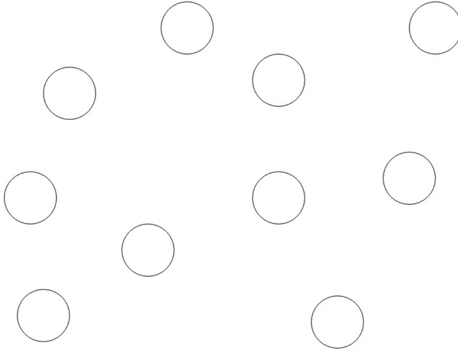
Fig. 1: Empty Network
