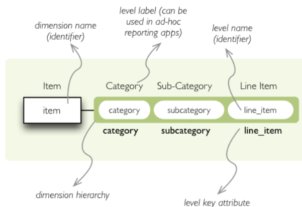
Fig. 6.4: Item dimension hierarchy.
