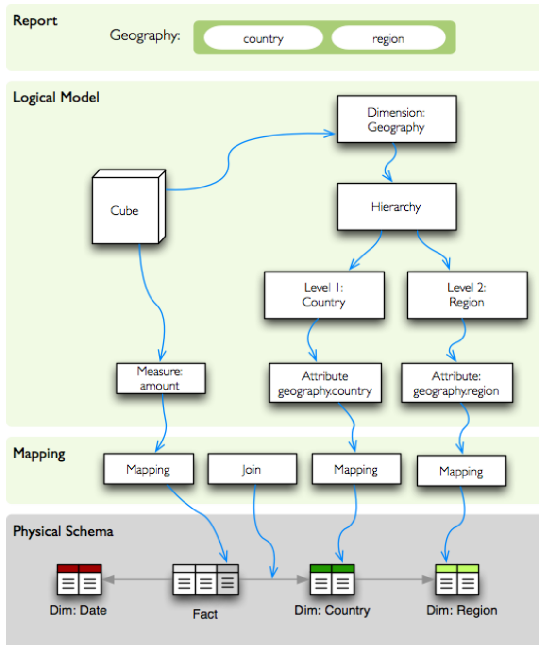
Fig. 2.1: Mapping from logical model to physical data.
