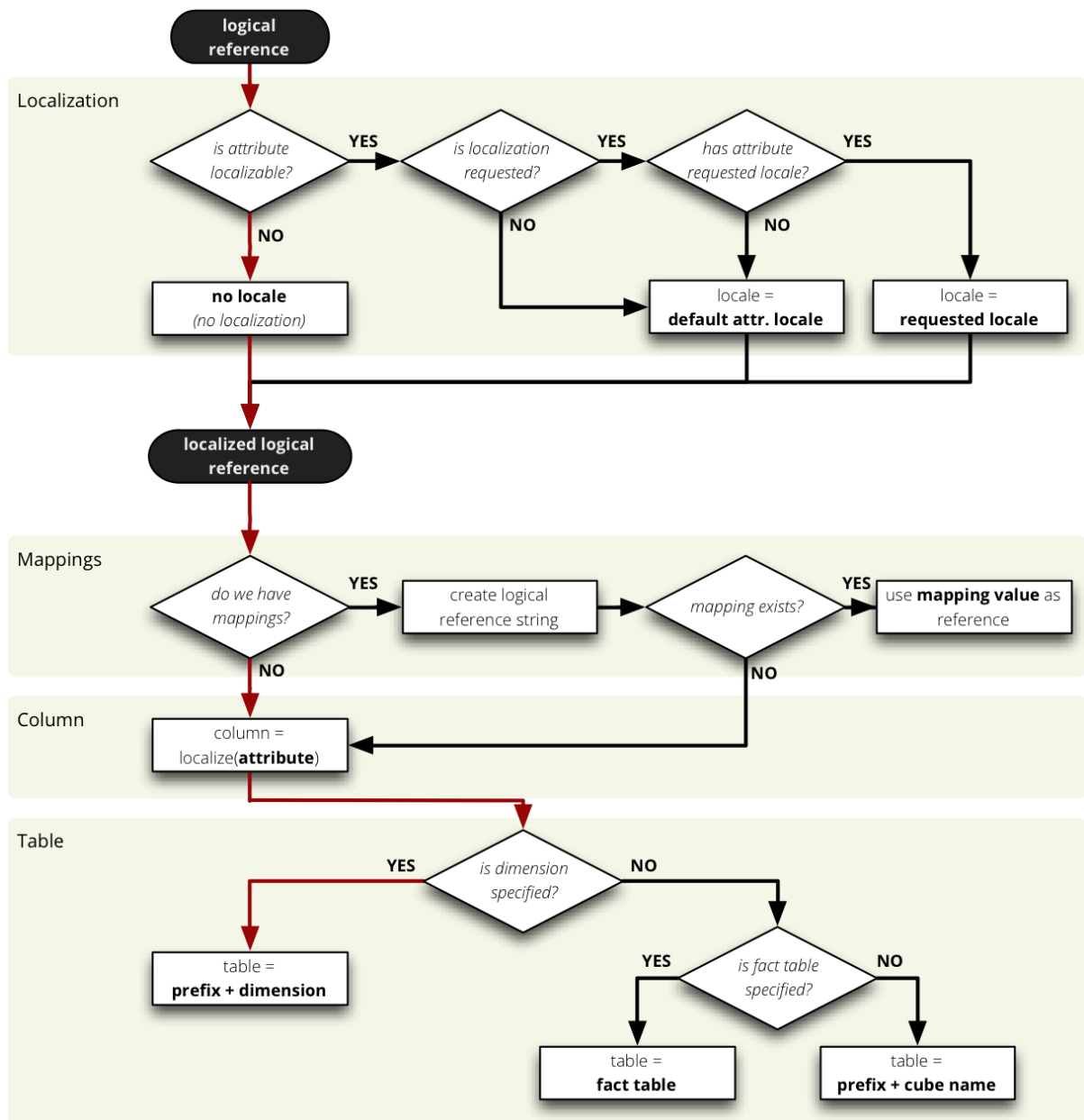
Figure 6.1: logical to physical attribute mapping
