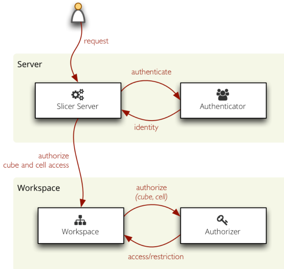
Figure 4.2: Overview of authorization and authentication process in Slicer
