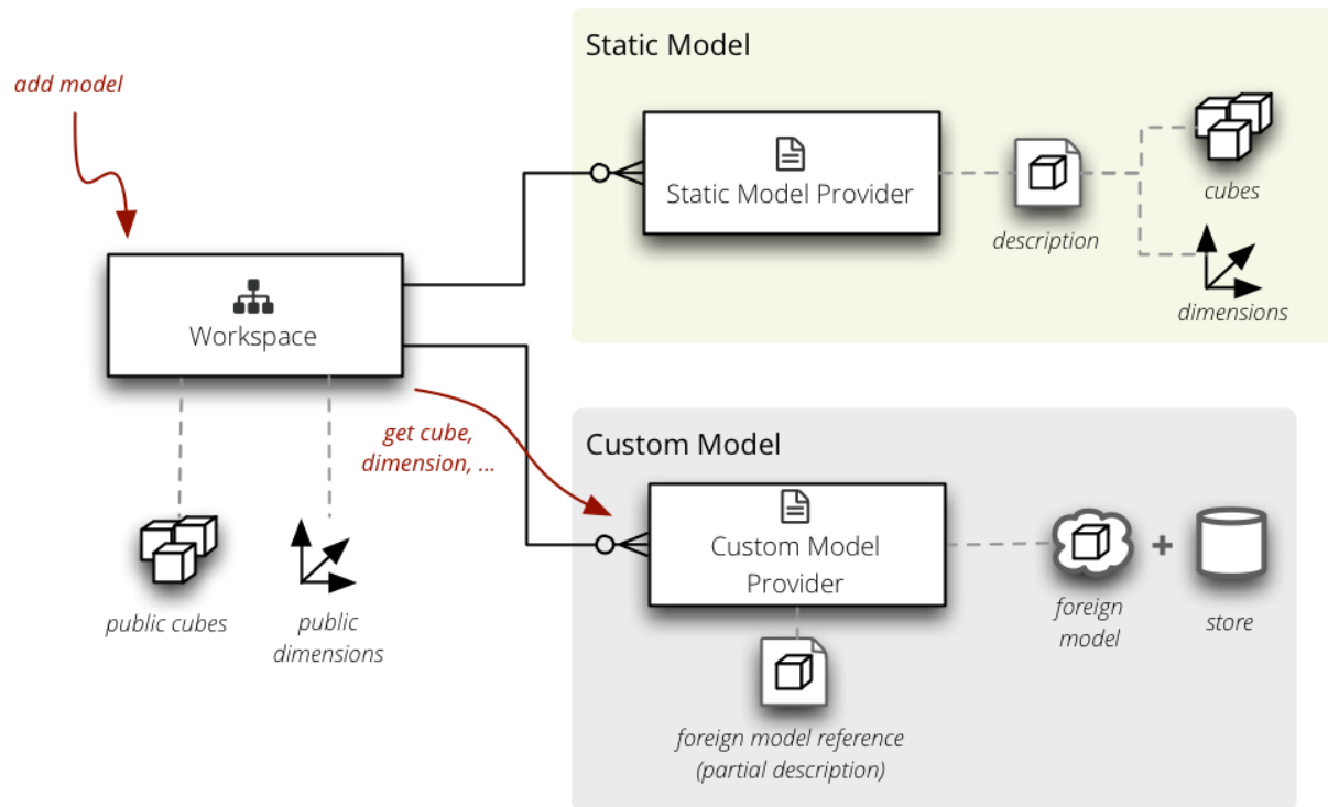
Figure 8.3: Context of Model Providers.
