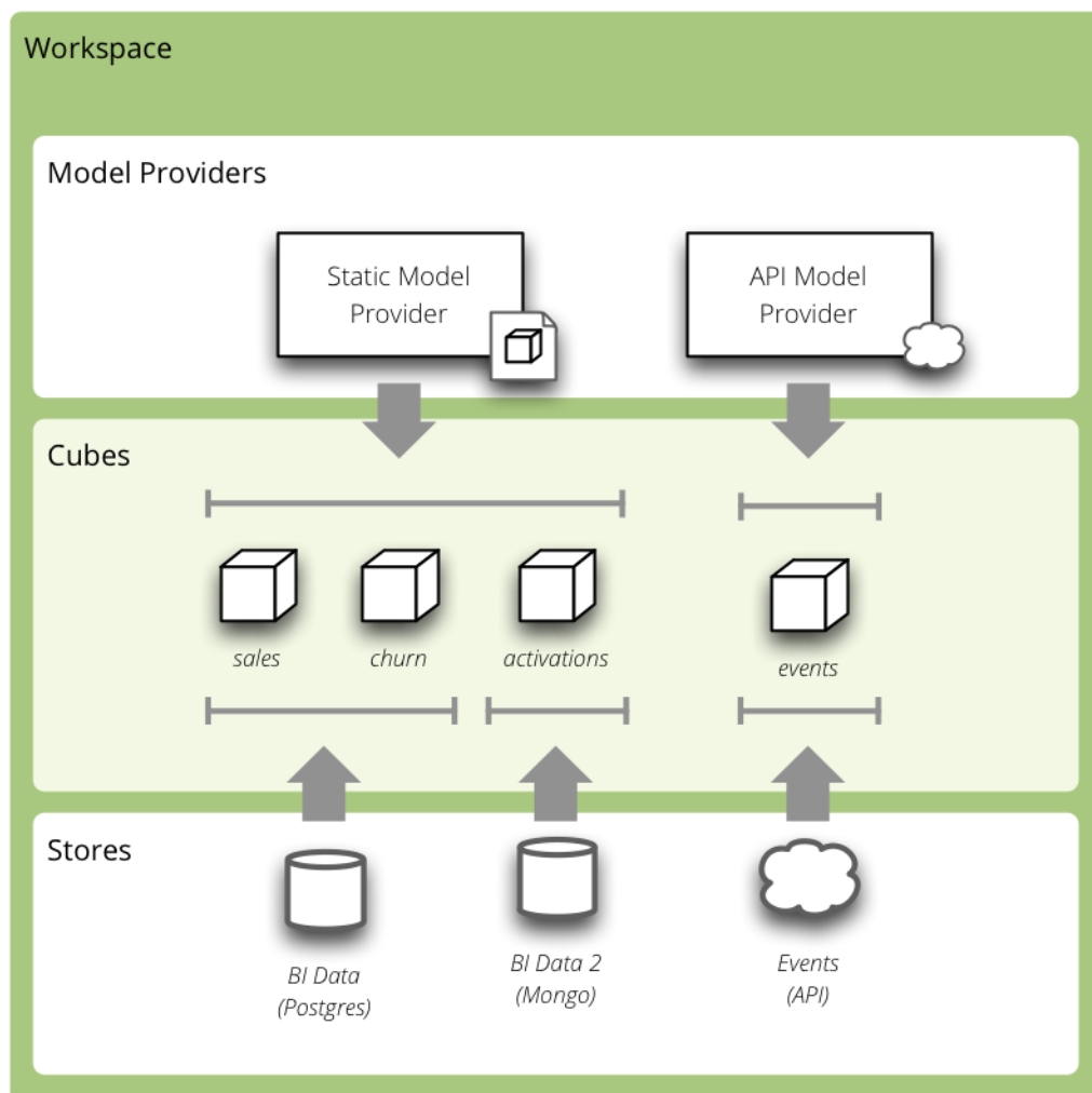
Figure 10.1: Analytical Workspace Overview
