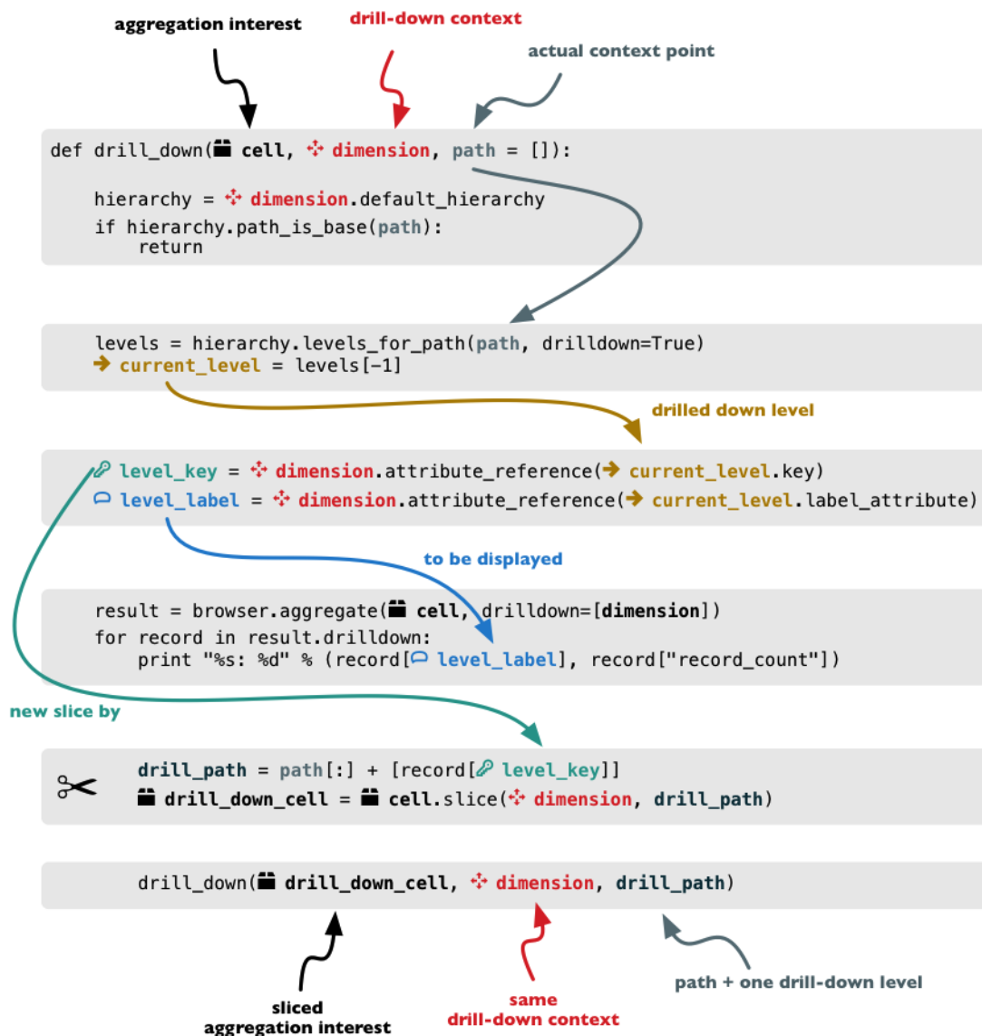
Figure 7.2: Recursive drill-down explained
