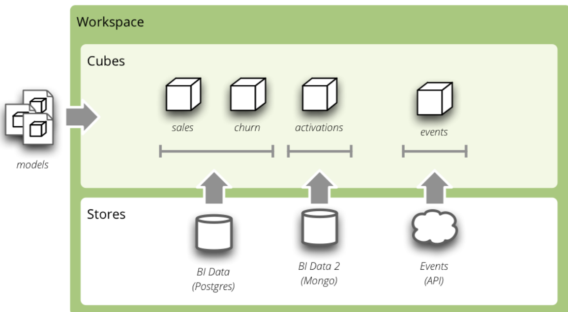
Figure 1.2: Analytical workspace and it's content
