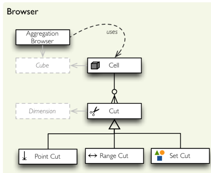
Figure 9.1: Browser package classes.
