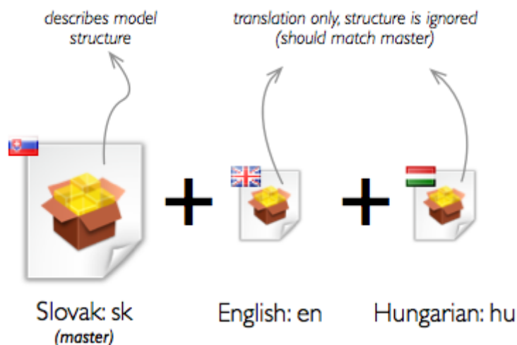
Figure 2.6: Localization master model and translation files.
