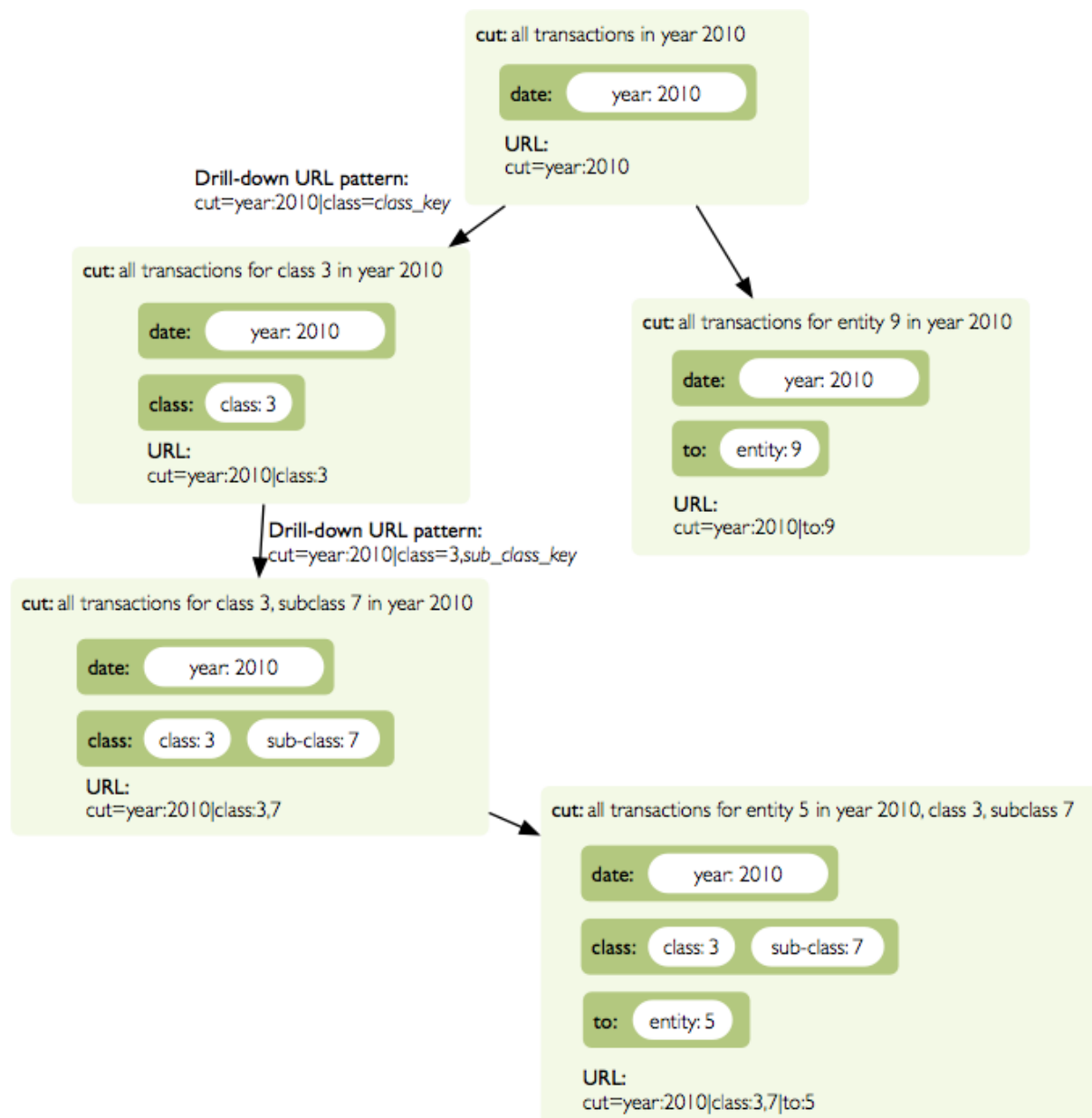
Figure 5.1: Example of how cuts in URL work and how they should be used in application view templates.
