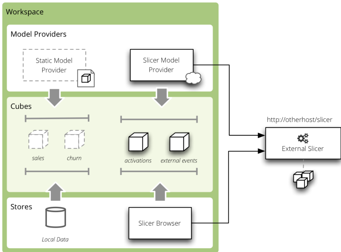
Figure 6.3: Slicer backend
