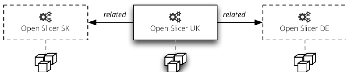
Figure 7.1: Related slicers.
