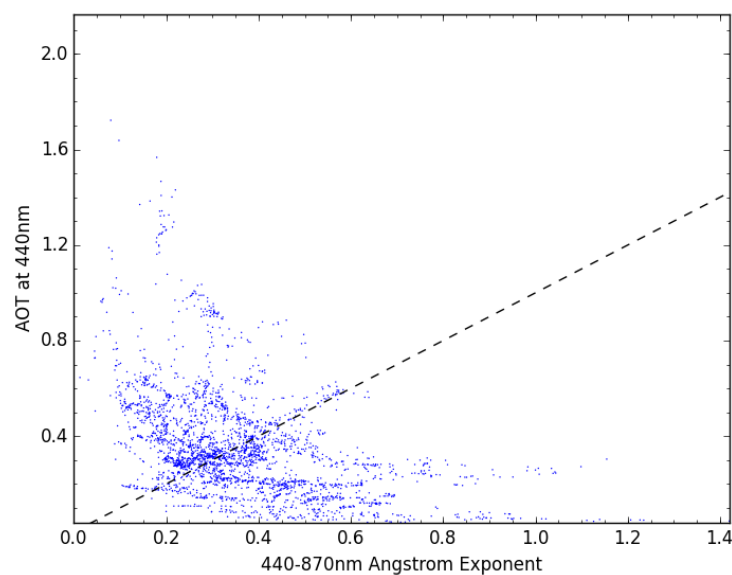
Fig. 7: Aeronet comparative scatter
