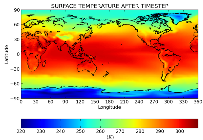
Fig. 1: Model output data
