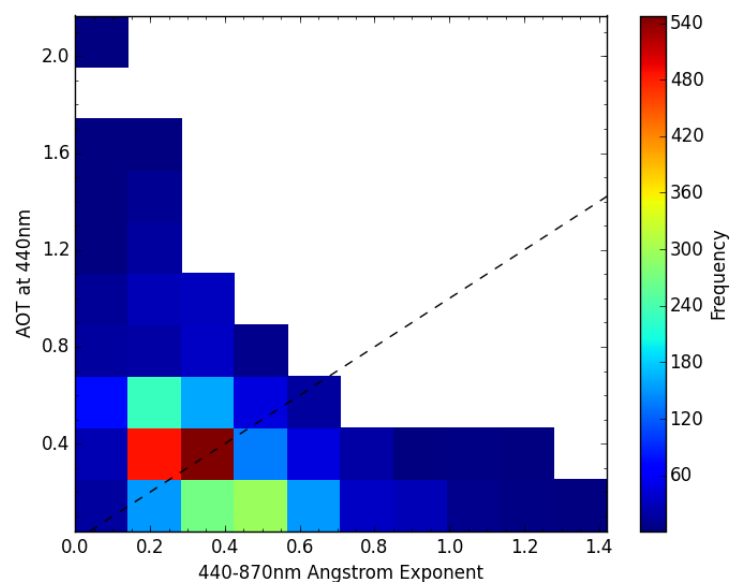
Fig. 8: Aeronet comparative histogram
