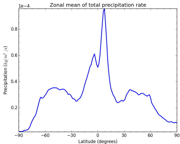
Fig. 2: Aggregated model data
