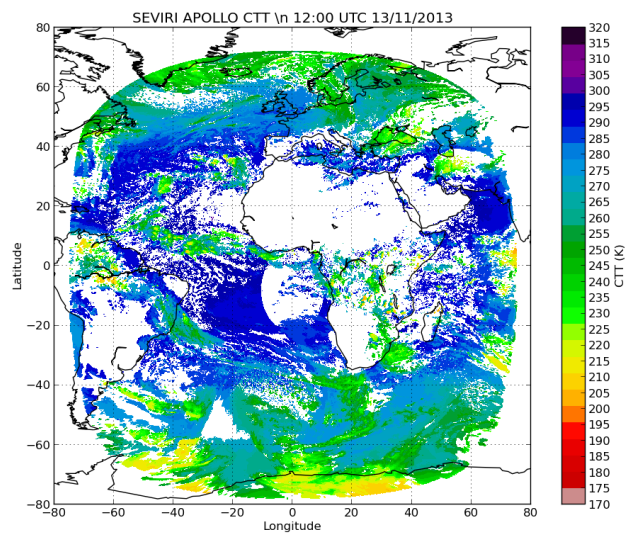
Fig. 5: Seviri Cloud top temperature
