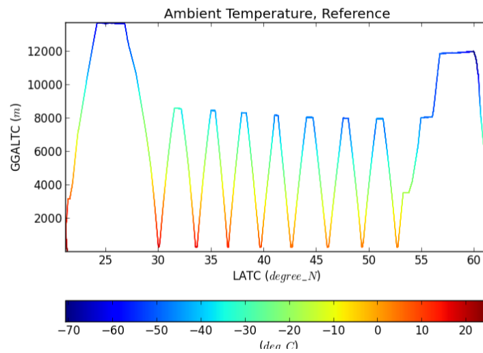
Fig. 13: NCAR-RAF ambient temperature
