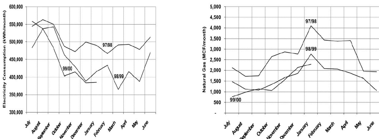
图 3: Figure 4-3. Natural Gas and Electricity Consumption at the Materials Research Institute Before and After Implementation of CCSM Measures
