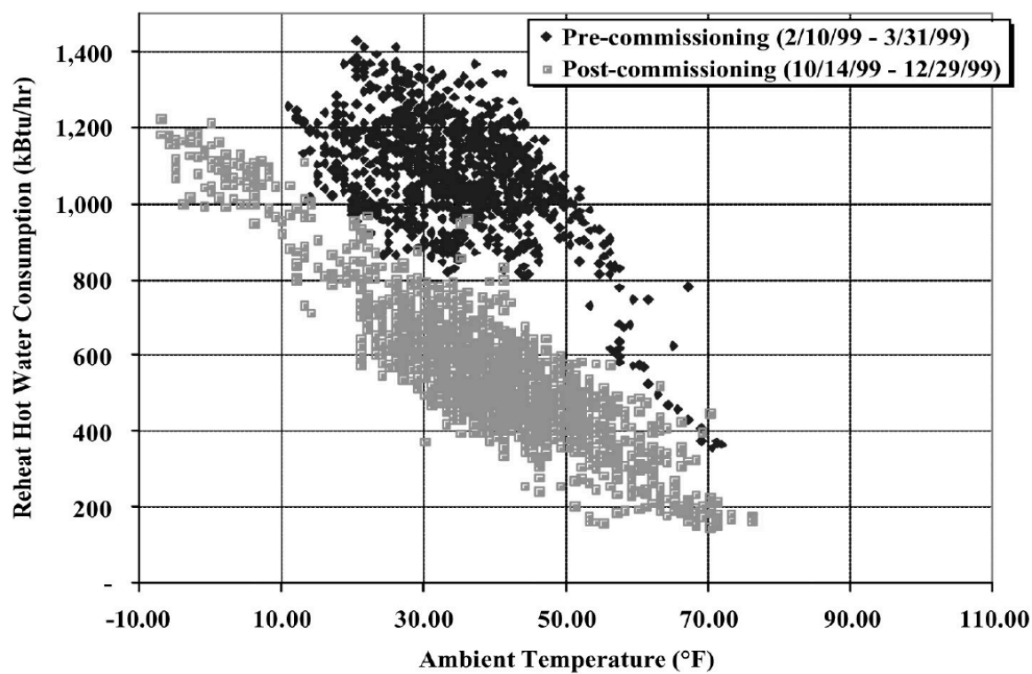
图 3: Figure 2-3. Hourly Reheat Energy at Riverside North (15-minute data)
