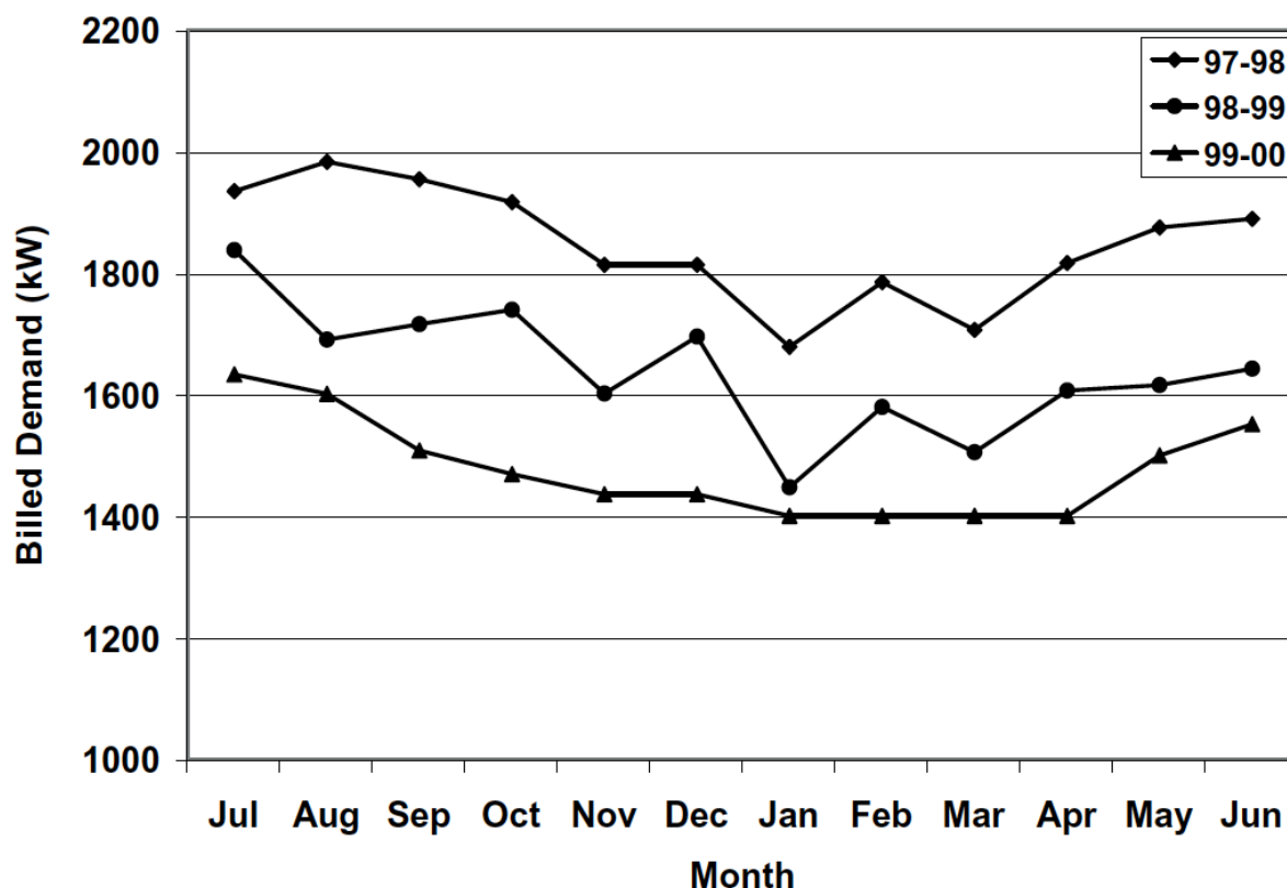
图 11: Figure 8-11. Comparison of Billed Electrical Demand Before and After Commissioning
