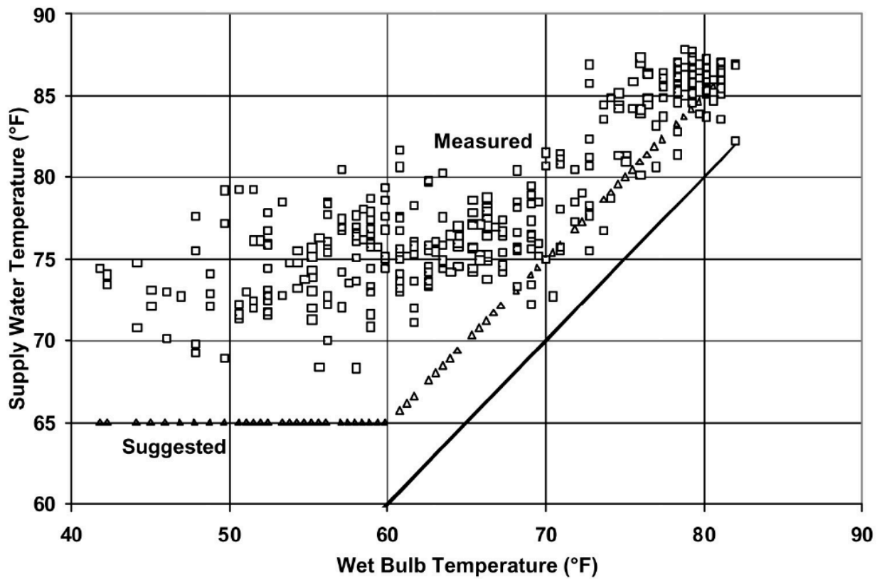
图 2: Figure 6-2. Measured Condenser Supply Water Temperature at the UTMB Chiller Plant as a Function of Ambient Wet Bulb Temperature
