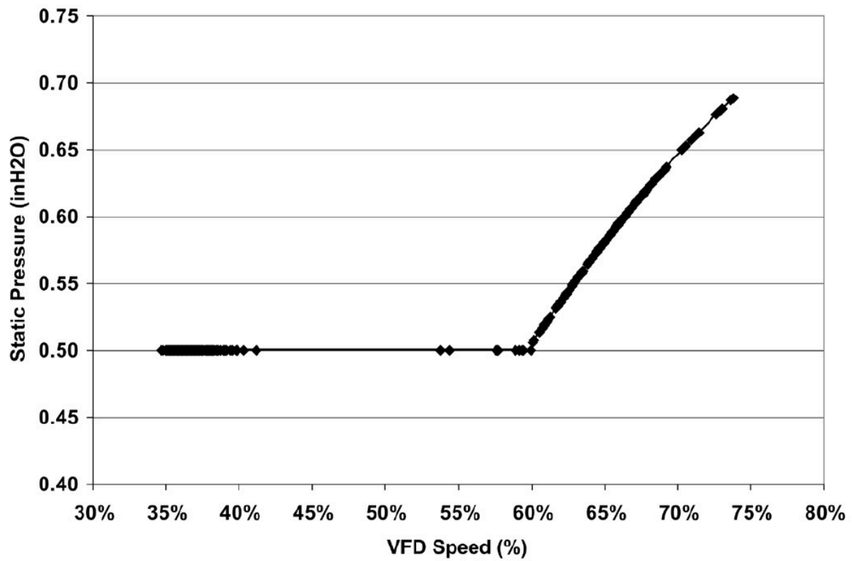
图 6: Figure 4-6. Optimal Static Pressure Reset Schedule and Measured Static Pressure Versus the VFD Speed for AHU-P2 at the CSF Building, M.D. Anderson Cancer Center, Houston, Texas
