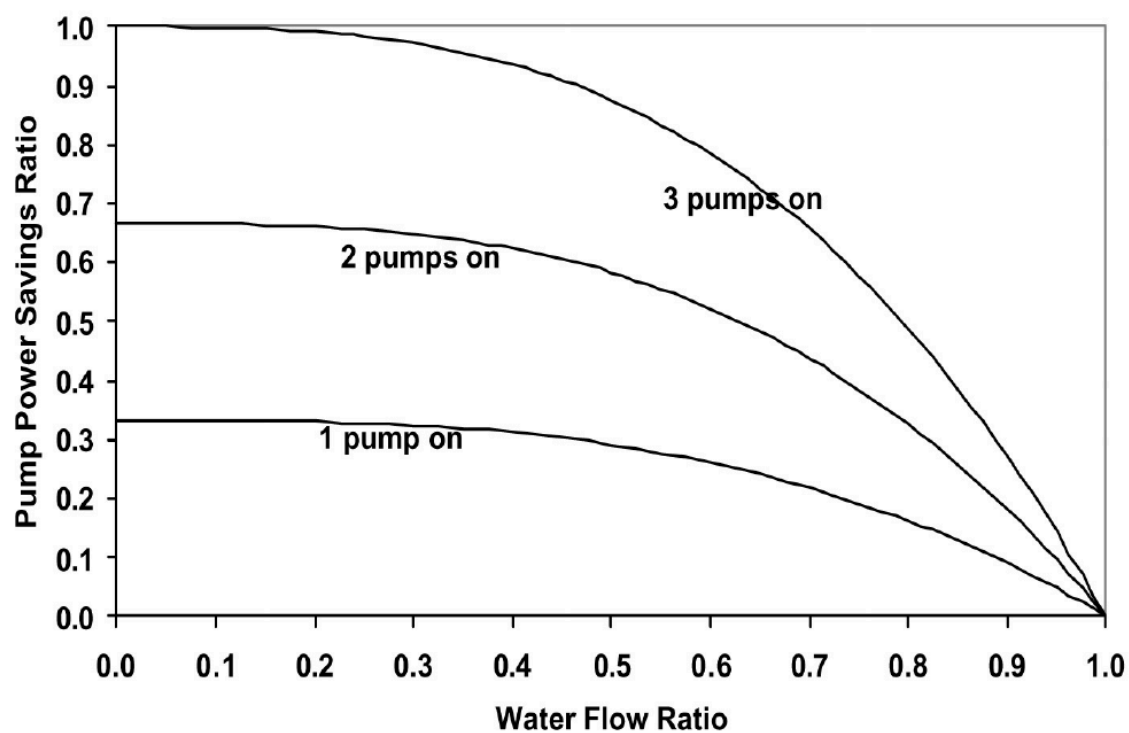
图 5: Figure 6-5. Potential Primary Pump Power Savings Ratio Versus Chilled Water Flow Ratio through Each Chiller
