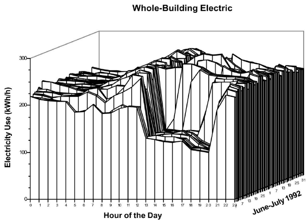
图 4: Figure 8-4. Hourly Electricity Consumption for the Hospital in Monahans, Texas, for June and July, 1993
