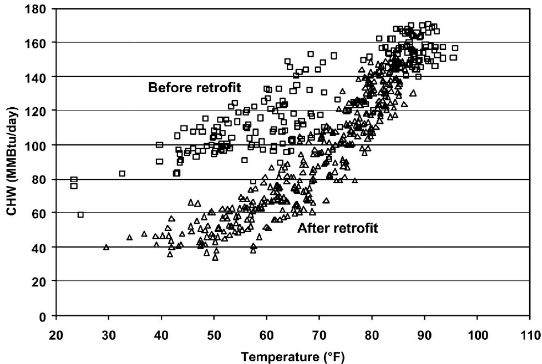
图 3: Figure A-3. ZEC Daily Chilled Water Consumption in 1990 Before the Retrofit and in 1994 After the Retrofit
