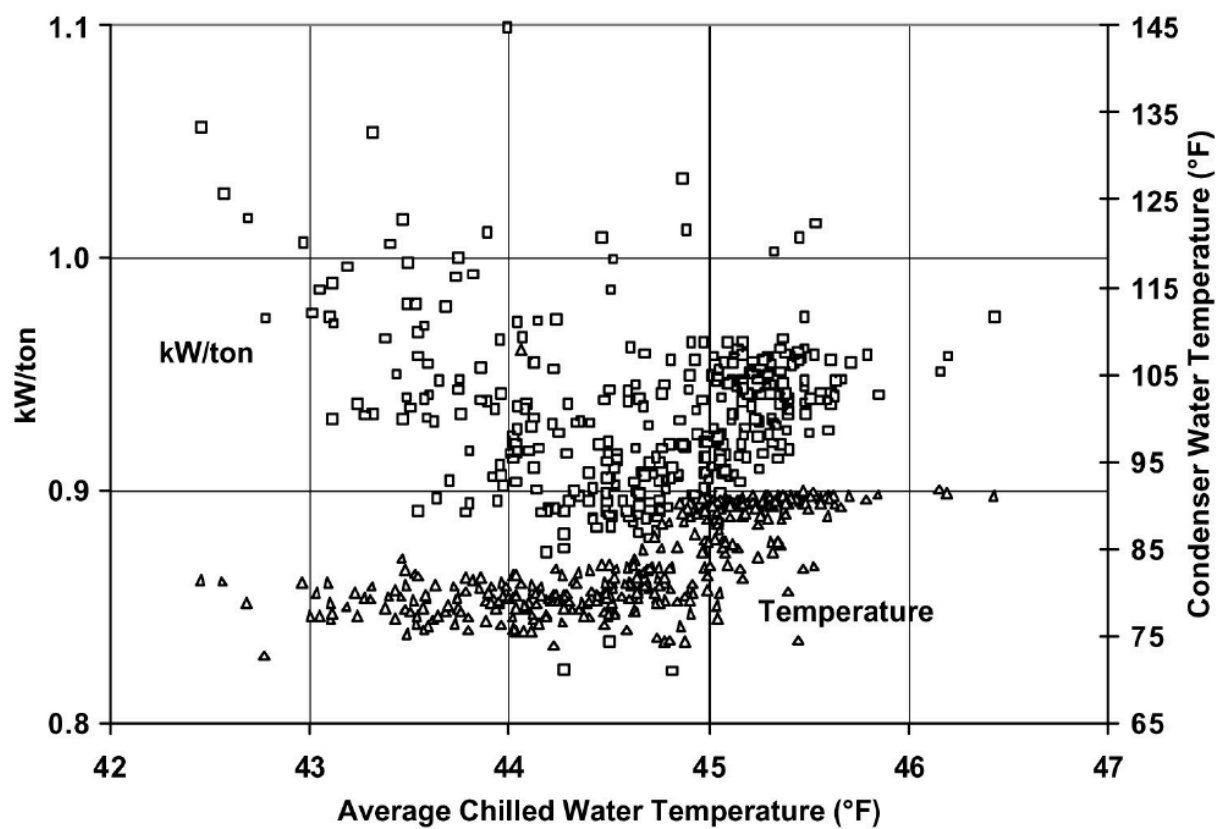
图 1: Figure 6-1. Measured Chiller Plant Efficiency and Condenser Water Temperature Plotted as Functions of Average Chilled Water Temperature
