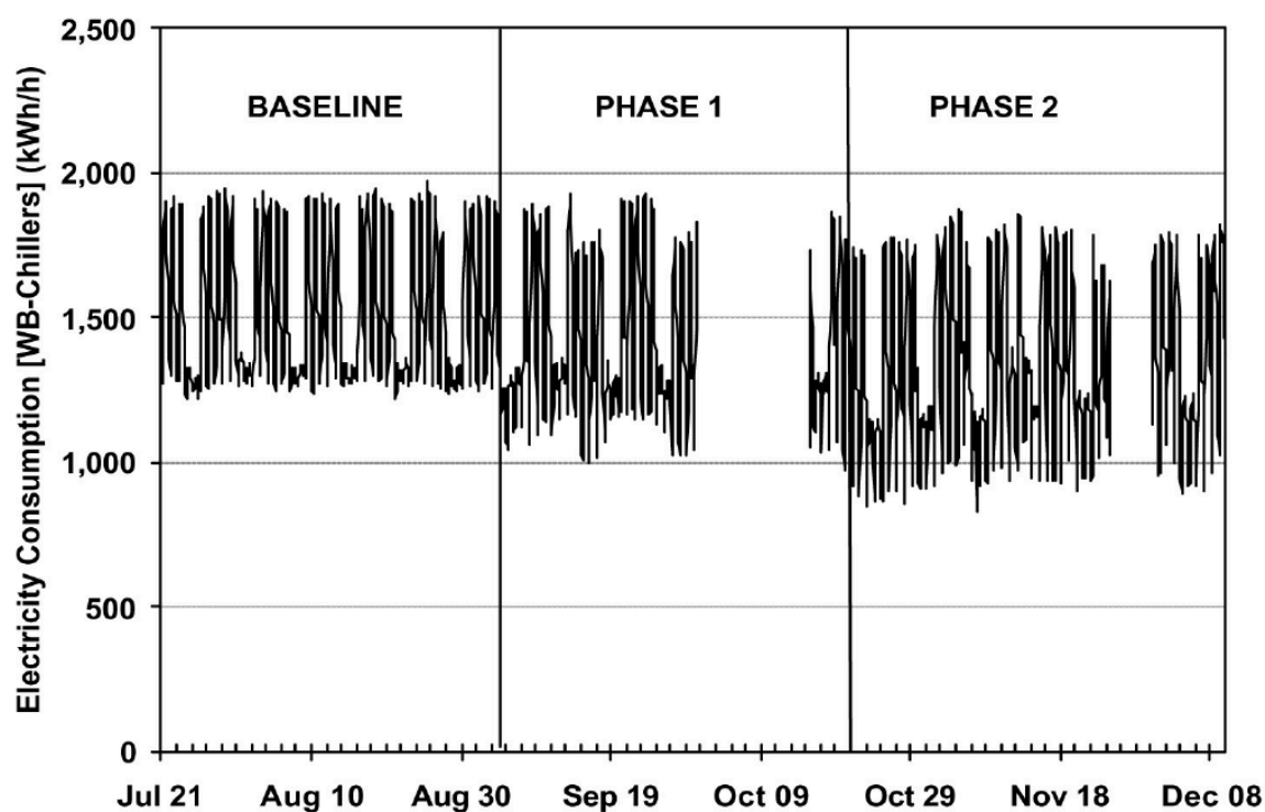
图 2: Figure 3-2. Hourly Whole Building Electricity Consumption at the Stephen F. Austin (SFA) Building Before and After Night Shut Down of AHUs Was Initiated
