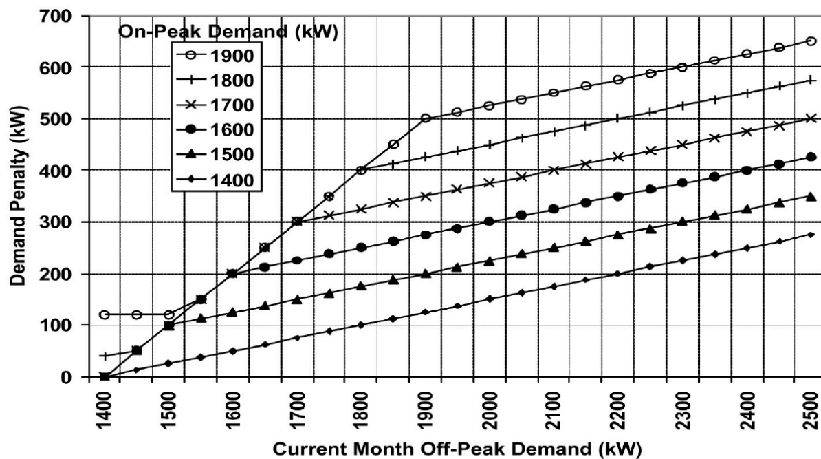
图 8: Figure 8-8. Demand Penalties Under Different Current Month Demand Values When On-Peak Demand Has Been Set at Different Levels
