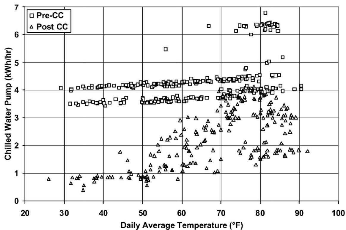
图 6: Figure 8-6. Pumping Power at the Monahans, Texas, Hospital Before and After CCSM Measures Were Implemented
