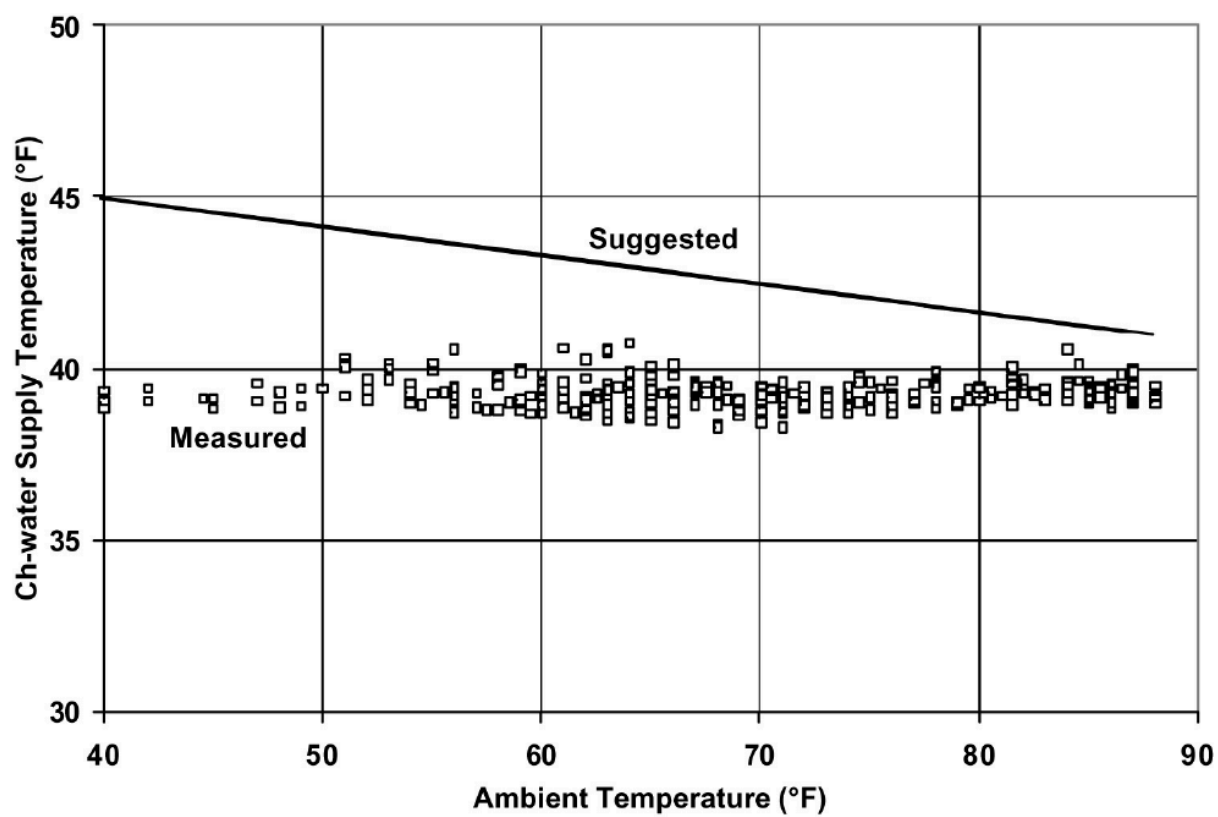
图 3: Figure 6-3. Measured And Suggested Chilled Water Supply Temperature at UTMB
