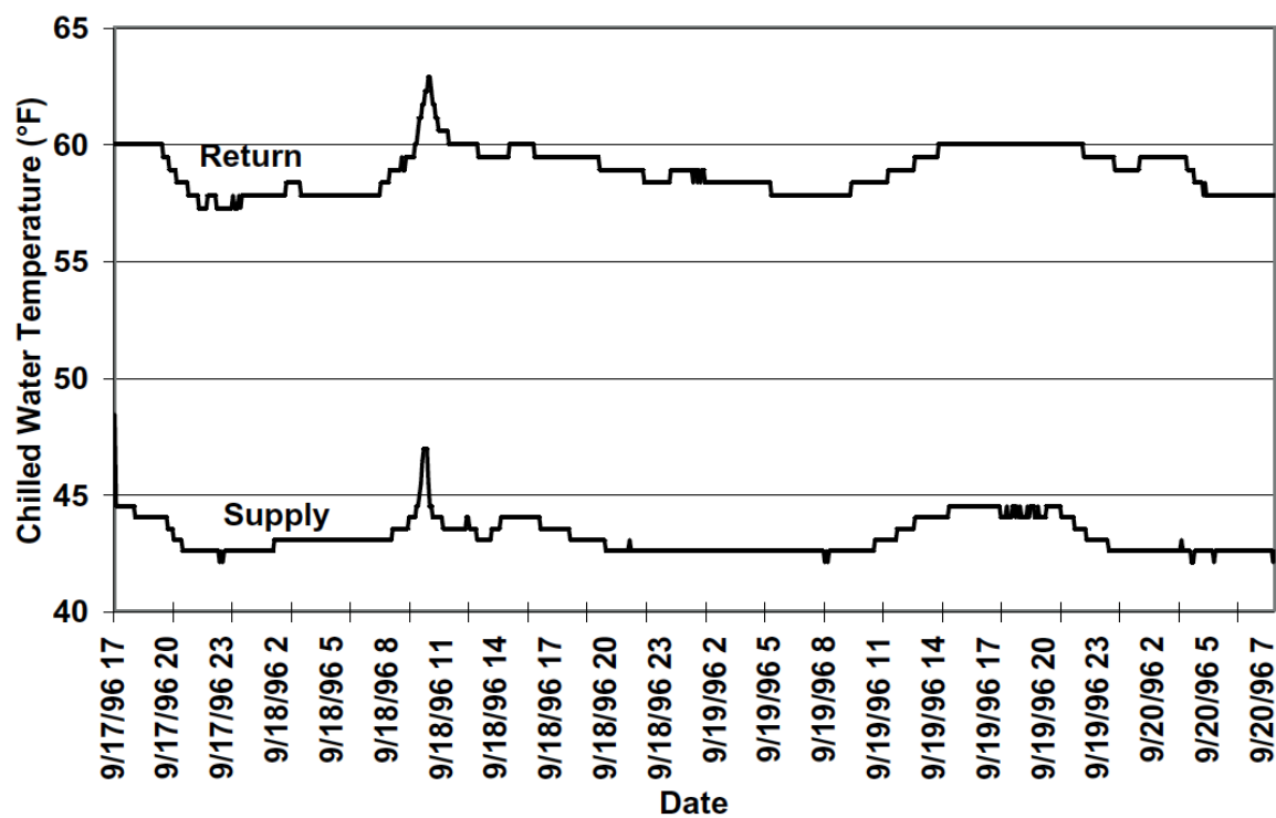
图 4: Figure 6-4. Measured Chilled Water Supply and Return Water Temperature After Building Commissioning (the building differential temperature was less than 10°F before commissioning)
