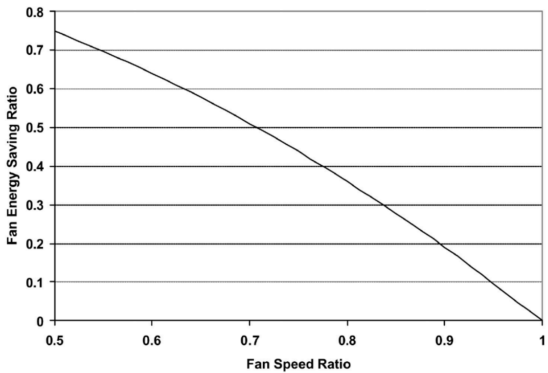
图 4: Figure 3-4. Potential Fan Energy Savings Using Fan Speed Limiting
