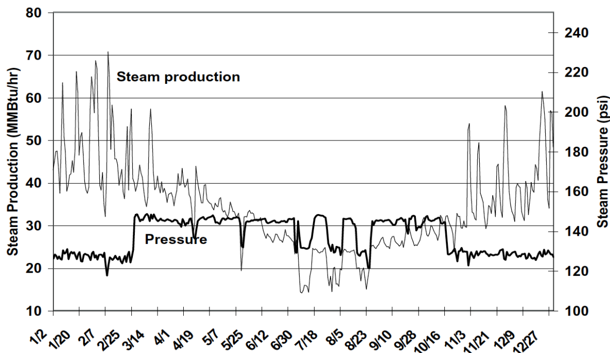
图 3: Figure 7-3. Variation of Steam Consumption and Boiler Pressure with Time at UTMB
