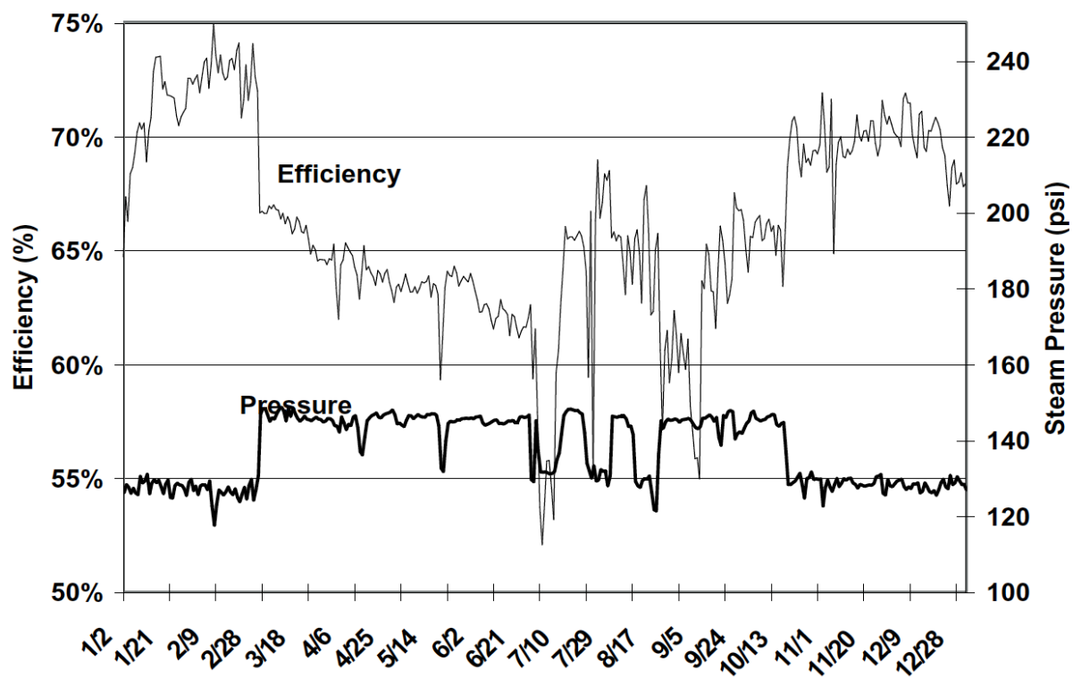
图 2: Figure 7-2. Boiler Efficiency and Steam Pressure at the UTMB Galveston Boiler Plant
