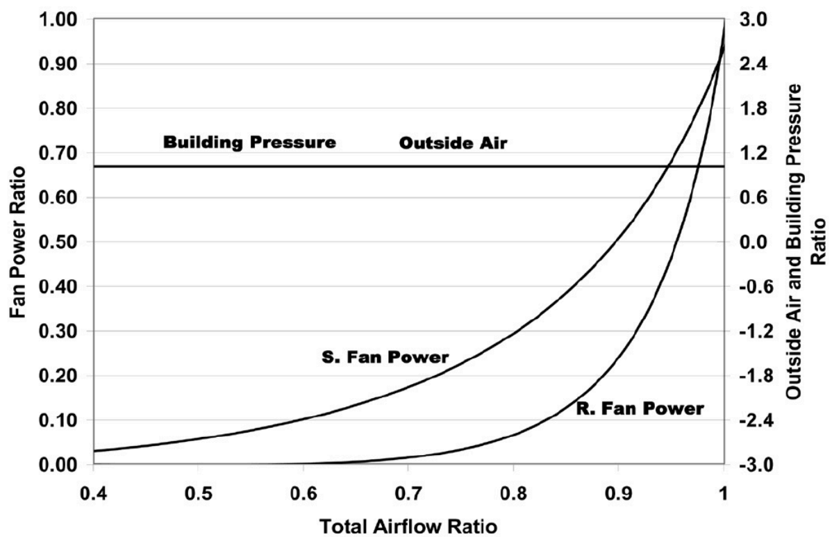
图 23: Figure 4-23. Simulated Building Pressure, Outside Air Intake and Fan Power Using VSDVT Control
