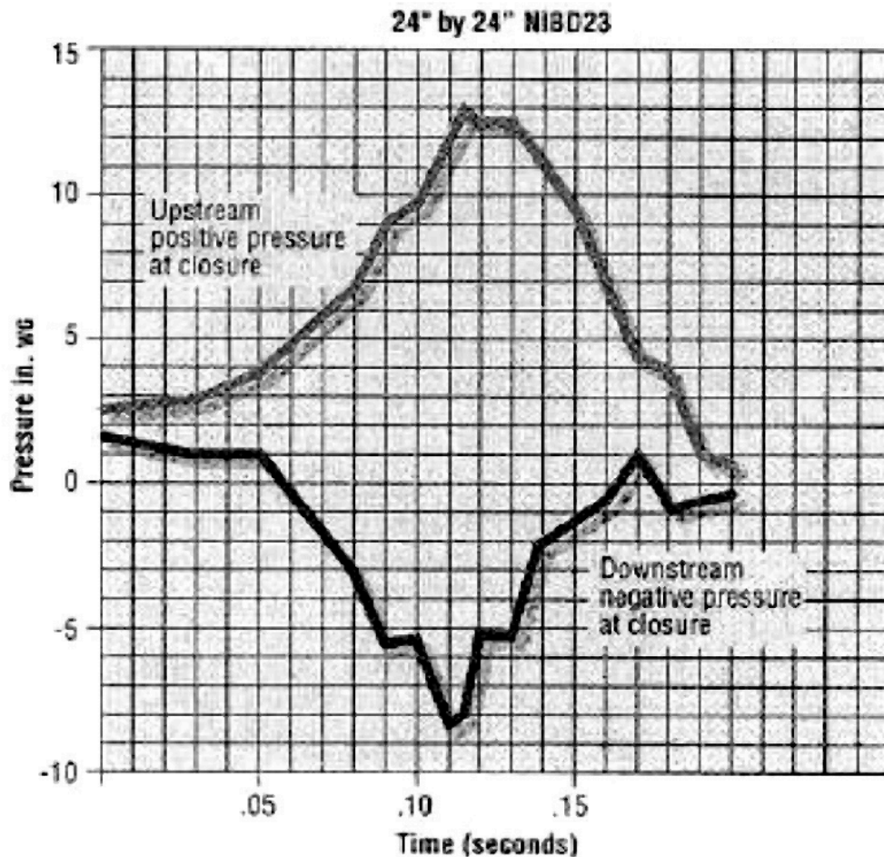
图 15: Figure 4-15. Static Pressure Versus Time Upstream and Downstream of a Fire Damper When Suddenly Closed
