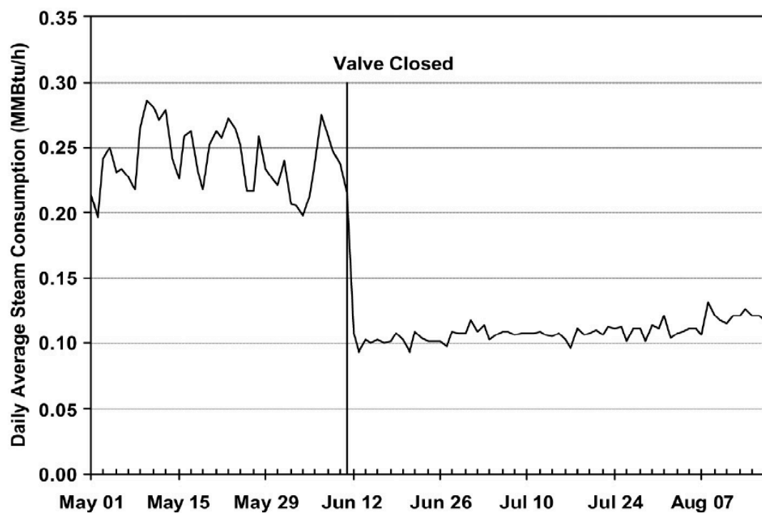
图 1: Figure 3-1 Comparison of Measured Daily Average Steam Consumption Before and After Manually Shutting Off Heating Coil Valves in the Business Administration Building at University of Texas at Austin
