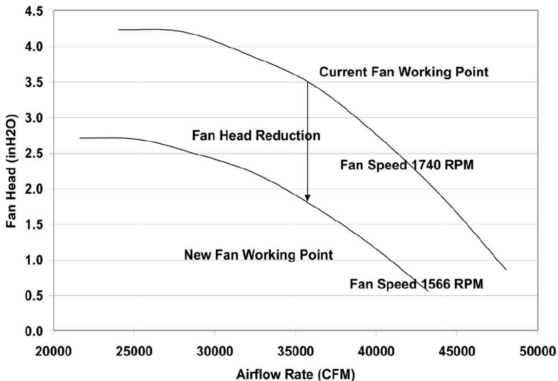
图 1: Figure 4-1. Determining New Fan Speed Using Measured Fan Head Reduction and Fan Performance Curve
