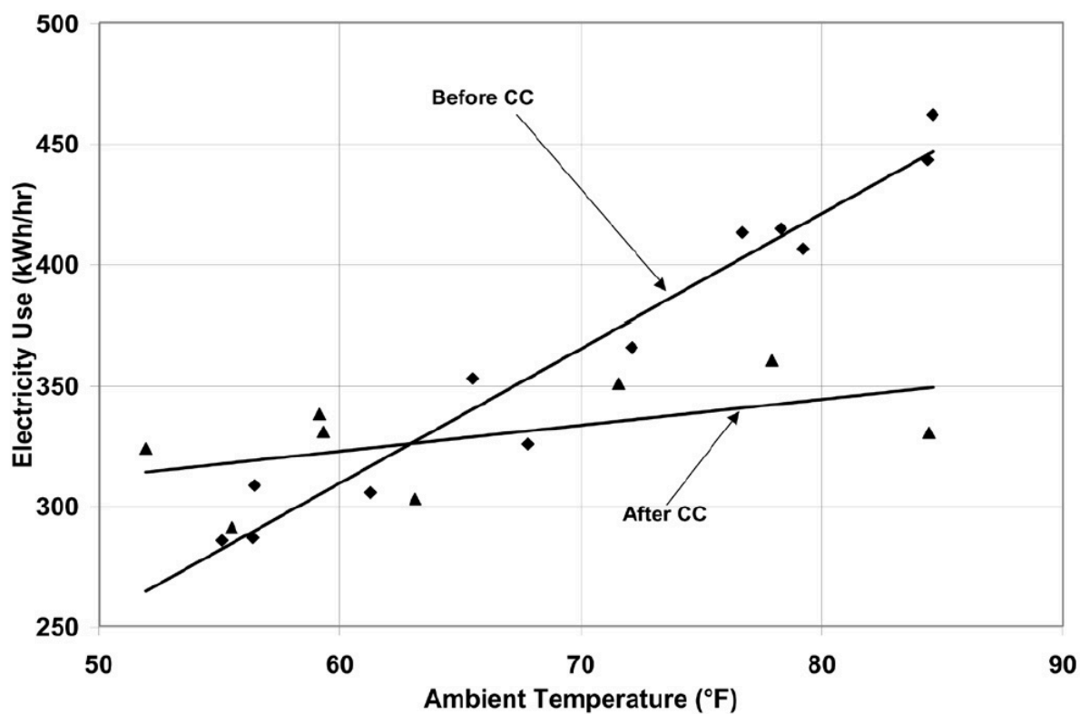
图 4: Figure 4-4. Measured Monthly Average Hourly Whole Building Electricity Consumption Versus the Monthly Average Ambient Temperature
