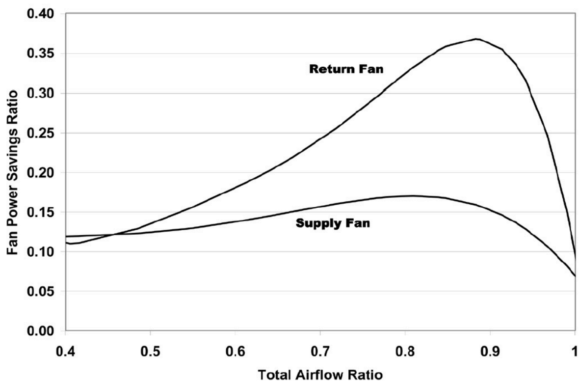
图 24: Figure 4-24. Potential Fan Power Savings of the VSDVT Method
