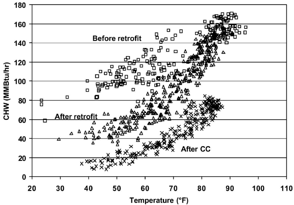
图 6: Figure A-6. ZEC Daily Chilled Water Consumption for 1990 Before the Retrofit, 1994 After the Retrofit and 1997 After CCSM
