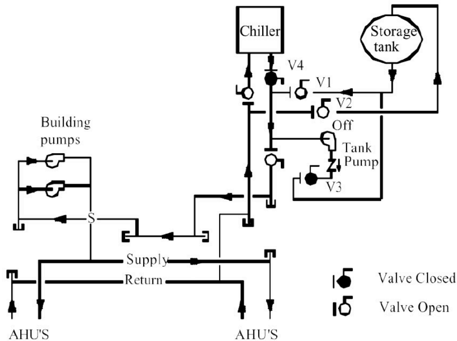
图 3: Figure 8-3. Waterside Schematic of the Chiller/Thermal Storage System at the Hospital in Monahans, Texas
