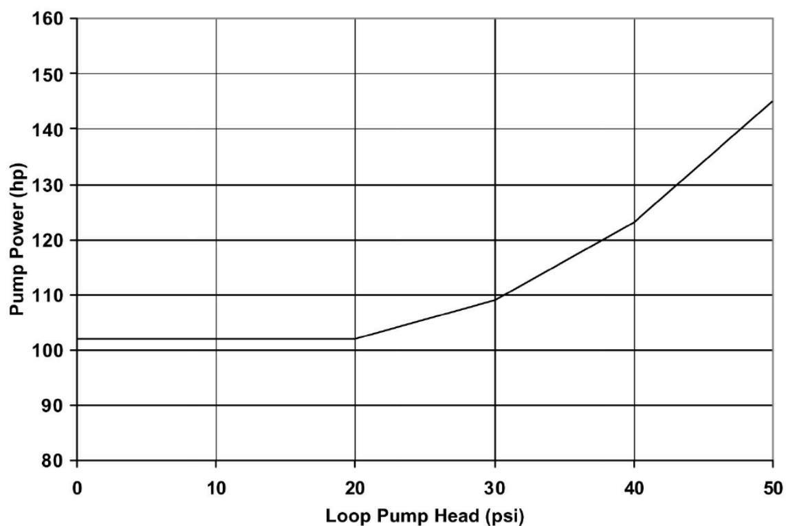
图 7: Figure 5-7. Pumping Power as a Function of Loop Pump Head for the System Considered in the Example
