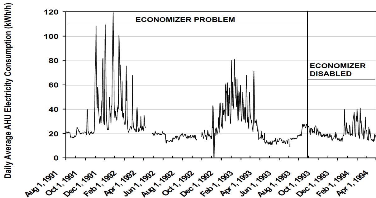
图 8: Figure 4-8. Measured Hourly Fan Power for the Nursing Building in Austin, Texas
