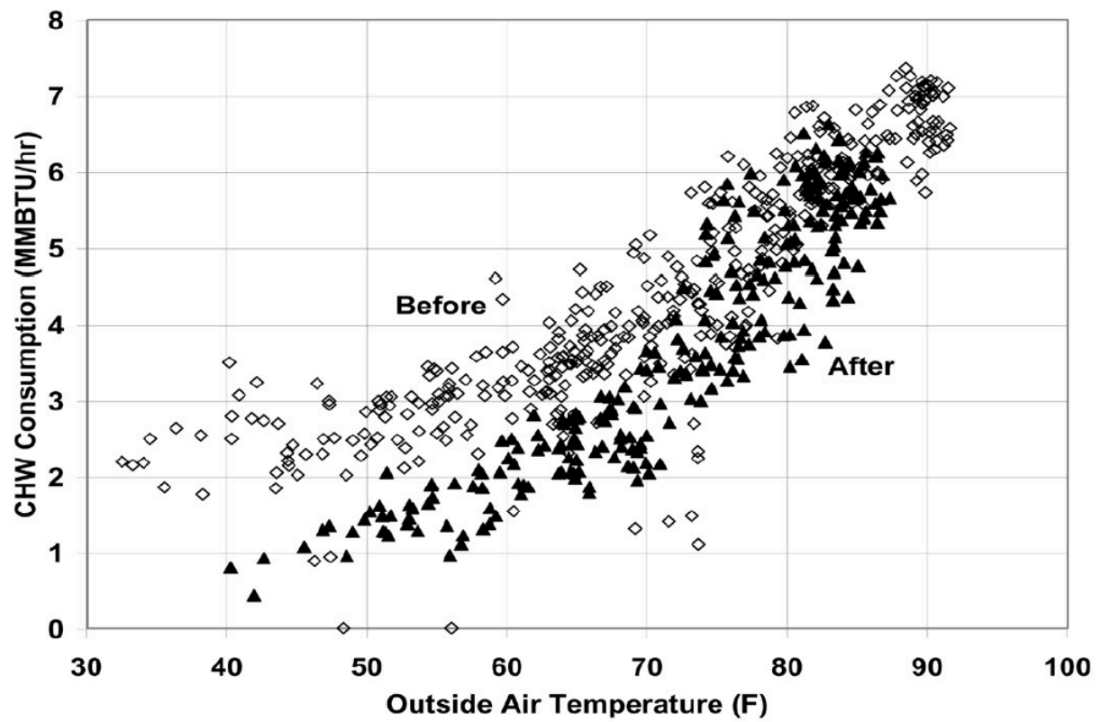
图 7: Figure 4-7. Comparison of Measured Daily Average Chilled Water Consumption Before and After Implementation of the Optimal Hot and Cold Deck Temperature Reset Schedules
