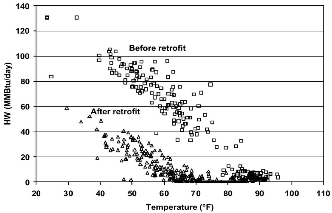
图 4: Figure A-4. ZEC Daily Hot Water Consumption in 1990 Before the Retrofit and in 1994 After the Retrofit
