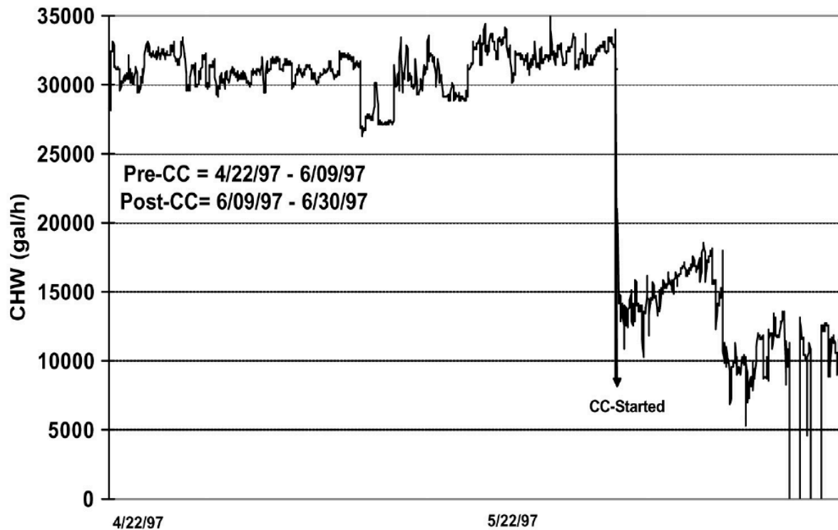
图 2: Figure 5-2. Comparison of Measured Chilled Water Flow Under Both Initial and Optimal Differential Pressure Reset Schedules
