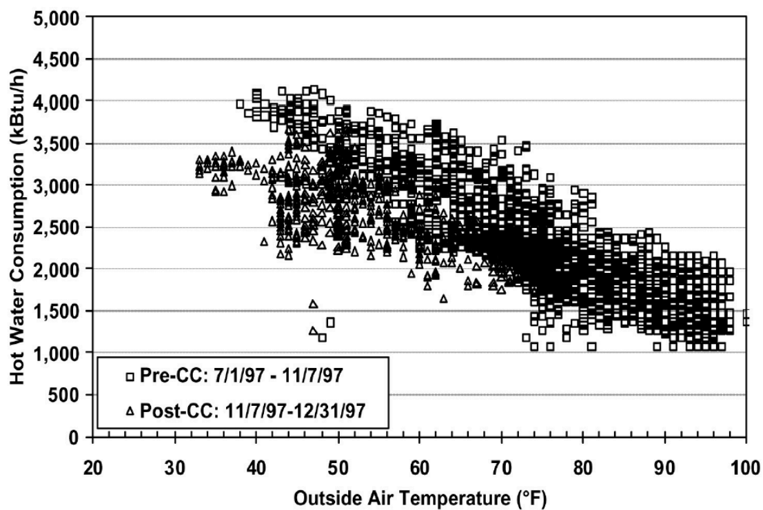
图 14: Figure 4-14. Comparison of Hot Water Energy Consumption Before and After Implementation of CCSM Measures
