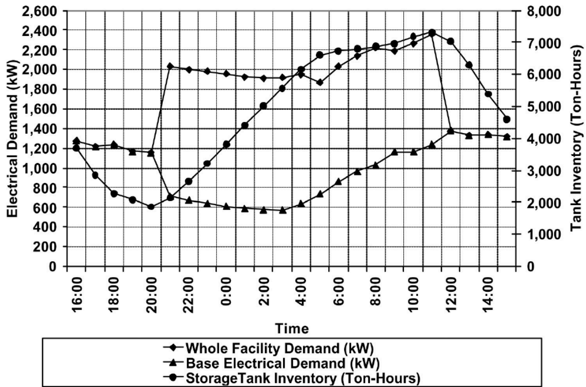
图 9: Figure 8-9. Typical On-Peak Months Whole Facility Demand, Base Electrical Demand and Storage Tank Inventory Profiles
