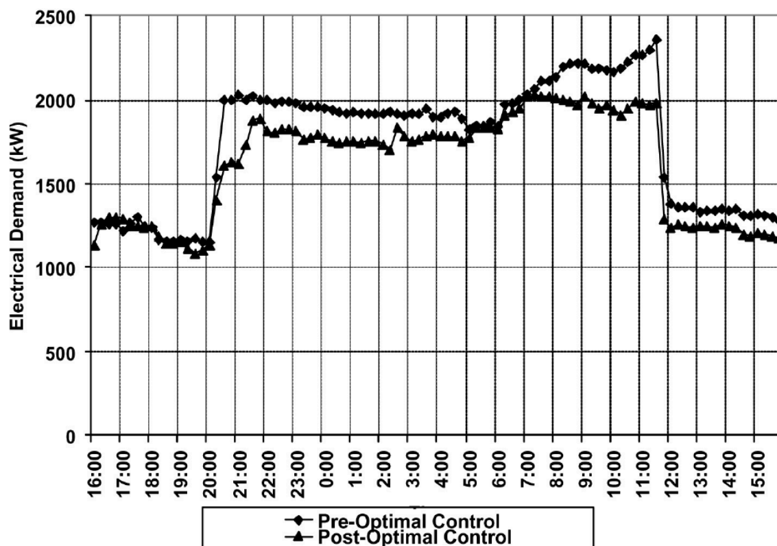
图 10: Figure 8-10. Comparison of Typical Facility Electrical Demand Profile Before and After Implementation of Optimal Control Sequences
