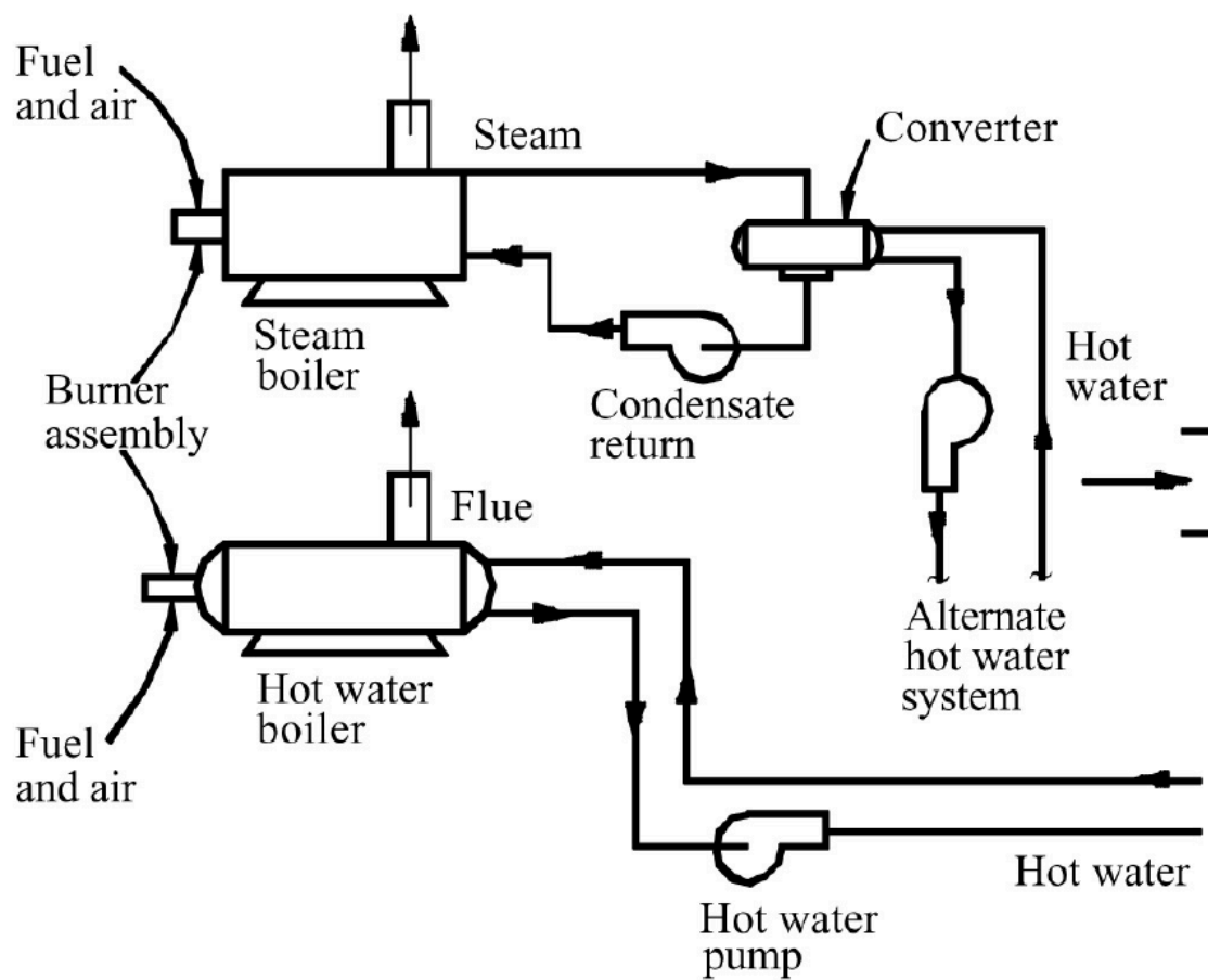
图 1: Figure 7-1. Steam and Hot Water Boilers
