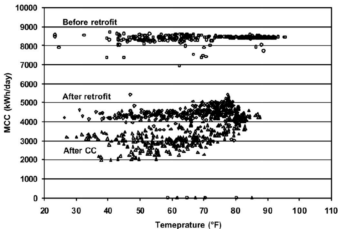
图 5: Figure A-5. ZEC Daily Motor Control Center Electricity Consumption for 1990 Before the Retrofit, 1994 After the Retrofit and 1997 After CCSM
