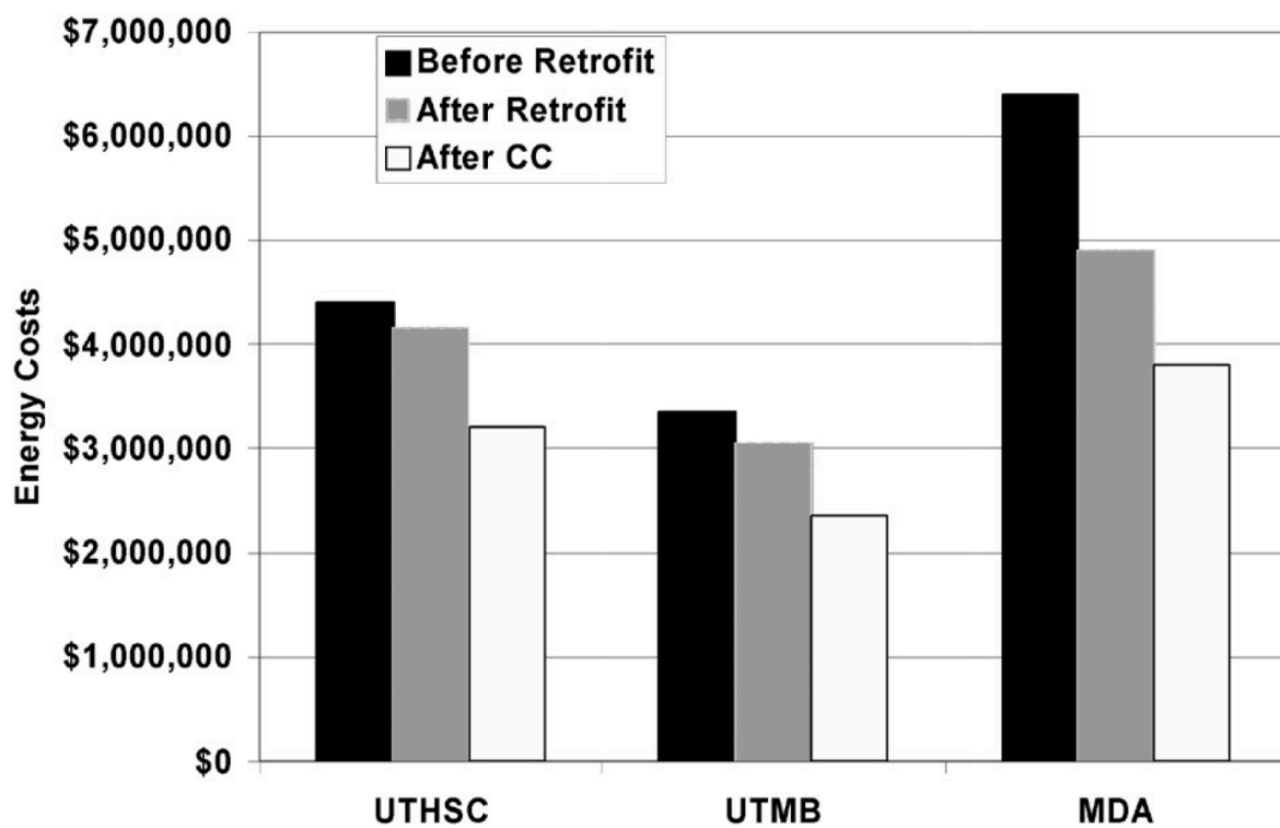
图 1: Figure 2-1. Energy Costs Before Retrofit, After Retrofit, and After Retrofit and CC SM at University of Texas, Health Science Center (UTHSC), University of Texas Medical Branch at Galveston (UTMB), University of Texas, M. D. Anderson Cancer Center (MDA)
