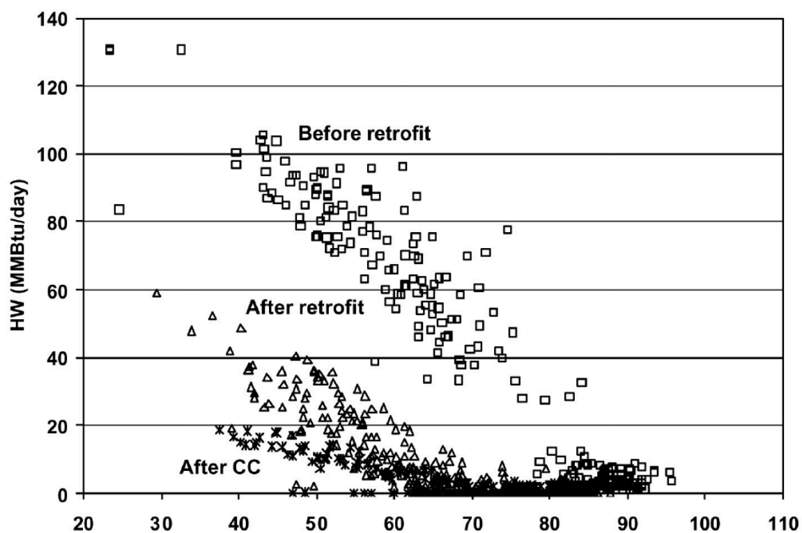
图 7: Figure A-7. ZEC Daily Hot Water Consumption for 1990 Before the Retrofit, 1994 After the Retrofit and 1997 After CCSM
