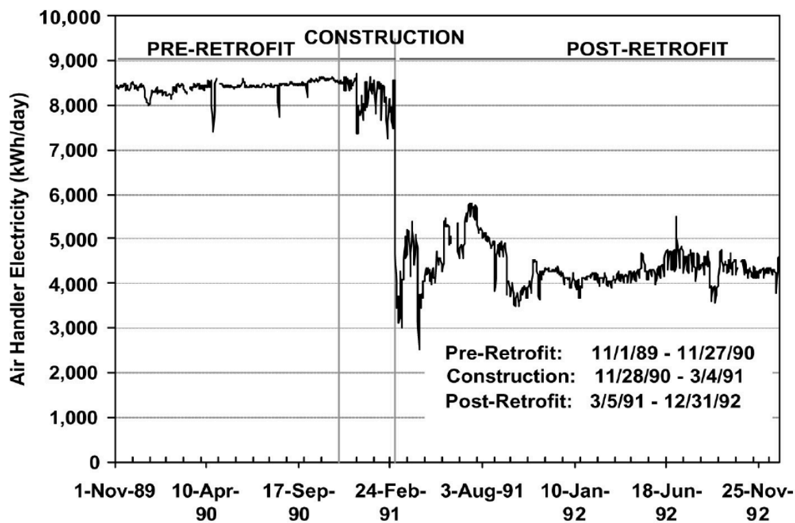
图 1: Figure 9-1. Daily Electricity Consumption for Approximately One Year Before a Retrofit and Two Years After the Retrofit
