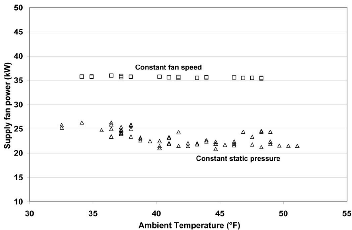
图 20: Figure 4-20. Measured Hourly Supply Air Fan Power for Both the CSFS and VSFS Operations
