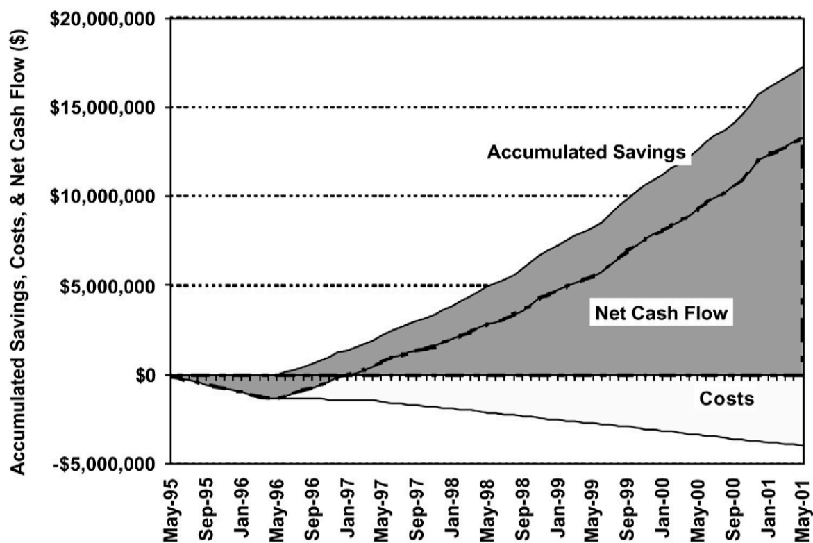
图 2: Figure 2-2. Accumulated Project Cost, Energy Cost Savings and Positive Cash Flow at Texas A&M University, College Station Campus
