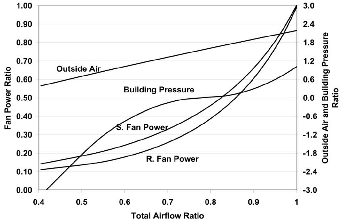
图 22: Figure 4-22. Simulated Building Pressure, Outside Air Intake and Fan Power Using Typical Fan Tracking Control
