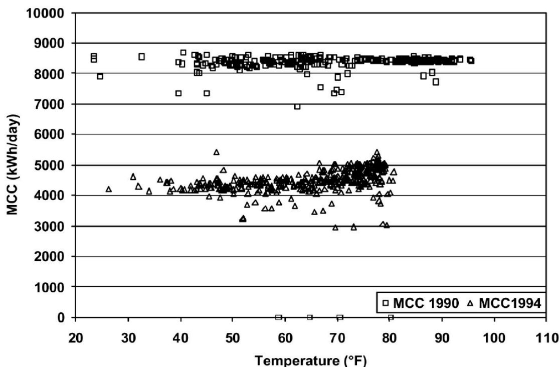
图 2: Figure A-2. ZEC Daily MCC Consumption in 1990 Before the Retrofit, in 1994 After the Retrofit
