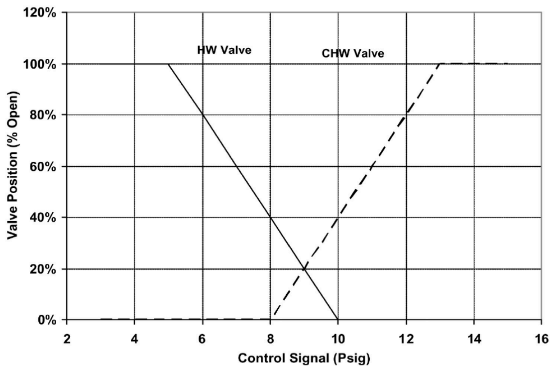
图 12: Figure 4-12. Typical Valve Overlap for a Coupled Control System
