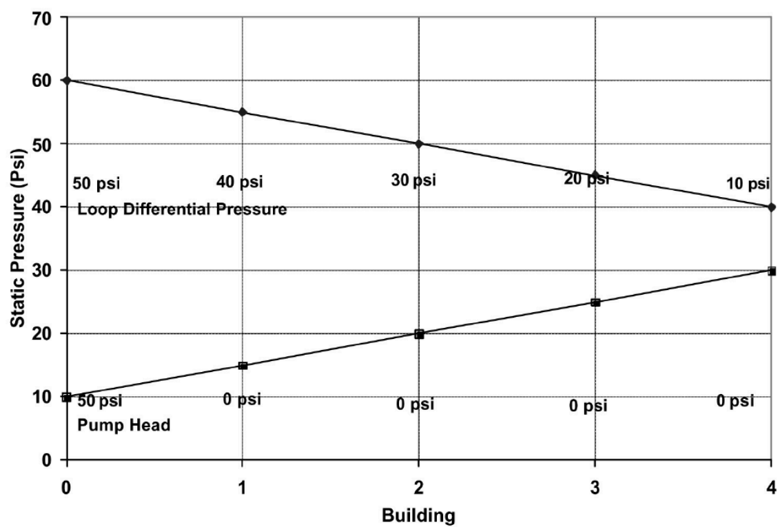
图 5: Figure 5-5. Differential Pressure Distribution for Source Distributed Pumping
