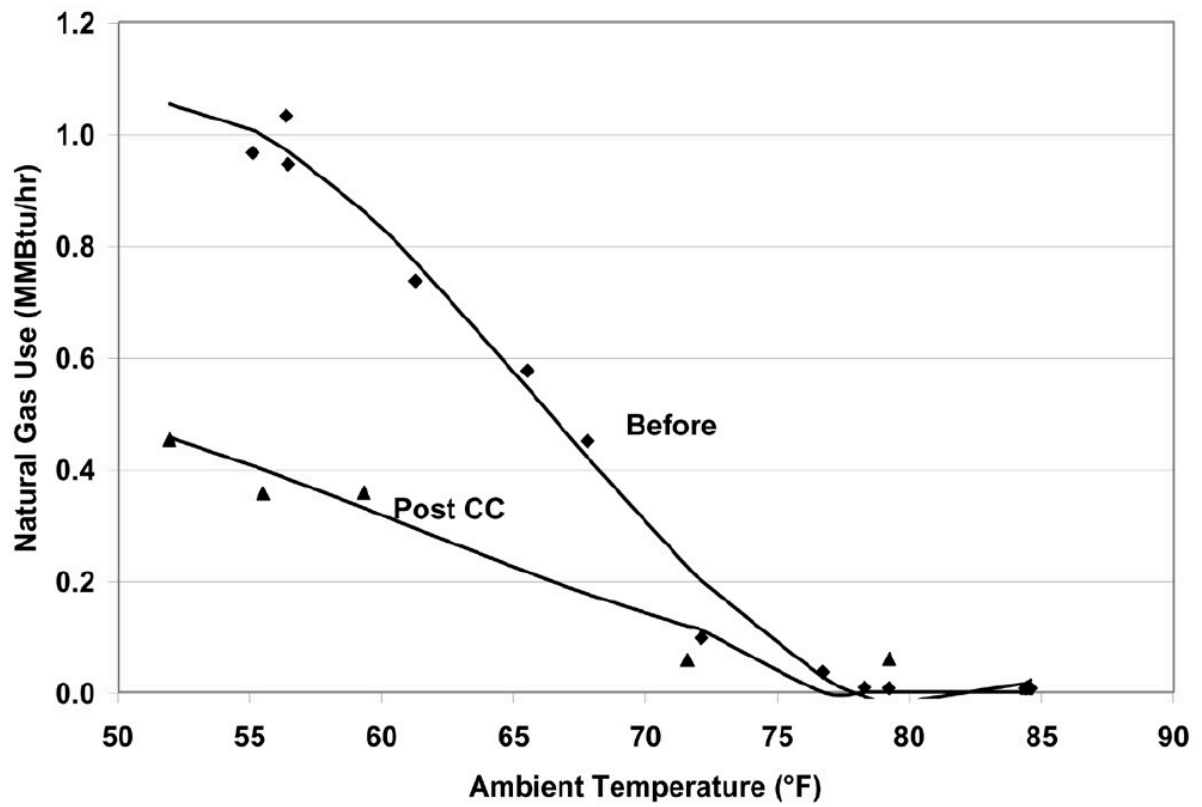
图 5: Figure 4-5. Measured Heating Energy Consumption Versus the Monthly Average Hourly Ambient Temperature
