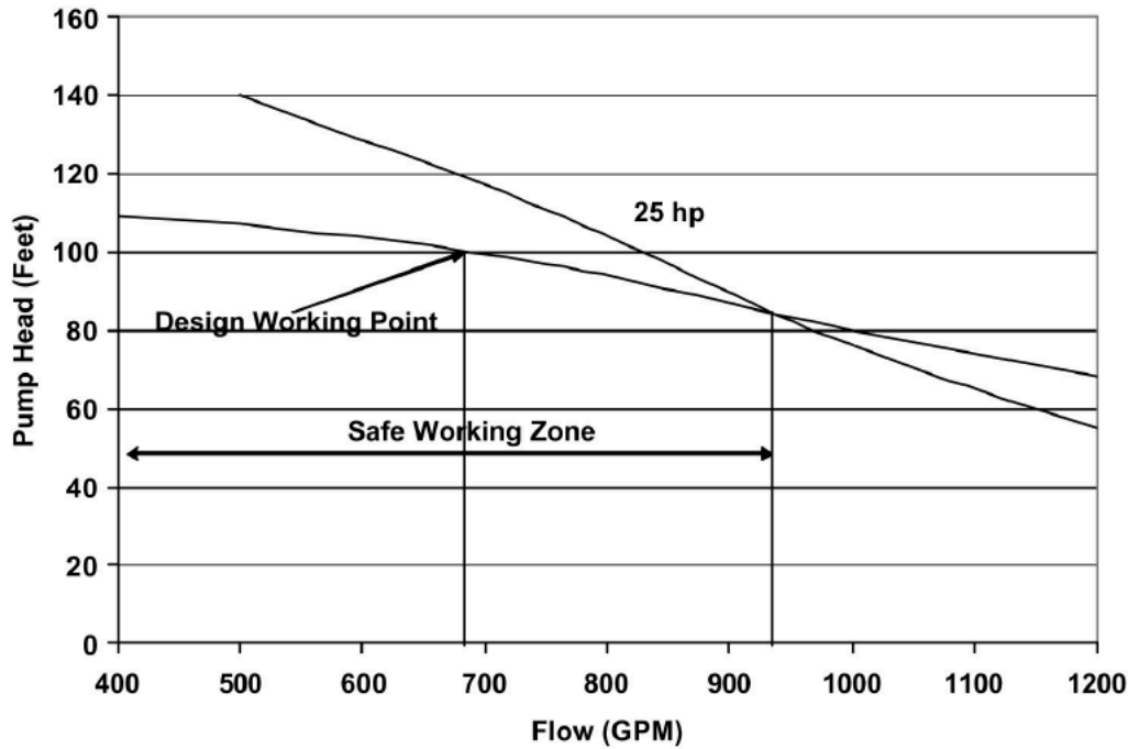
图 10: Figure 5-10. Chilled Water Pump Curve (regenerated using pump curves from TACO, TA Series Model 1229, speed 1760 RPM, and 10.25" impeller)
