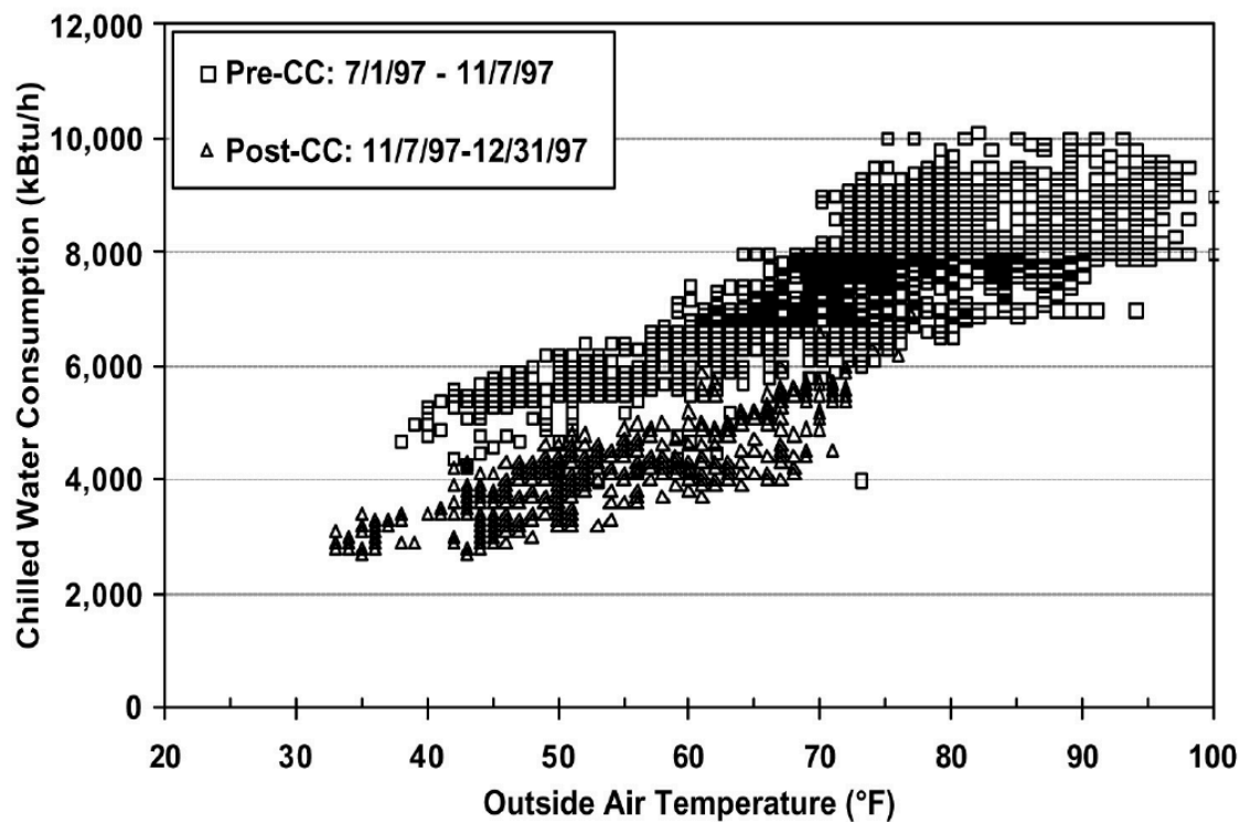
图 13: Figure 4-13. Comparison of Chilled Water Energy Consumption Before and After Implementation of CCSM Measures
