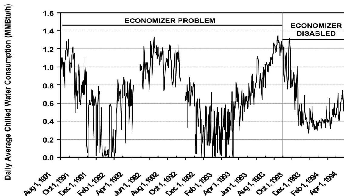
图 10: Figure 4-10. Measured Hourly Cooling Energy Consumption of the Nursing Building in Austin, Texas
