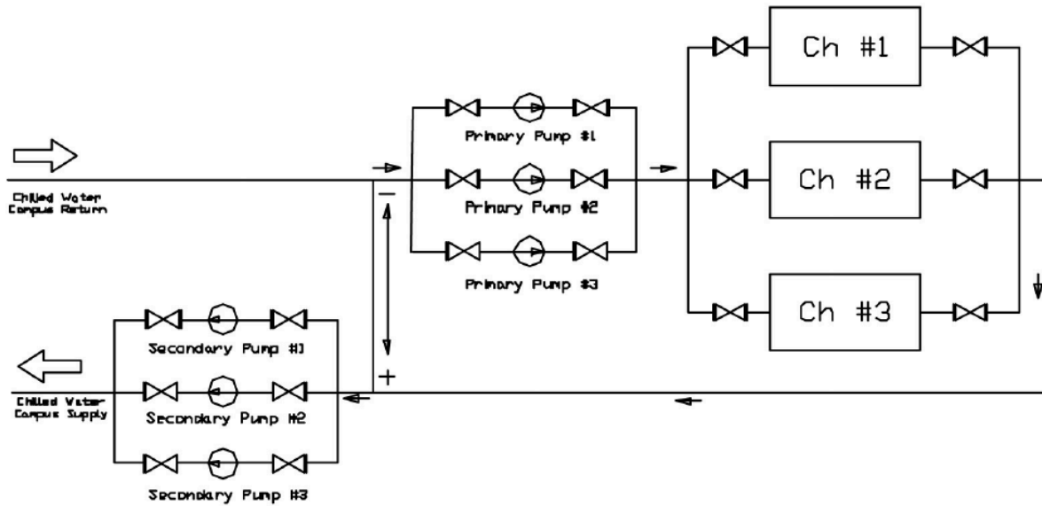
图 11: Figure 5-11. Primary and Secondary Loop Configurations for the South Satellite Plant on the Texas A&M Campus
