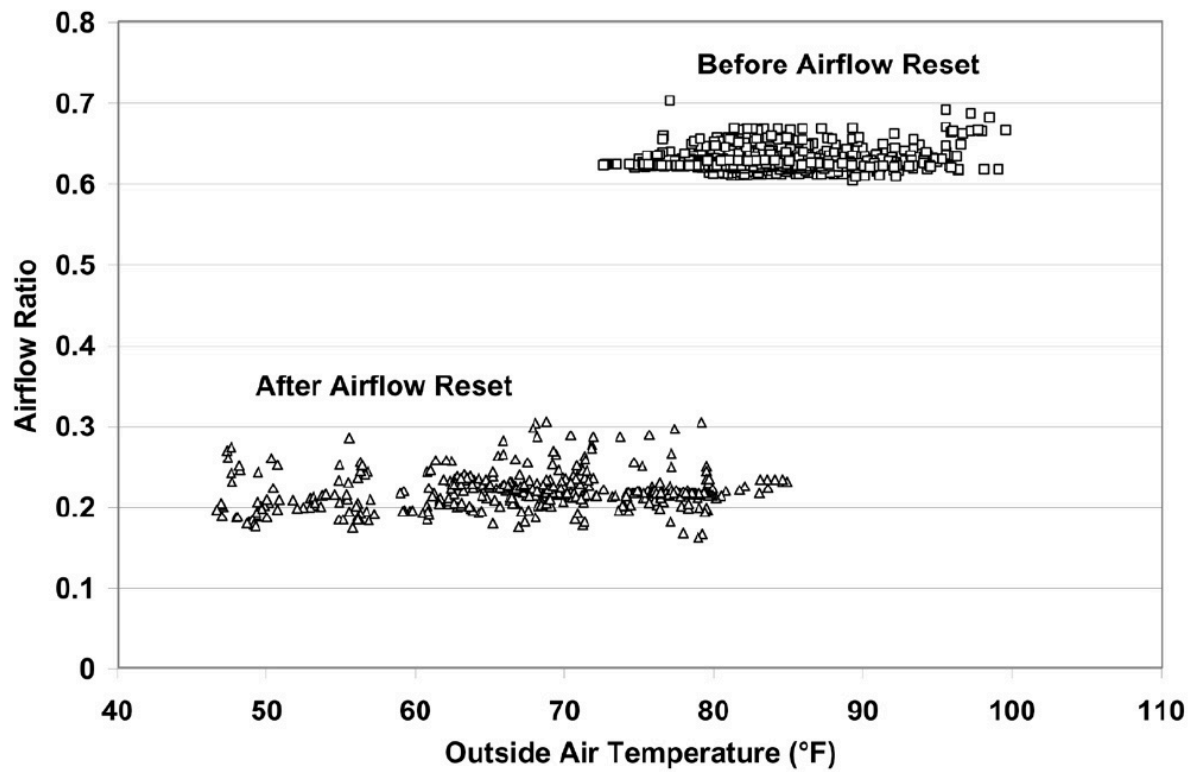
图 25: Figure 4-25. Comparison of Air Flow Before and After Airflow Reset During Unoccupied Hours (Airflow Ratio is defined as the ratio of the air flow to the design air flow)
