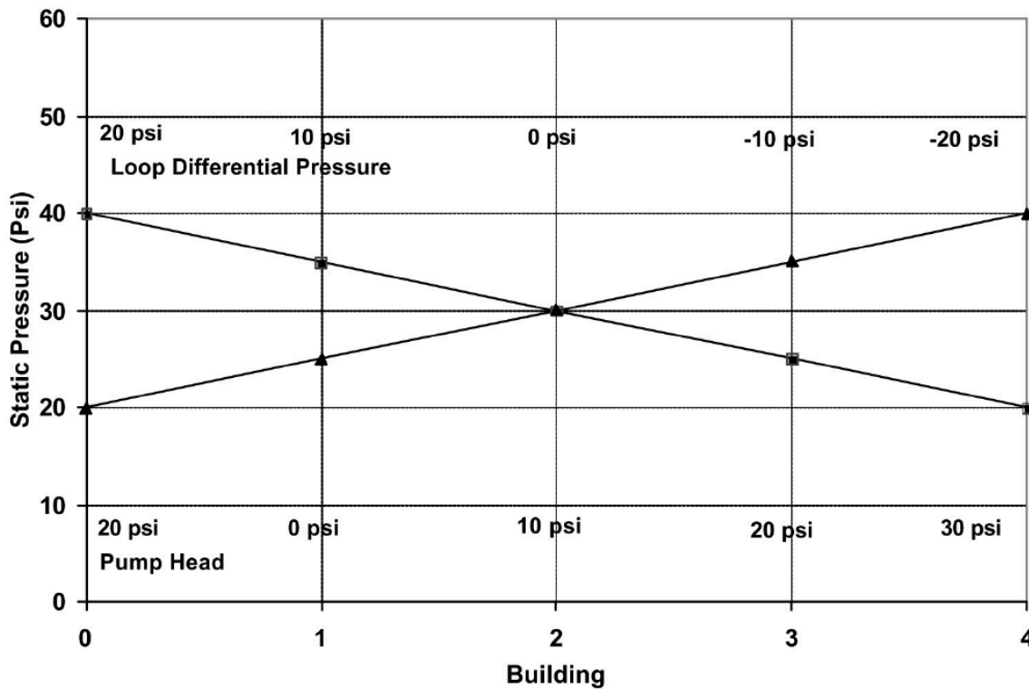
图 6: Figure 5-6. Differential Pressure Distribution for the Evaluation of Combined Source and Distributed Pumping
