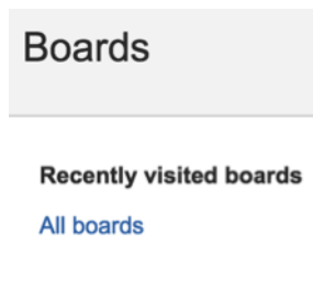
Fig. 28.2: Jira boards
