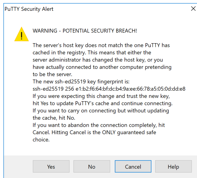
Fig. 198: PuTTY security alert when connecting to a new server
