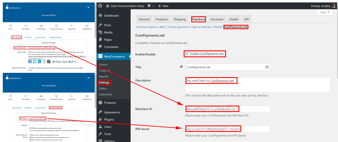
Fig. 177: Configuring the CoinPayments.net WooCommerce plugin
