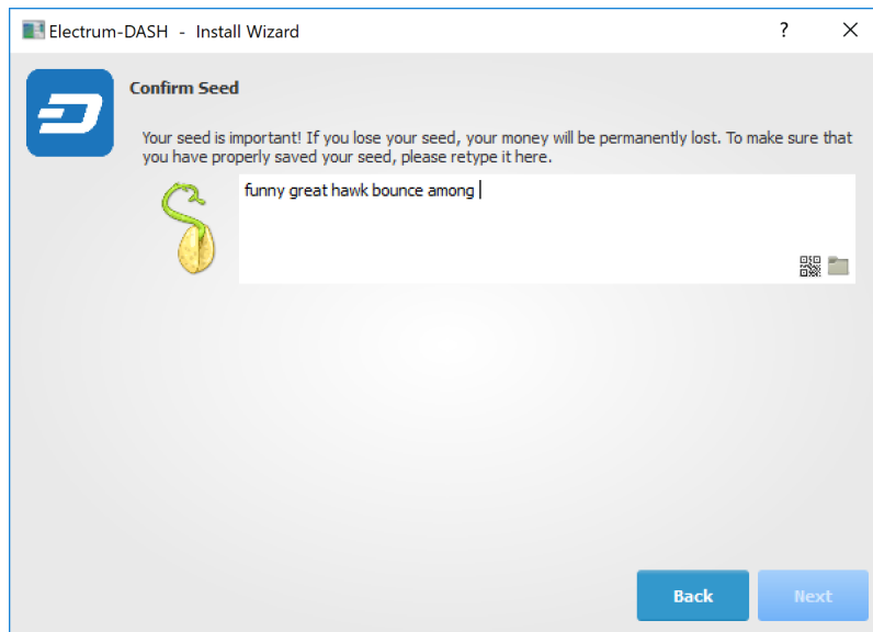
Fig. 104: Generating and confirming the recovery seed
