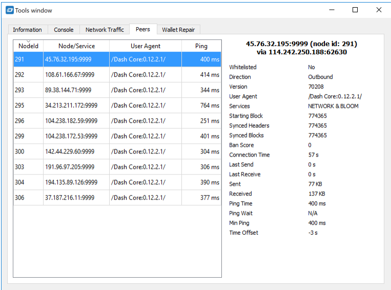
Fig. 73: The Peers tab of the Axe Core Tools dialog
