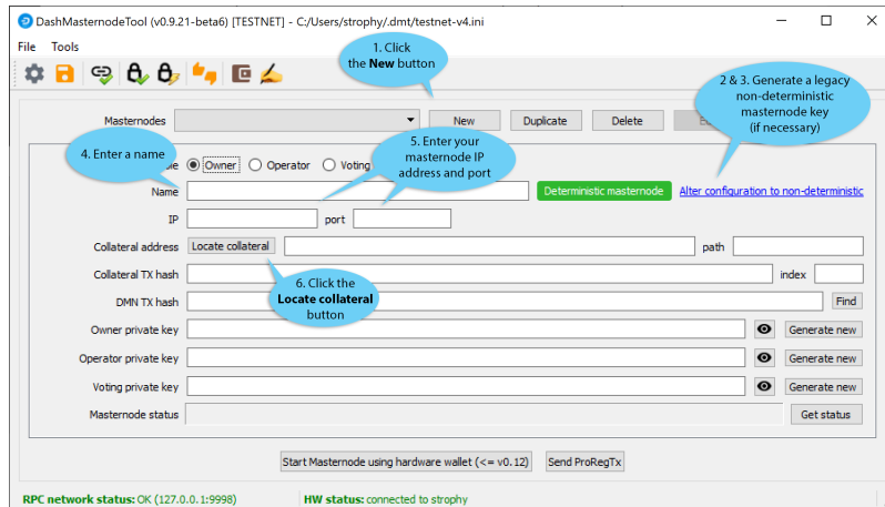
Fig. 204: Axe Masternode Tool configuration steps
