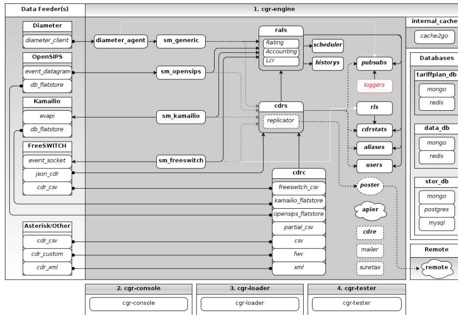
Fig. 1.1: CGRateS high level design
