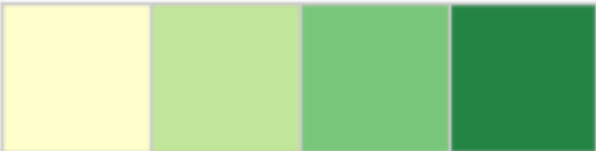
YIGn - 4
