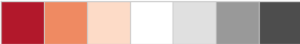
RdGy - 7
