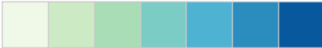
GnBu - 7
