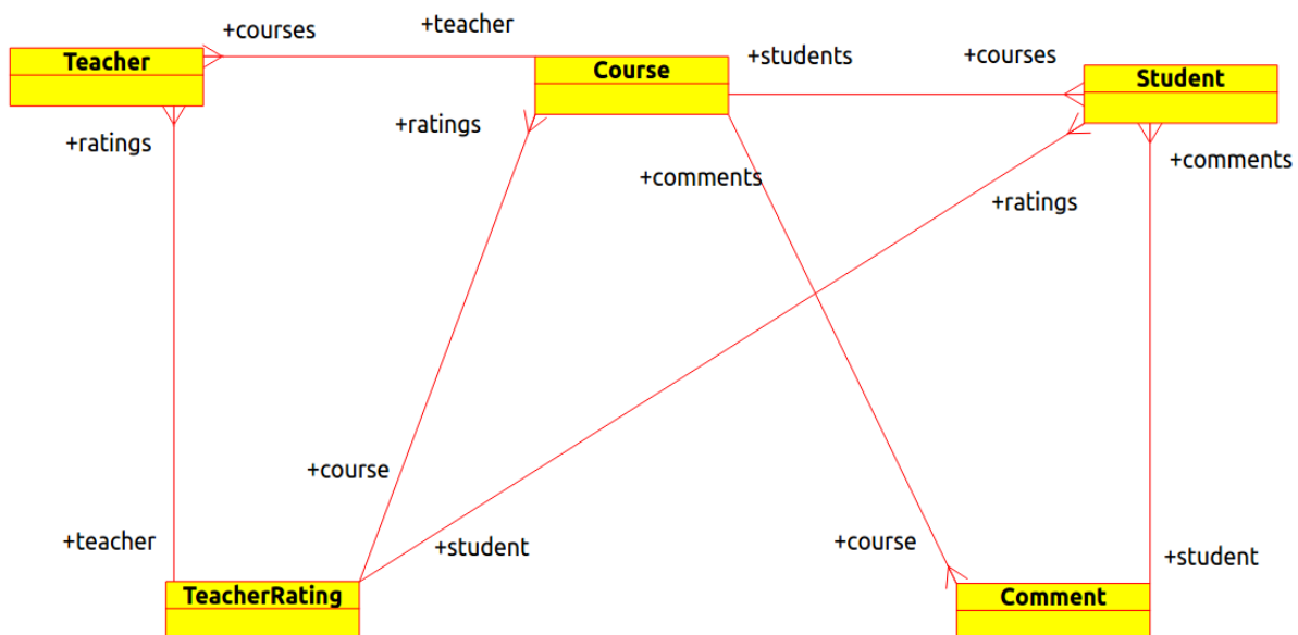
Figure 1.1: Entity diagram
