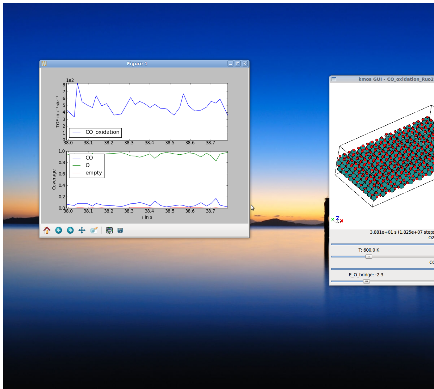
Fig. 1.5: The compiled module can be run and watched in realtime. When parameters are changed this is immediately reflected in the rate constants.
