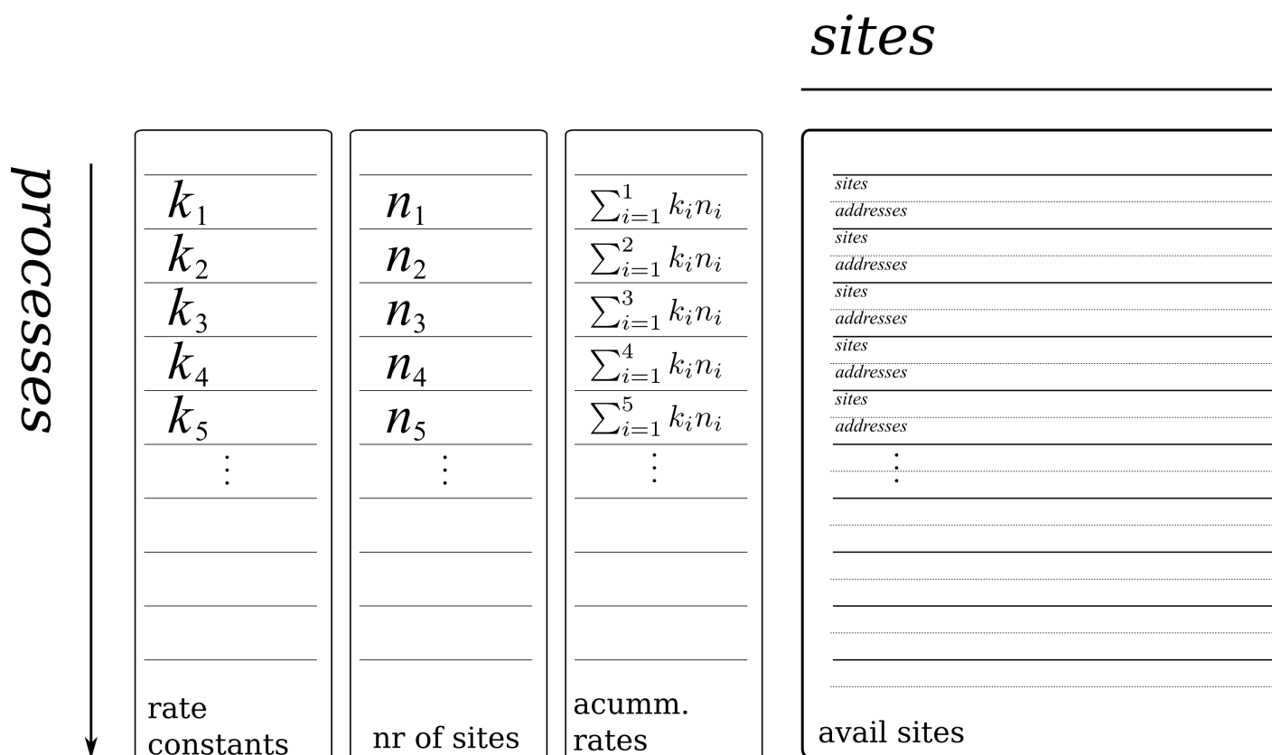
Fig. 2.2: The data model underlying the kmos solver. The central component is the avail_sites array which stores for each elementary step the sites for which it is executable. Secondly it stores the location in memory, where the availability of the site is stored for direct access. The array of rate constants holds the numeric rate constant and only changes, when a physical parameter is changed. The nr of sites array holds the total number of sites for each process and needs to be updated whenever a process becomes available und unavailable. The accum. rates has to be updated once per kMC step and holds the accumulated rate constant for each processes. That is, the last field of accum. rates holds k_{\text{tot}} , the total rate of the system.
