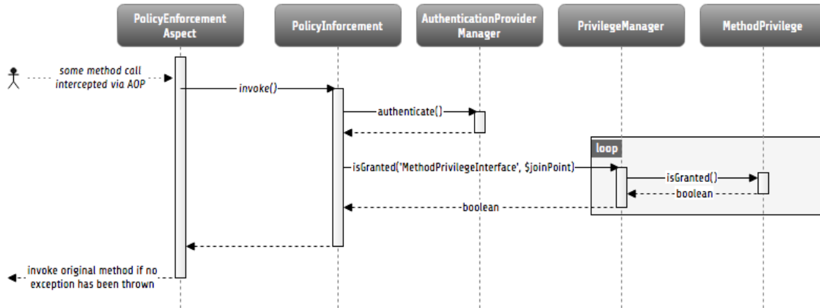
Fig. 29: How an authorization decision is formed and enforced in Flow
