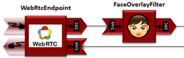
Fig. 18: WebRTC with filter in loopback Media Pipeline
