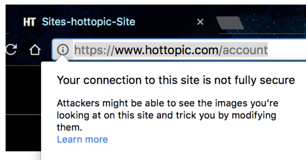
Fig. 19.3: This screenshot is of the login page on Hot Topic’s website. Even though it says https, this is an indication that not all data on the webpage is encrypted and some of the content is readable. However, the information that is being inputted into the email and password is secure. The screenshot below explains what is not encrypted on the webpage.
