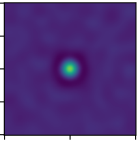
RickerWavelet2DKernel
